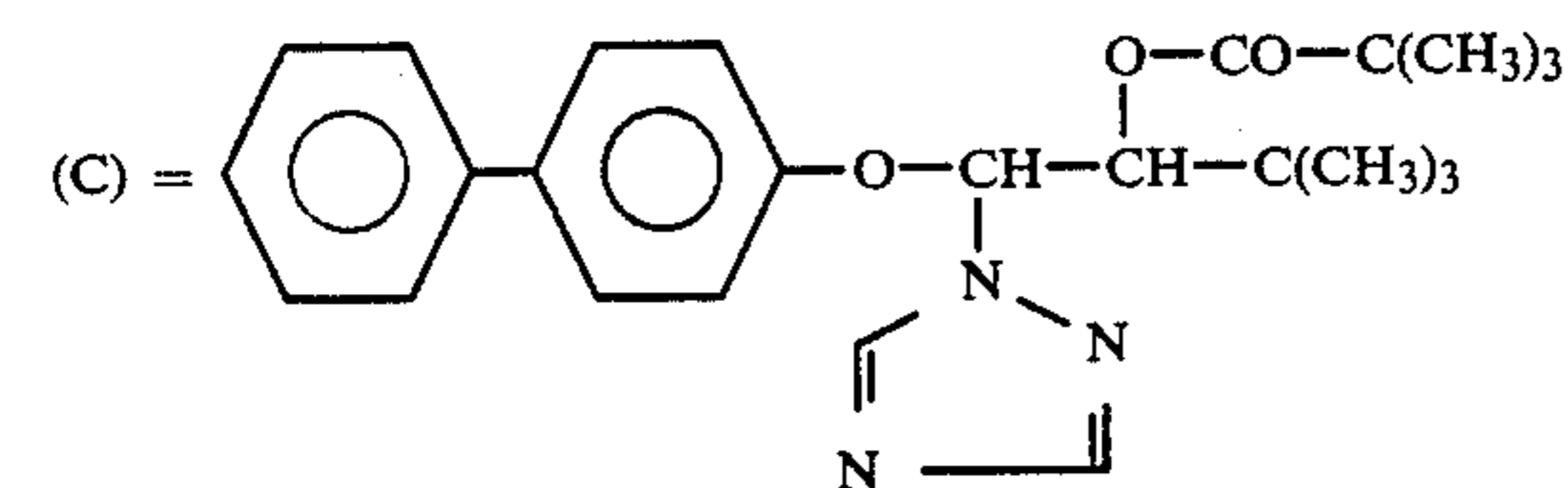
2-Chloroethyl-trimethyl-ammonium chloride
