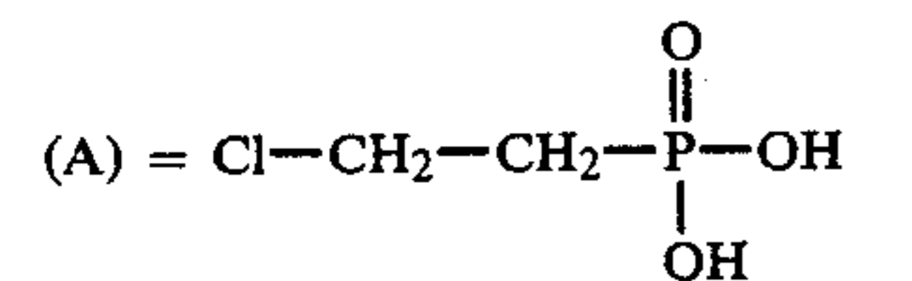
2-Chloroethylphosphonic acid
