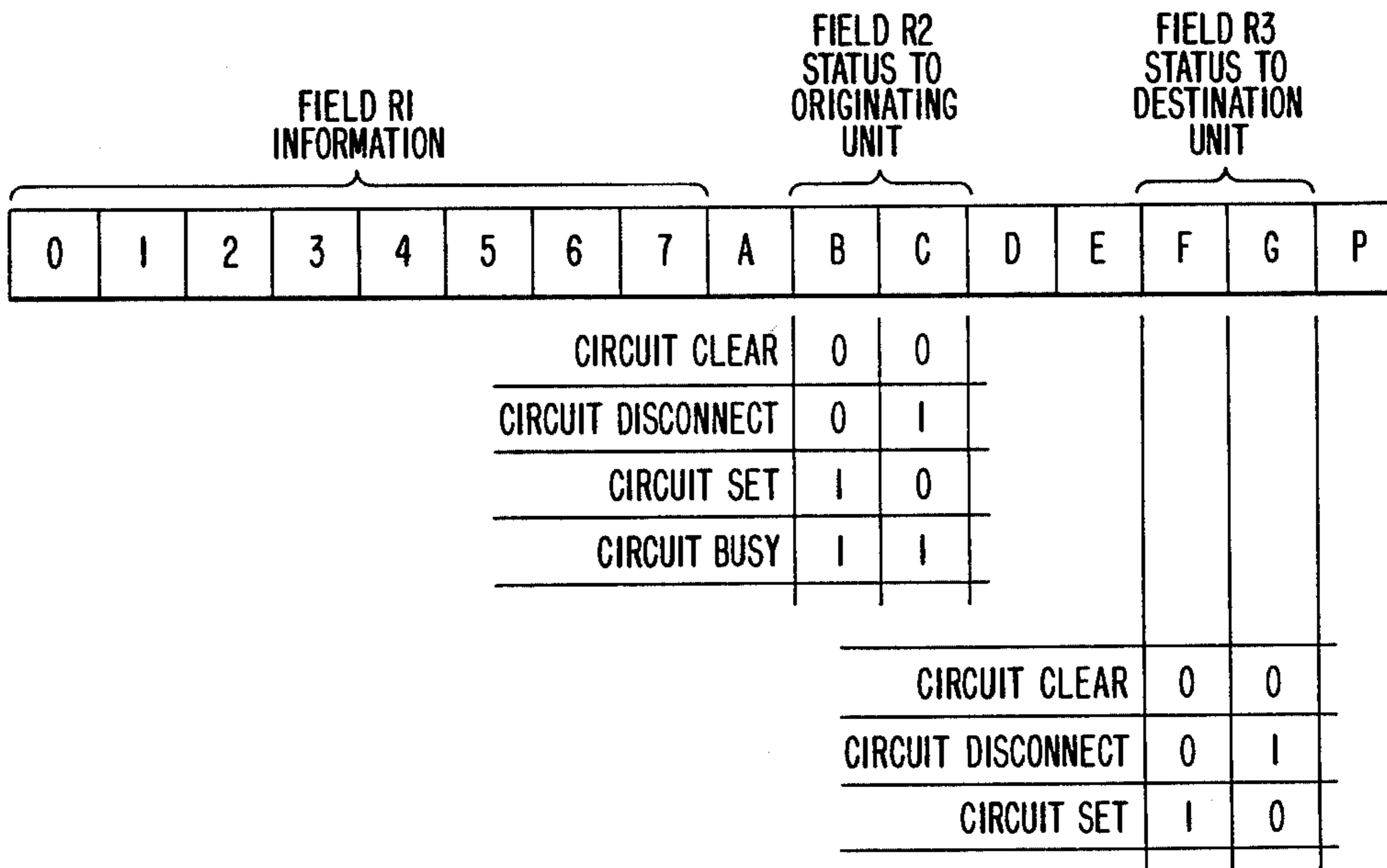
FIG. 12 CONTROL WORD FORMAT ON OUTGOING TIME-MULTIPLEXED LINE 302
