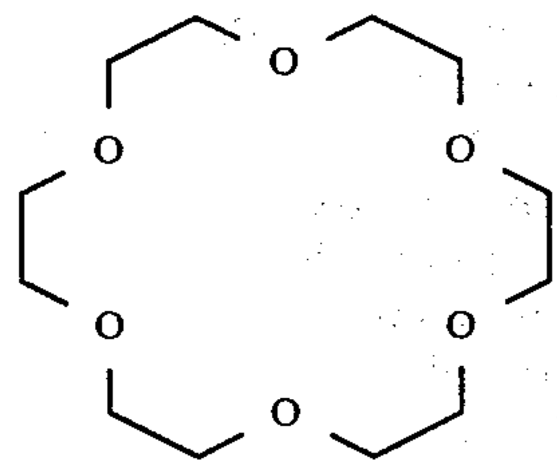
18-crown-6:
