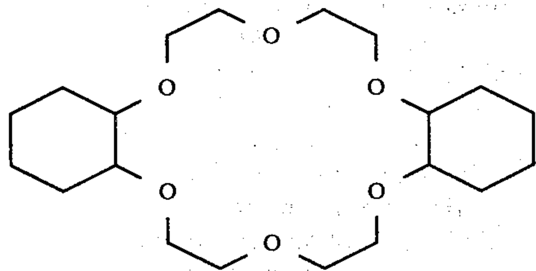
dicyclohexyl-18-crown-6:
