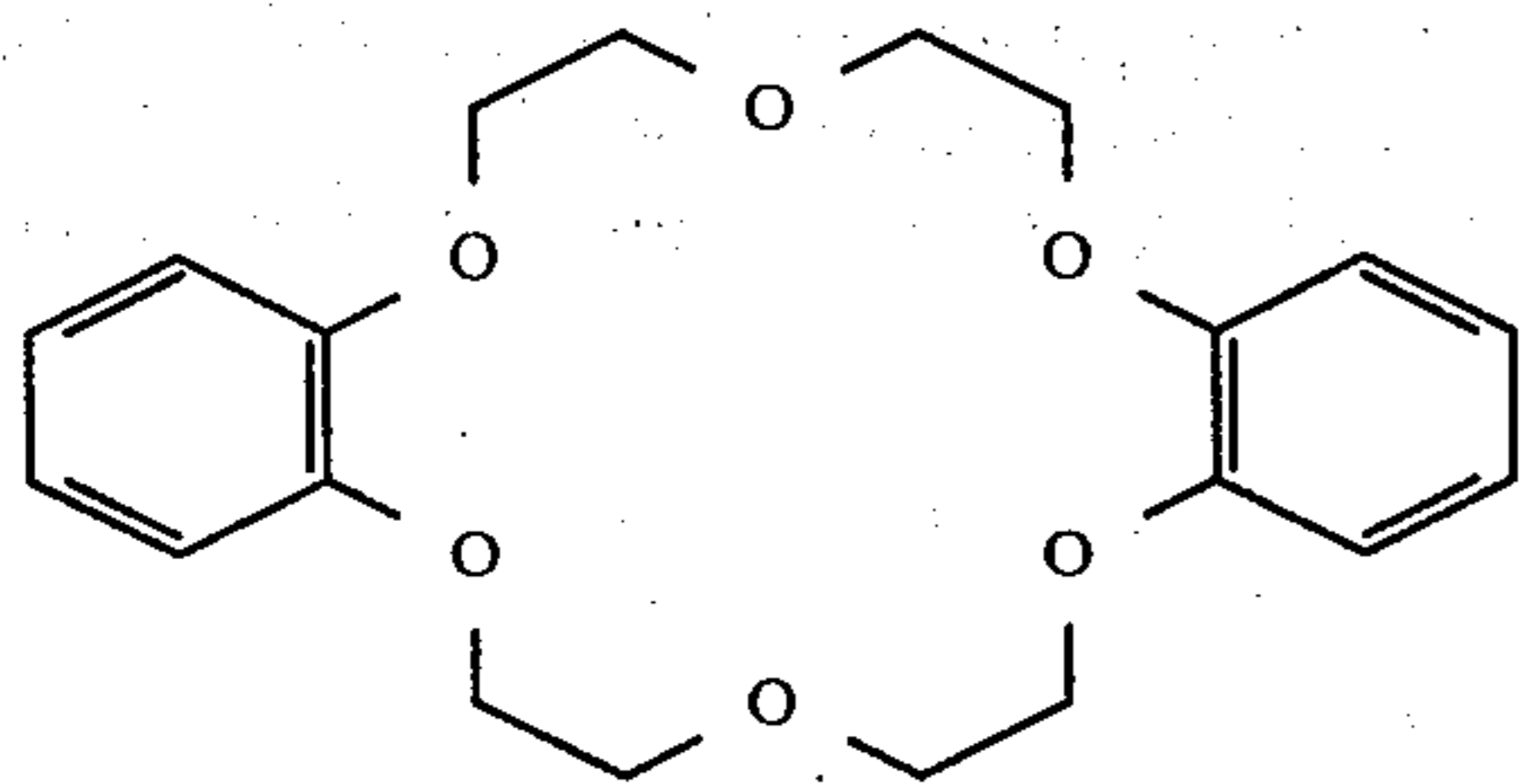
dicyclohexyl-18-crown-6:
