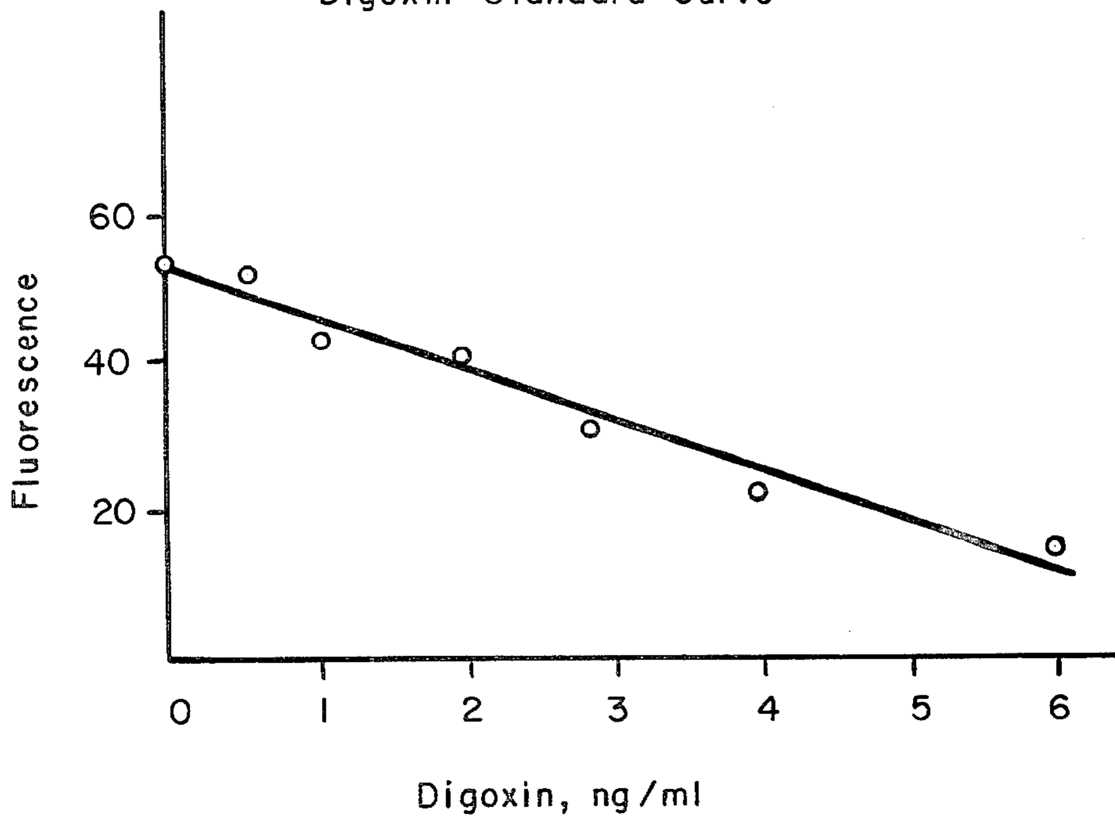
Digoxin Standard Curve
