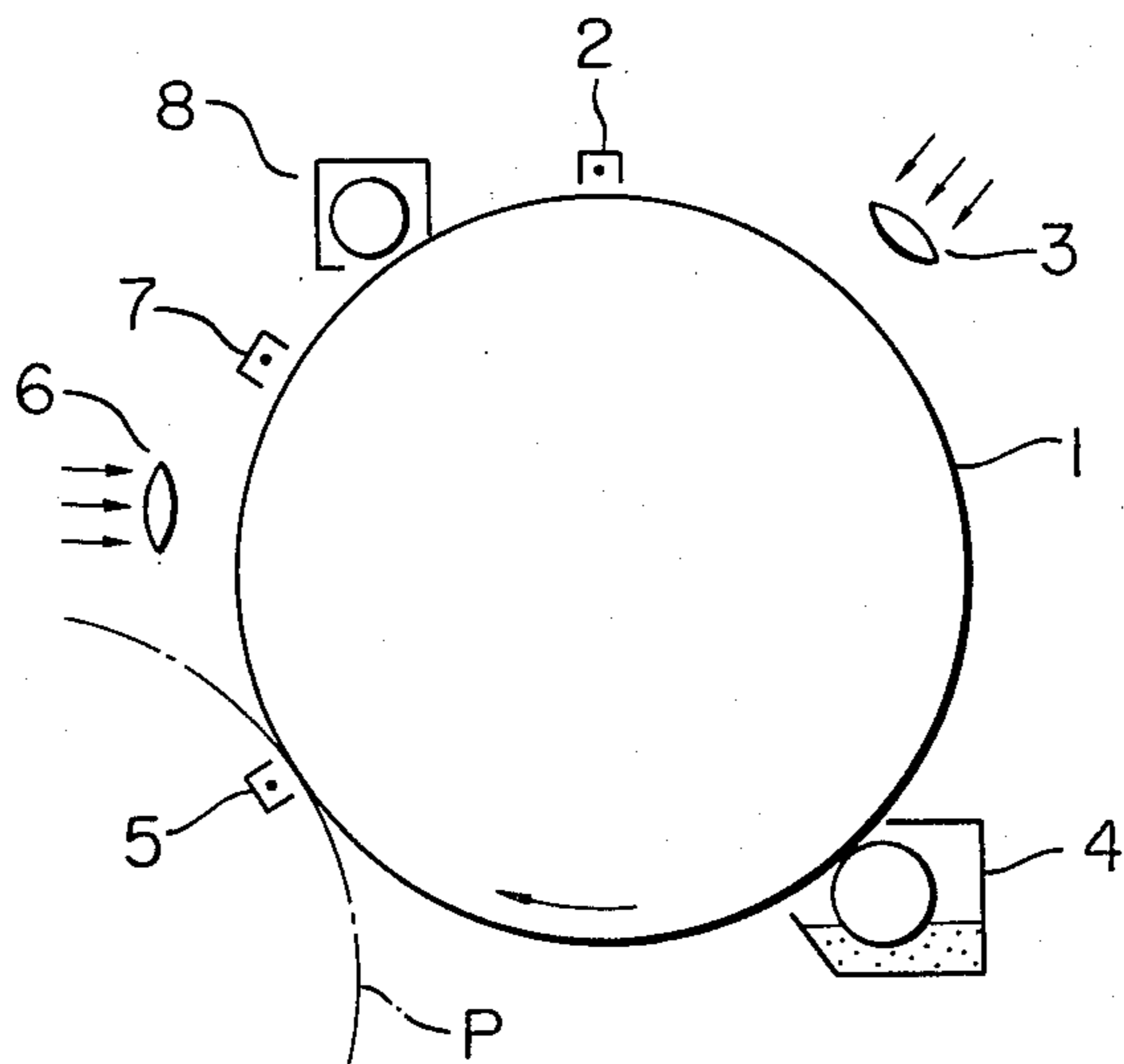
FIG. 1 (PRIOR ART)
