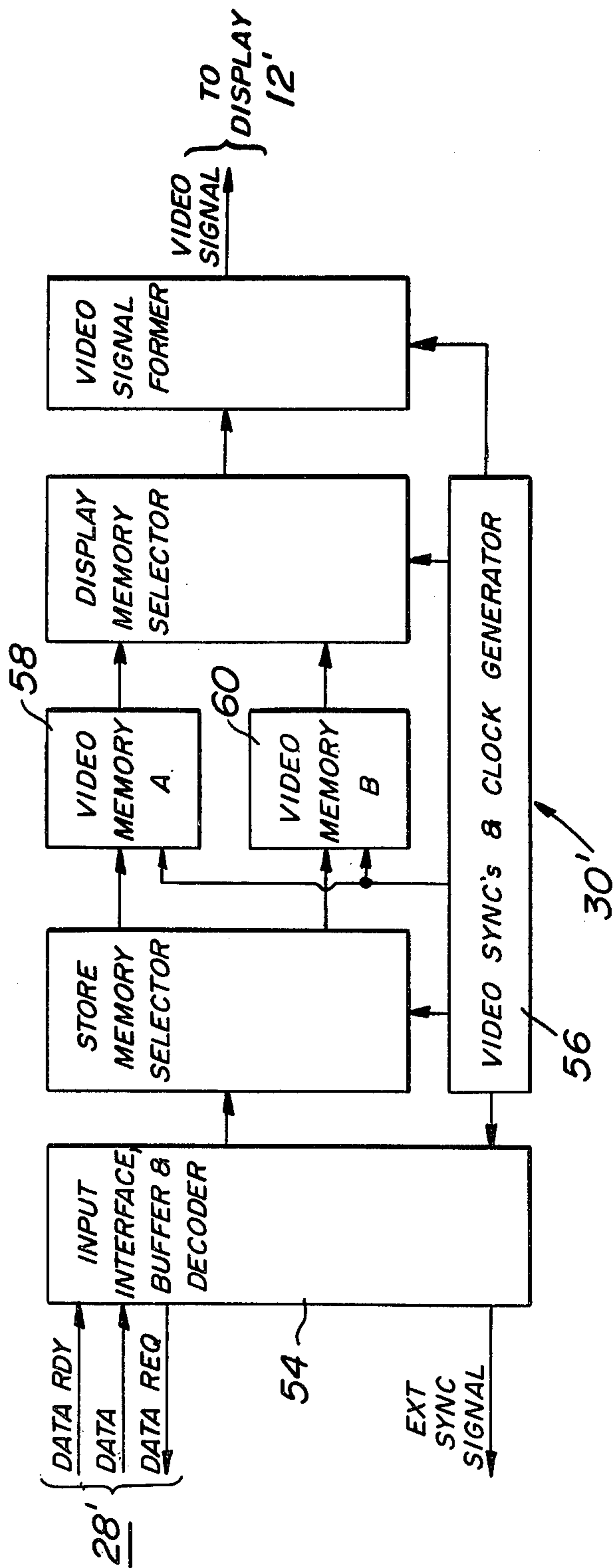
VIDEO DISPLAY PROCESSOR BLOCK DIAGRAM
