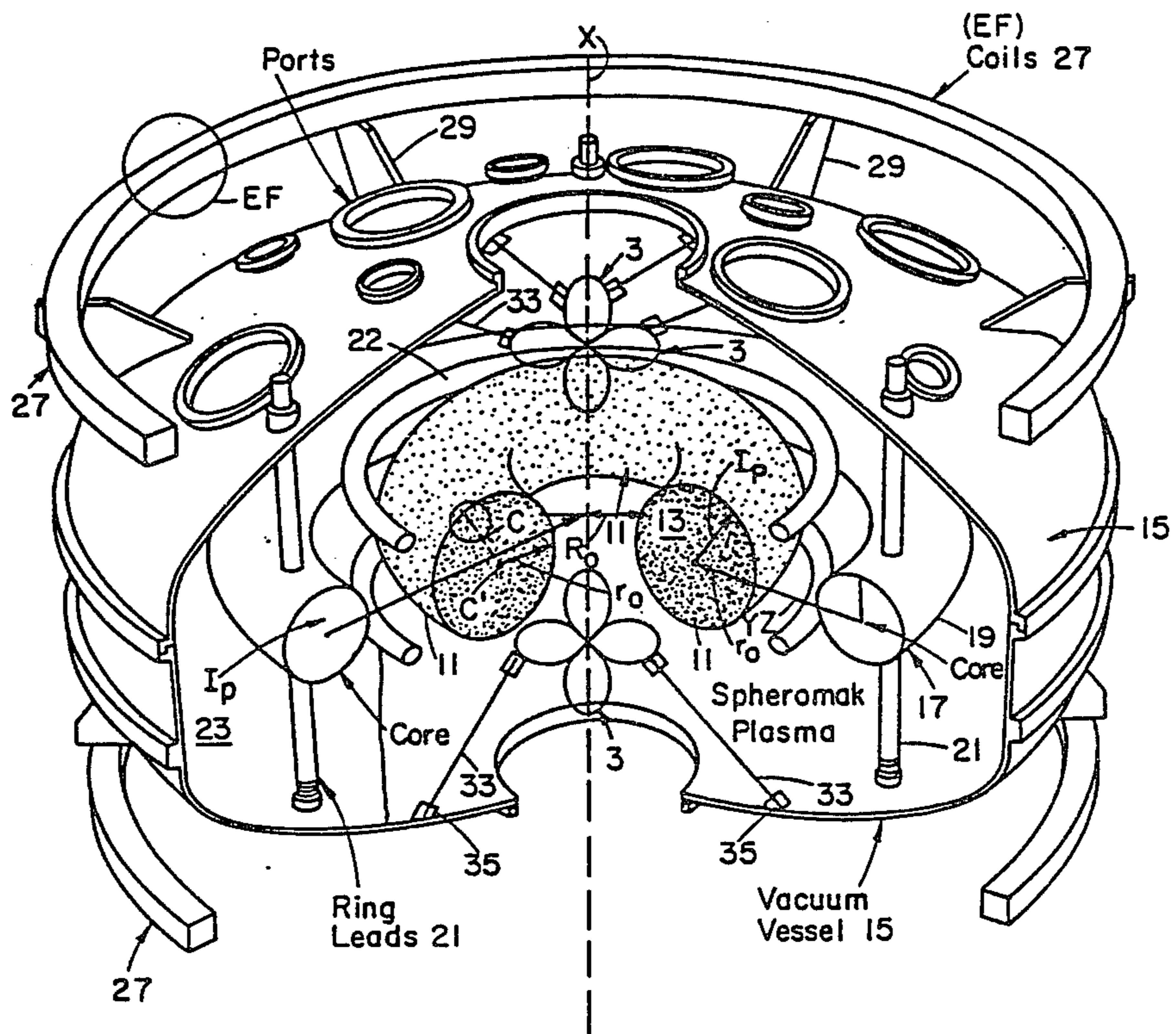
THE SPHEROMAK DEVICE
