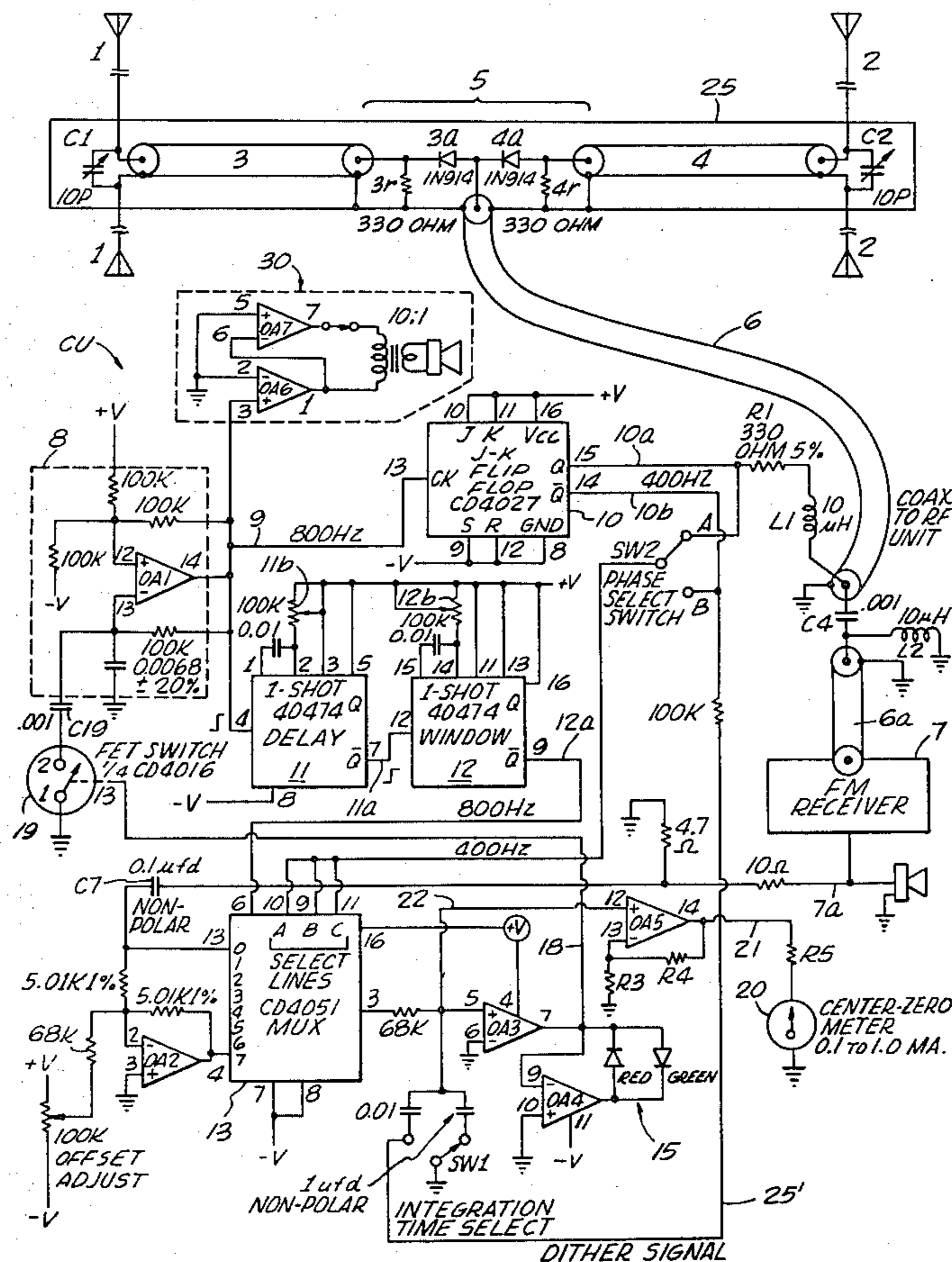
ALL OP AMPS ARE ELEMENTS OF LM324 QUAD PACKAGES
