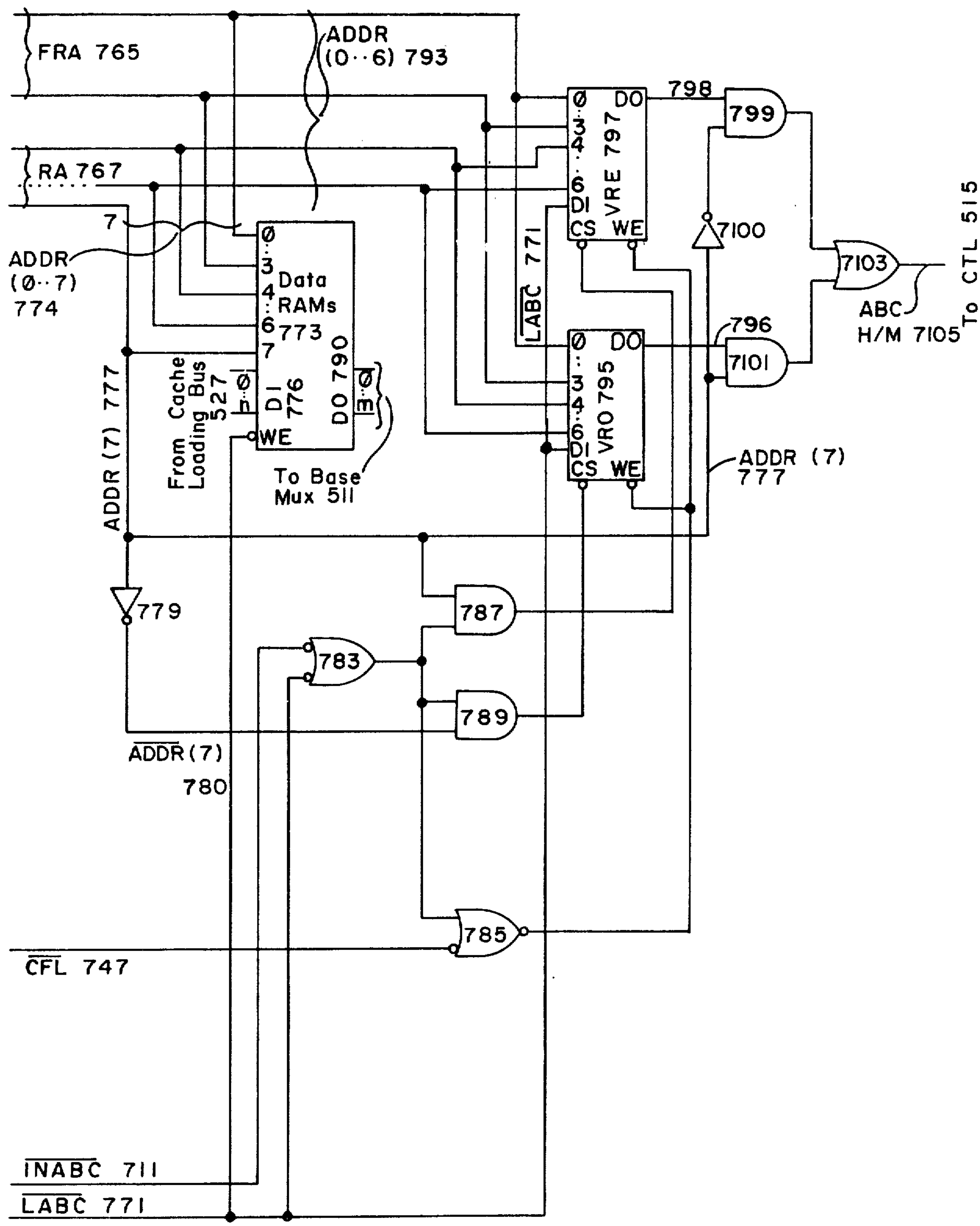
Fig. 7A Preferred Embodiment 772 of ABC Registers 504
