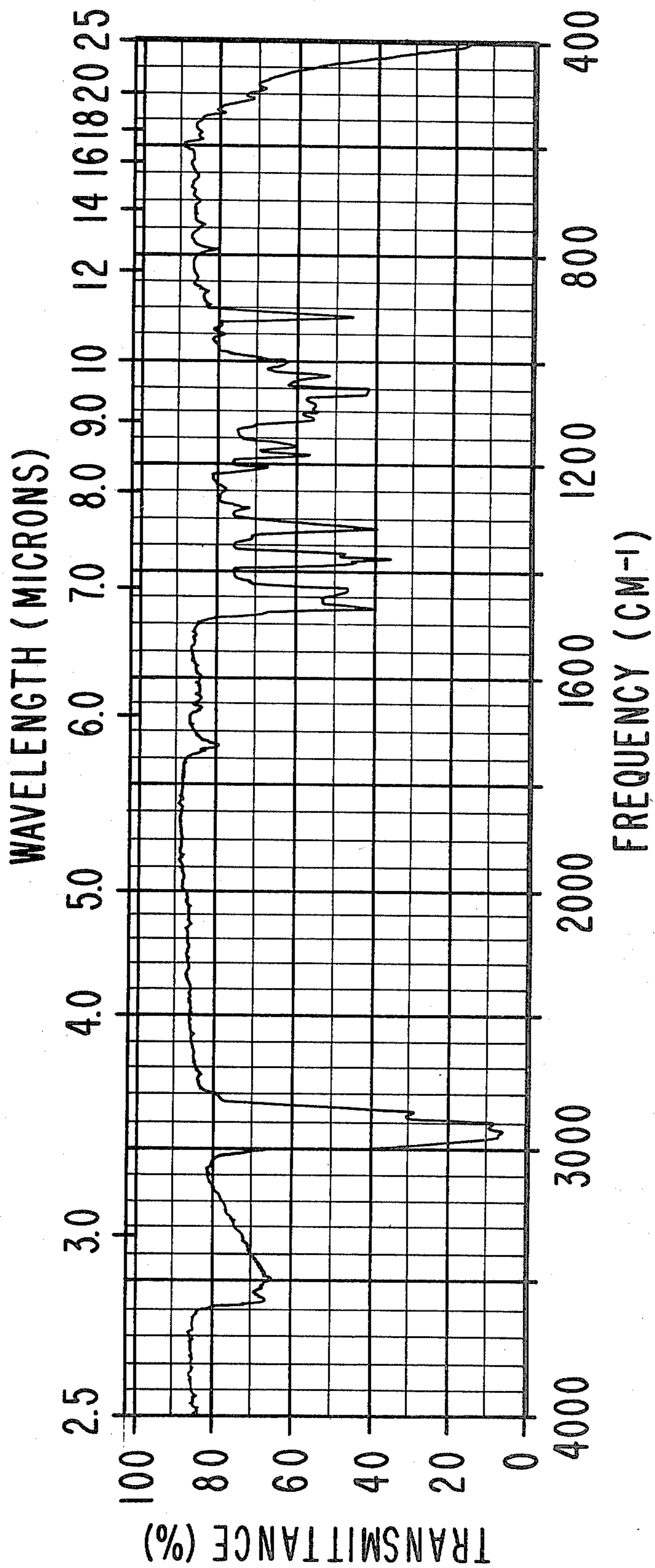
IR SPECTRUM FOR PEAK 901 OF FIG. 9 FOR EXAMPLE III.
