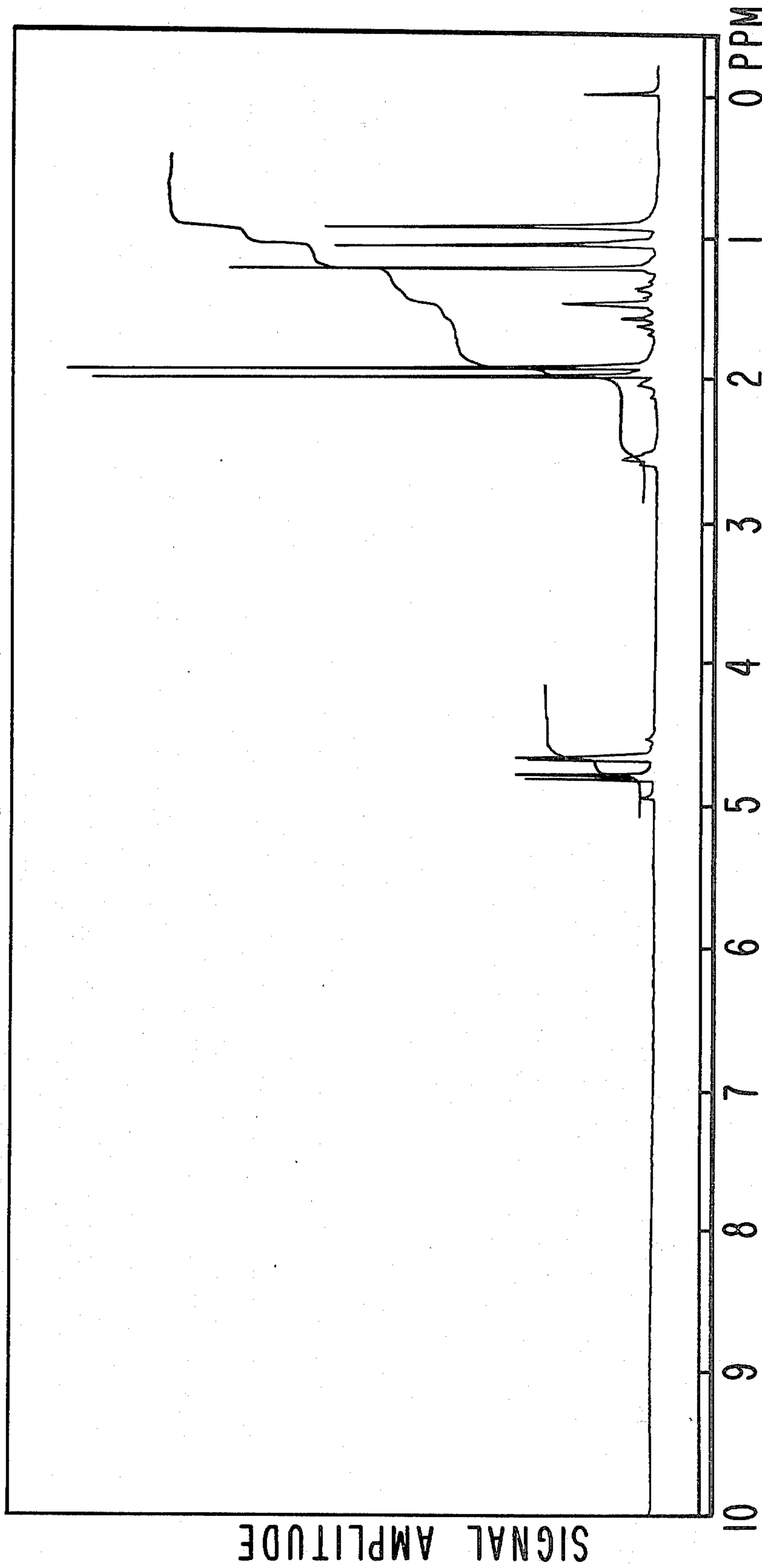
NMR SPECTRUM FOR PEAK 201 OF FIG. 20, EXAMPLE V.
