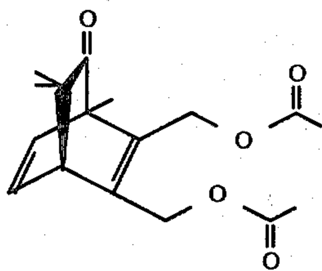
FIG. 17 is the mass spectrum for the peak indicated by reference numeral "162" of FIG. 16 for the compound produced according to Example IV having the structure:
