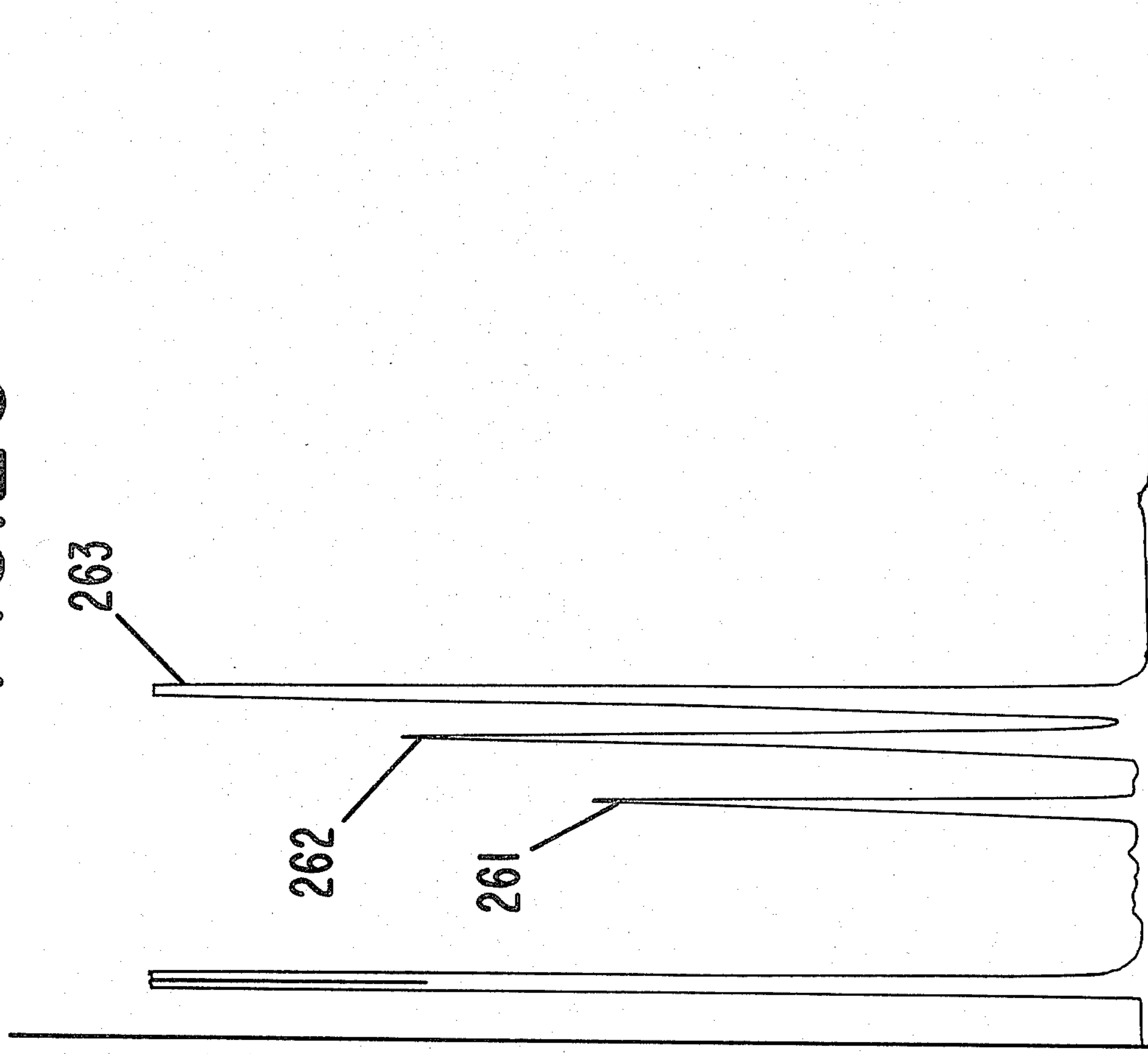
GLC PROFILE FOR EXAMPLE XX (A)
