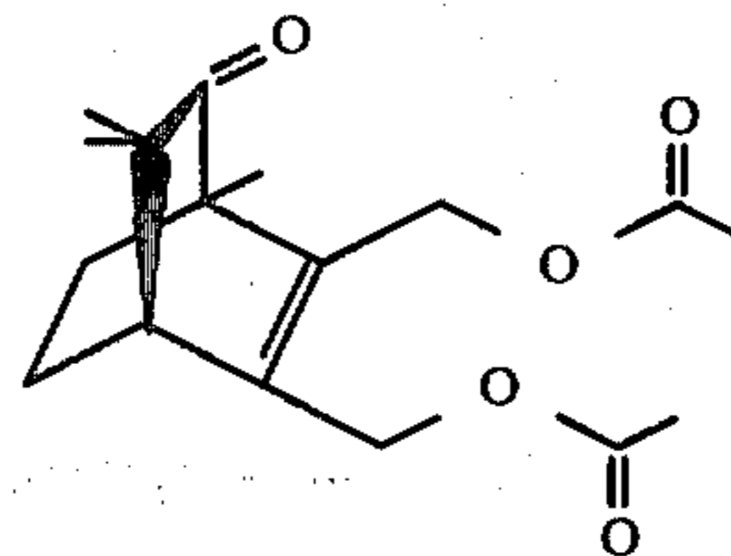
FIG. 24 is the GLC profile for the reaction product of Example VI containing the compound defined according to the structure:
