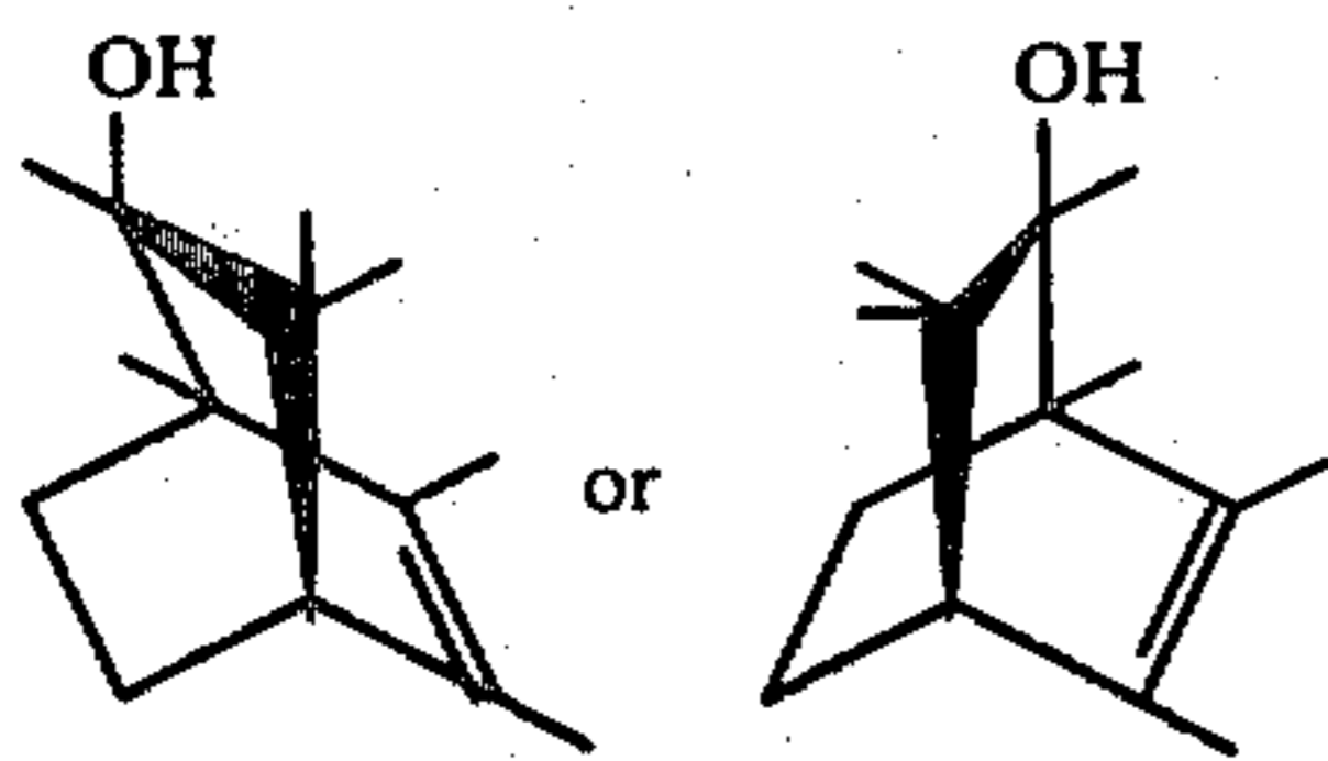
FIG. 16 is the GLC profile for the reaction product of Example IV containing the compound having the structure:
