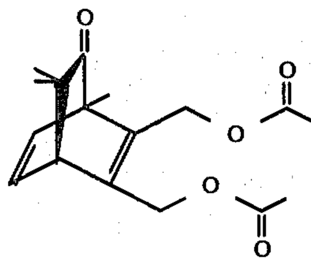
FIG. 18 is the infra-red spectrum for the peak indicated by reference numeral "162" of FIG. 16 for the compound produced according to Example IV having the structure:
