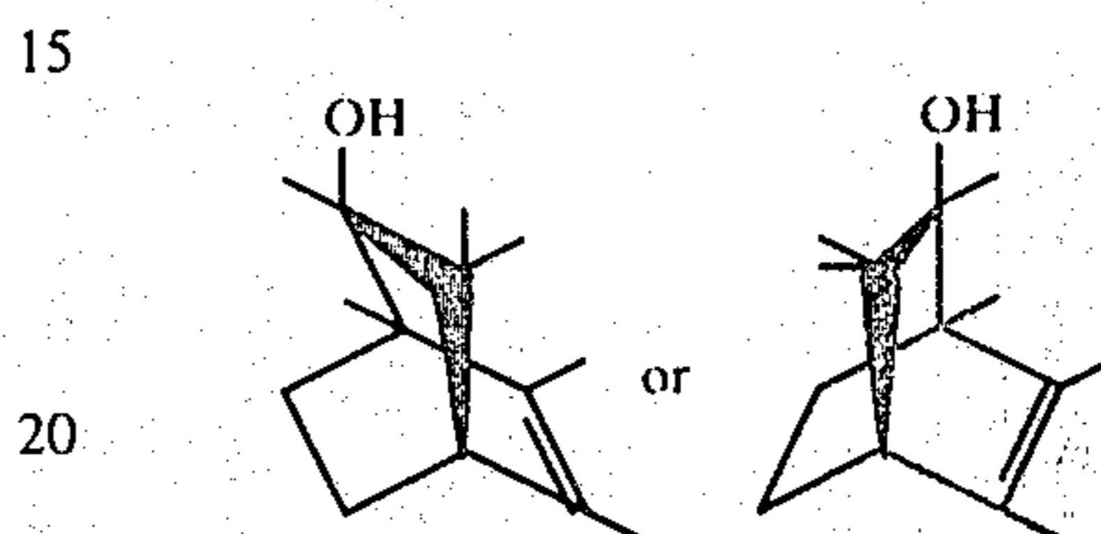
FIG. 11 is the infra-red spectrum for the compound of peak 901 of FIG. 9 having one of the structures:
