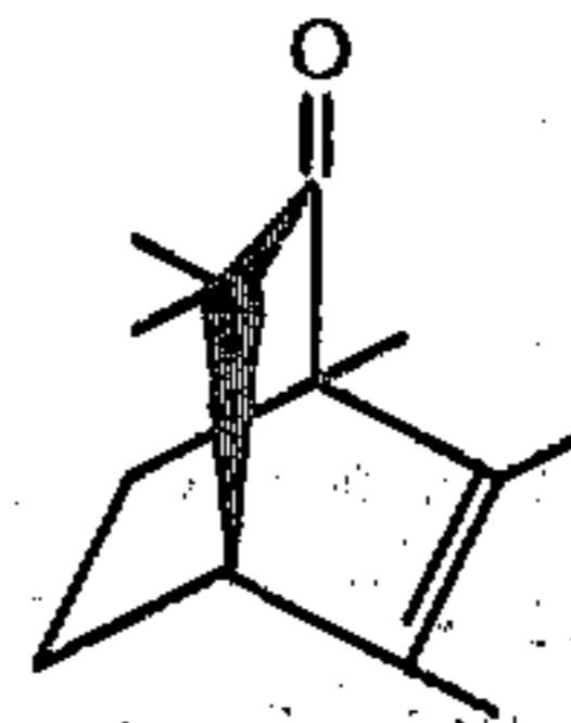
FIG. 24 is the GLC profile for the reaction product of Example VI containing the compound defined according to the structure:
