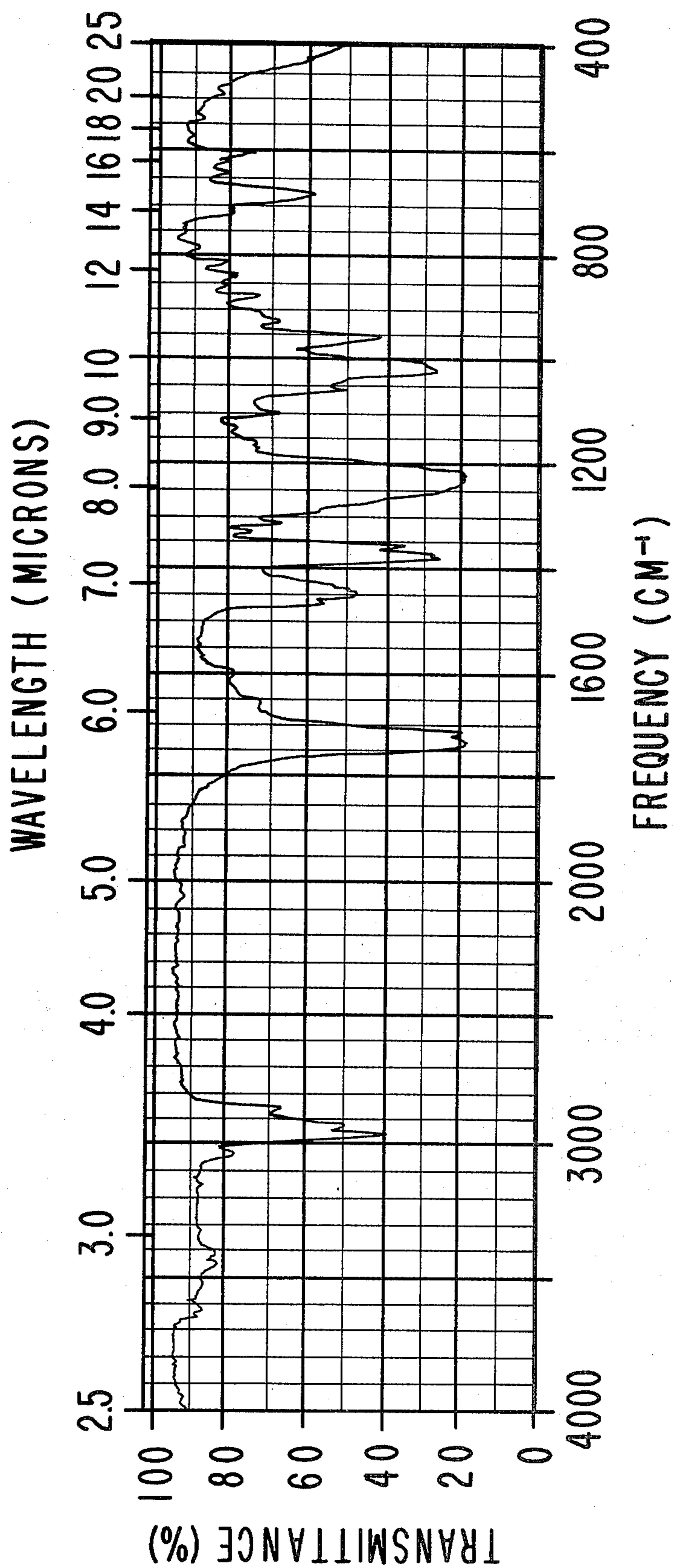
IR SPECTRUM FOR PEAK 162 OF FIG. 16 FOR EXAMPLE IV.
