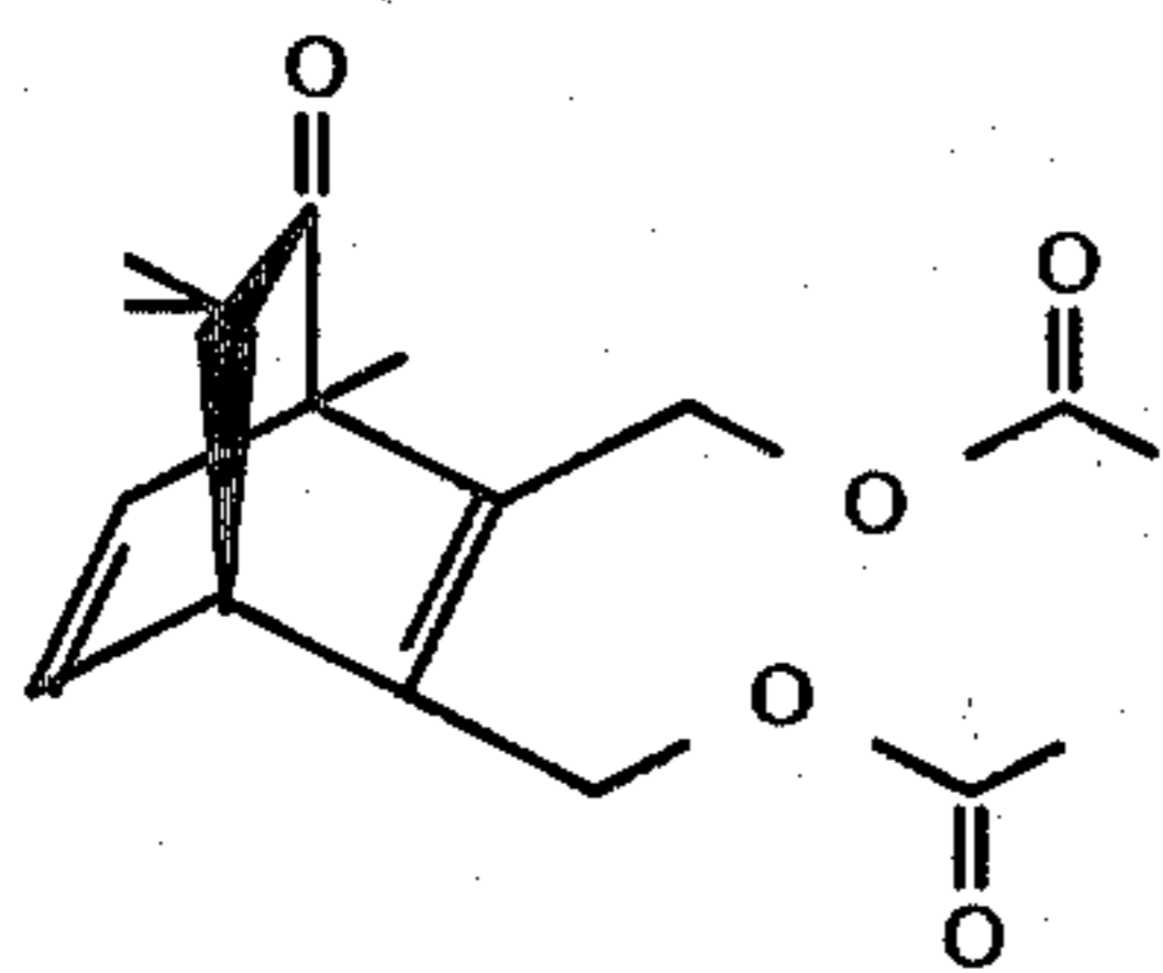
FIG. 17 is the mass spectrum for the peak indicated by reference numeral "162" of FIG. 16 for the compound produced according to Example IV having the structure:
