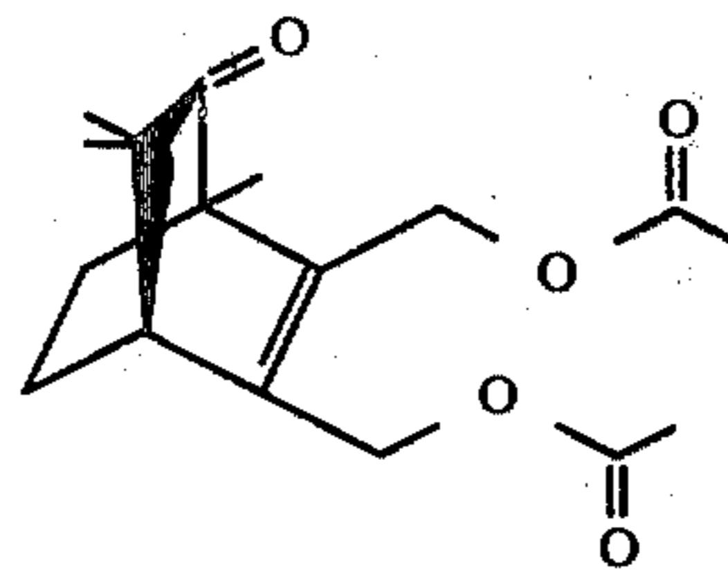
FIG. 21 is the infra-red spectrum for the compound of peak 201 of FIG. 20 which is for the compound produced according to Example V having the structure:
