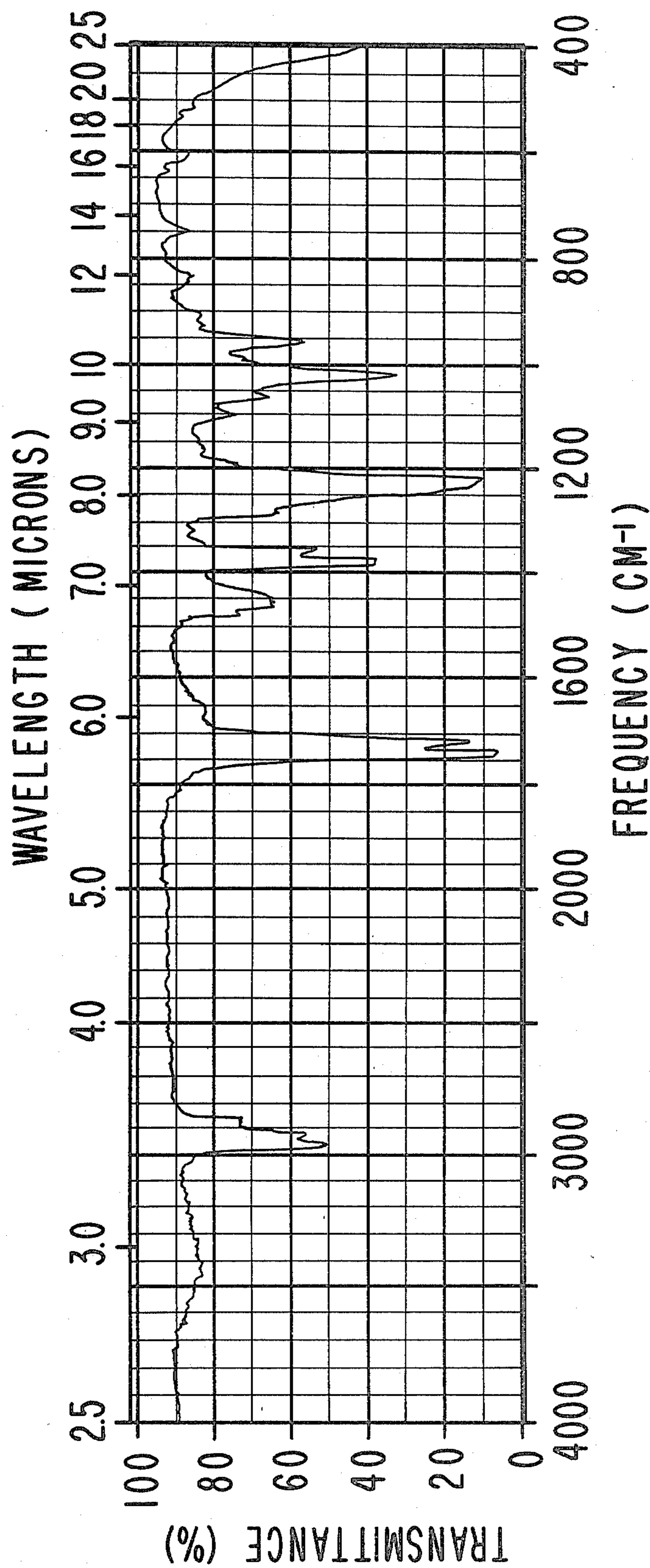
IR SPECTRUM FOR PEAK 201 OF FIG. 20 FOR EXAMPLE V.
