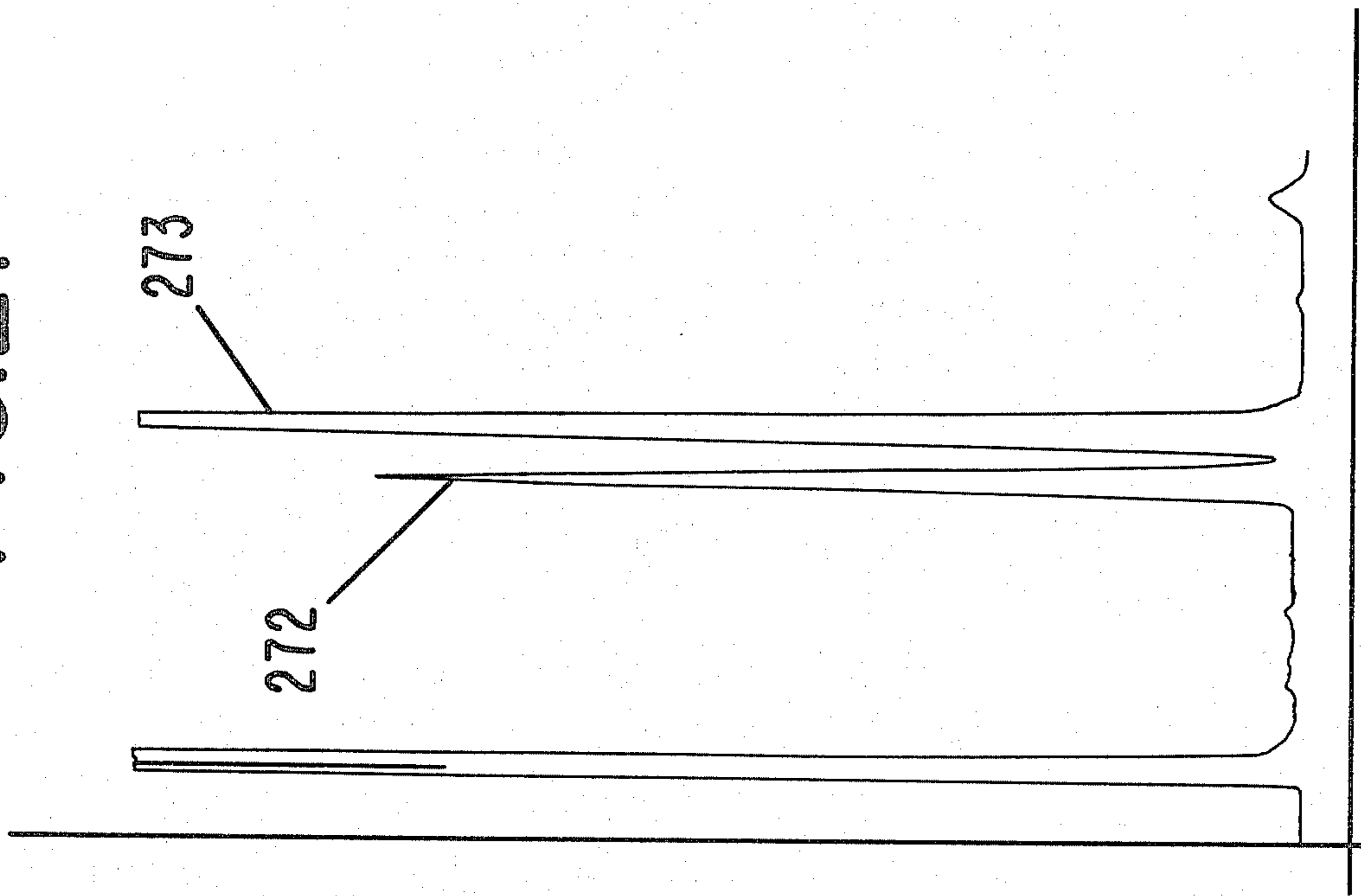
GLC PROFILE FOR EXAMPLE XX (B)
