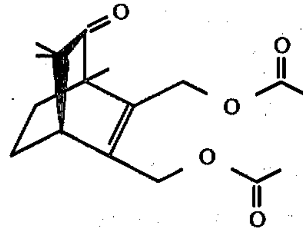
FIG. 23 is the mass spectrum for the compound of the peak indicated by reference numeral "201" of FIG. 20, the compound produced according to Example V having the structure:
