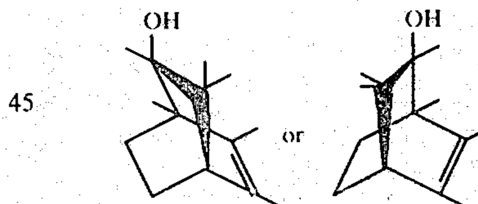
FIG. 8 is the infra-red spectrum for the compound of peak 501 of FIG. 5 having the structure:
