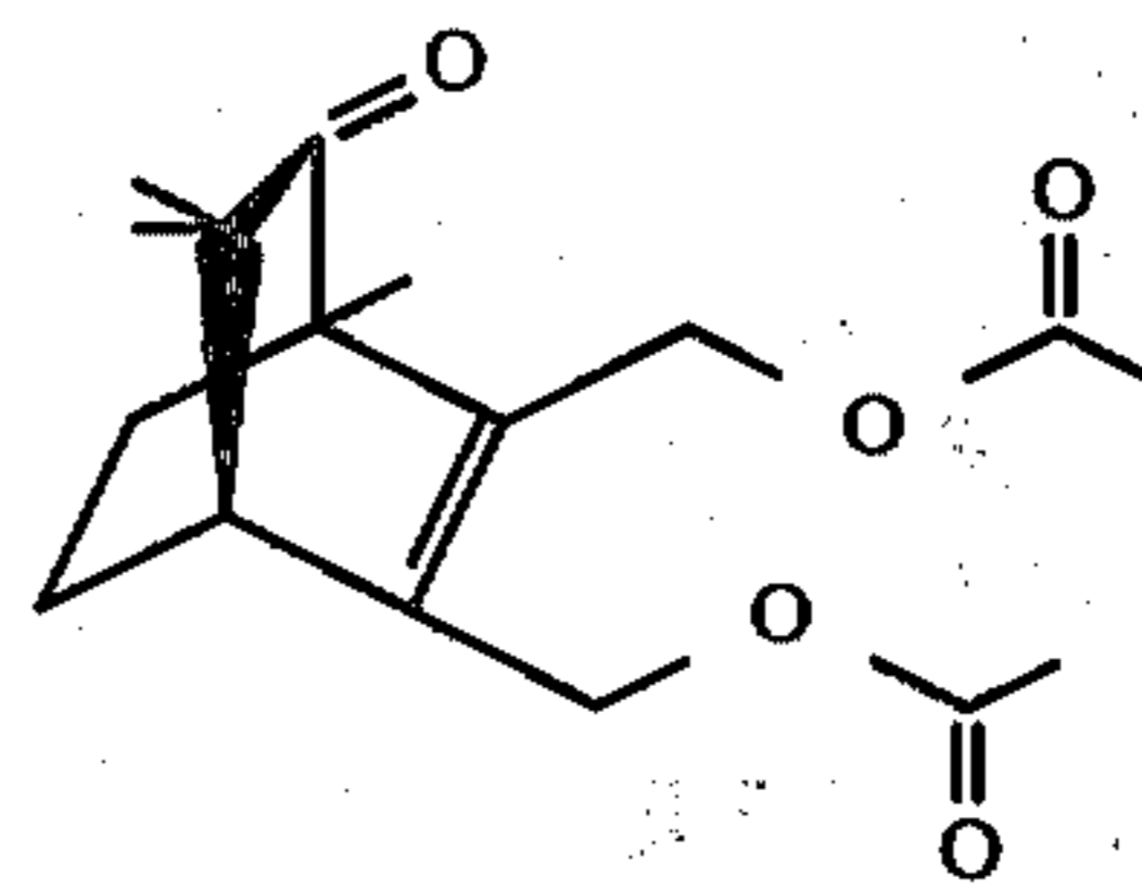
FIG. 22 is the NMR spectrum for the compound of the peak indicated by reference numeral "201" of FIG. 20, the compound produced according to Example V having the structure:
