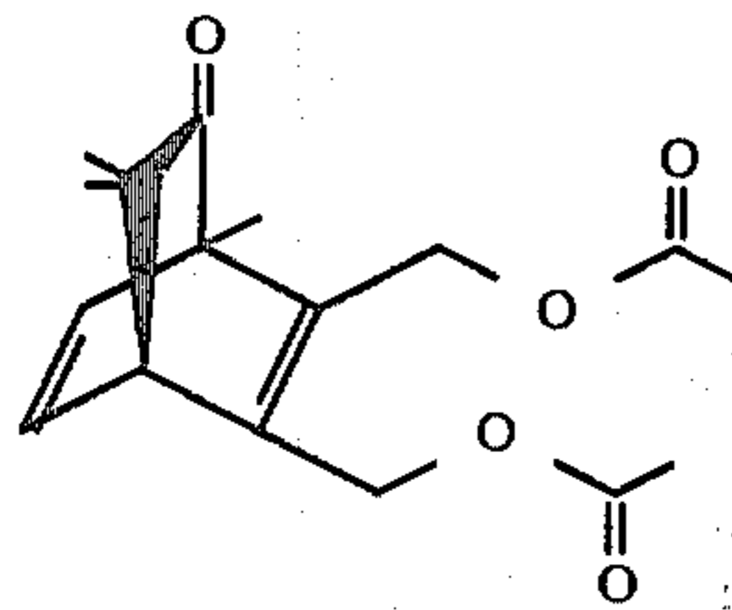
FIG. 19 is the NMR spectrum for the compound of the peak indicated by reference numeral "162" of FIG. 16 for the compound produced according to Example IV having the structure:
