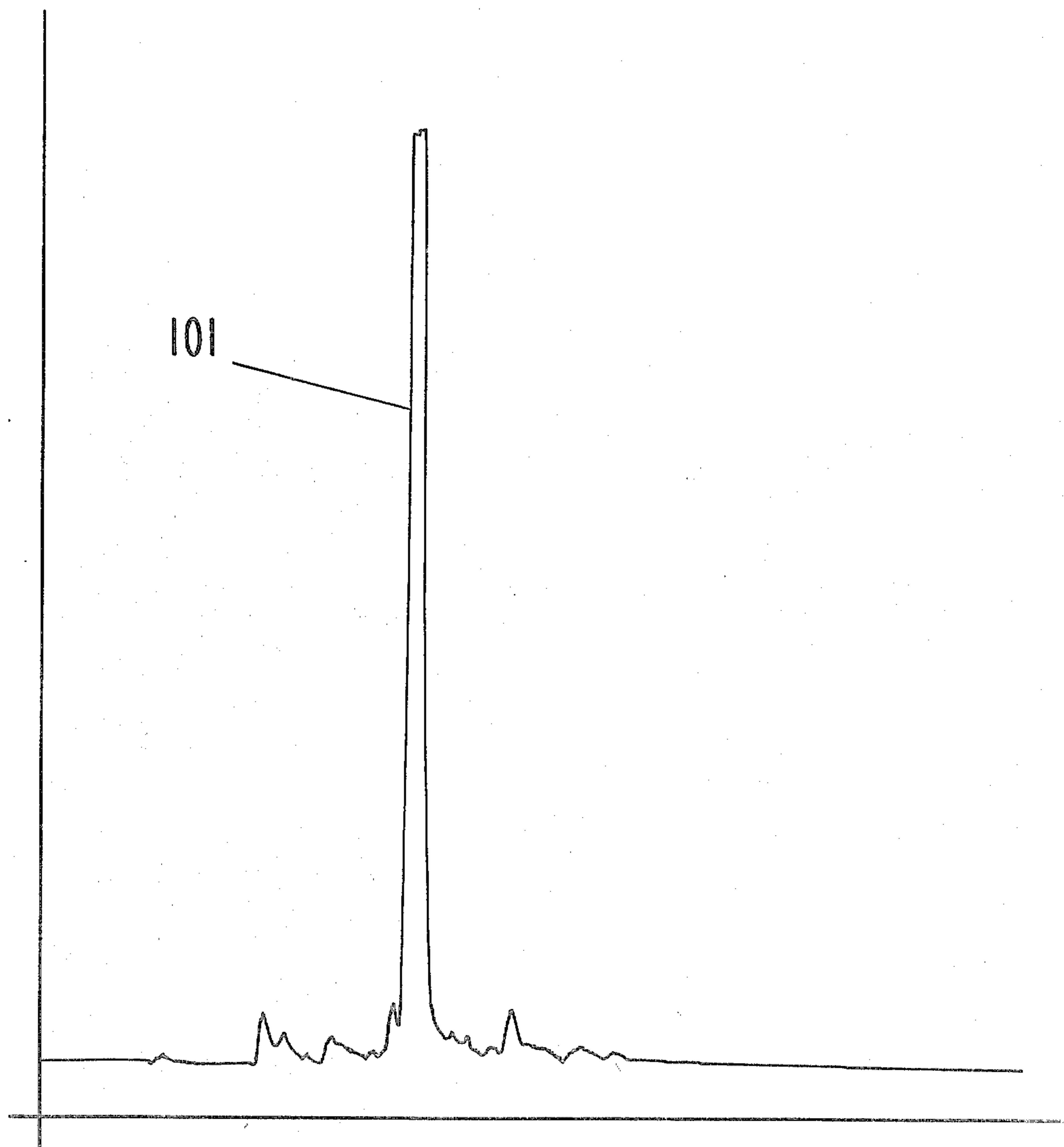
GLC PROFILE FOR EXAMPLE I.
