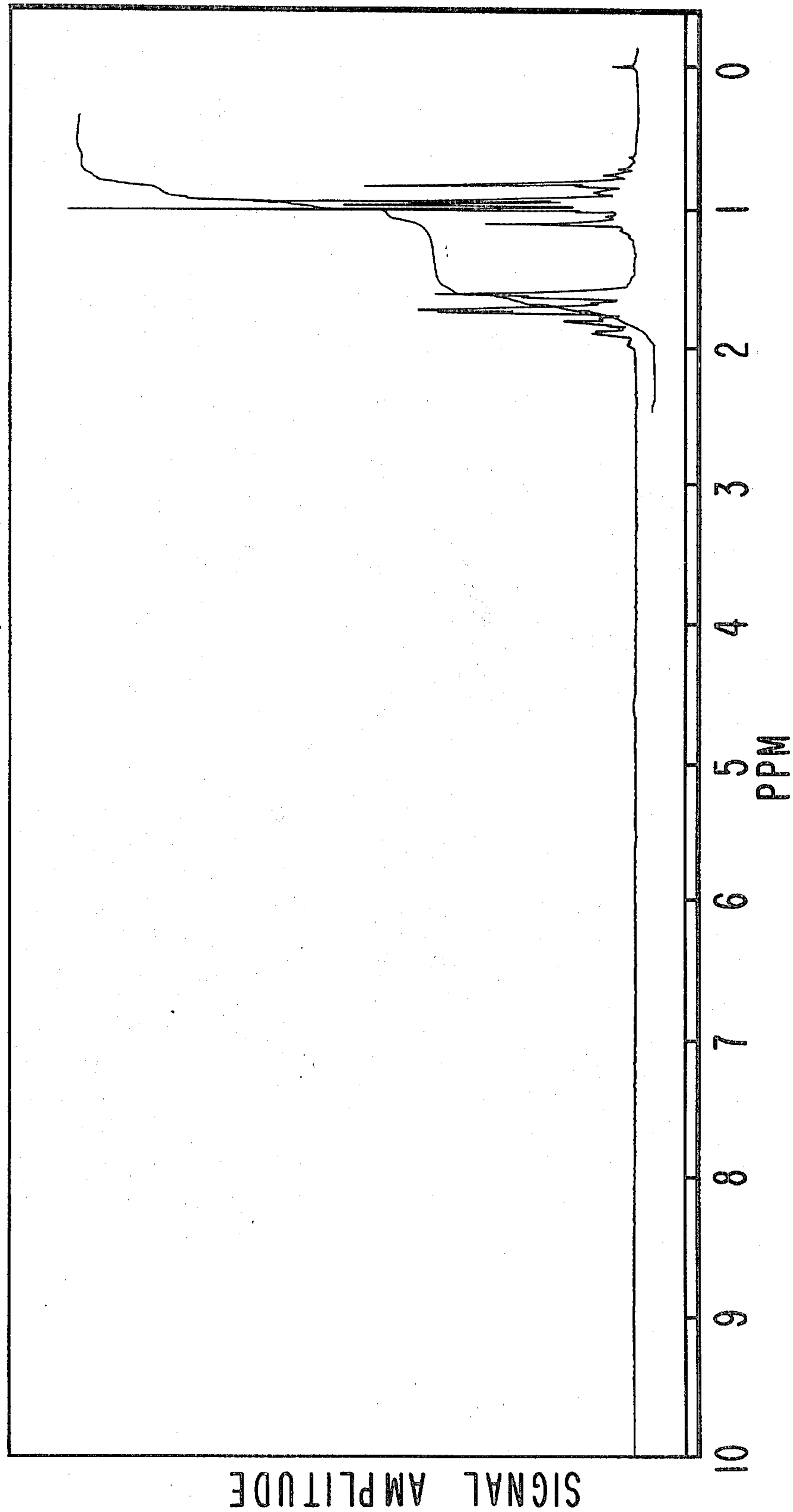
NMR SPECTRUM FOR PEAK 902 OF FIG.9, EXAMPLE III.
