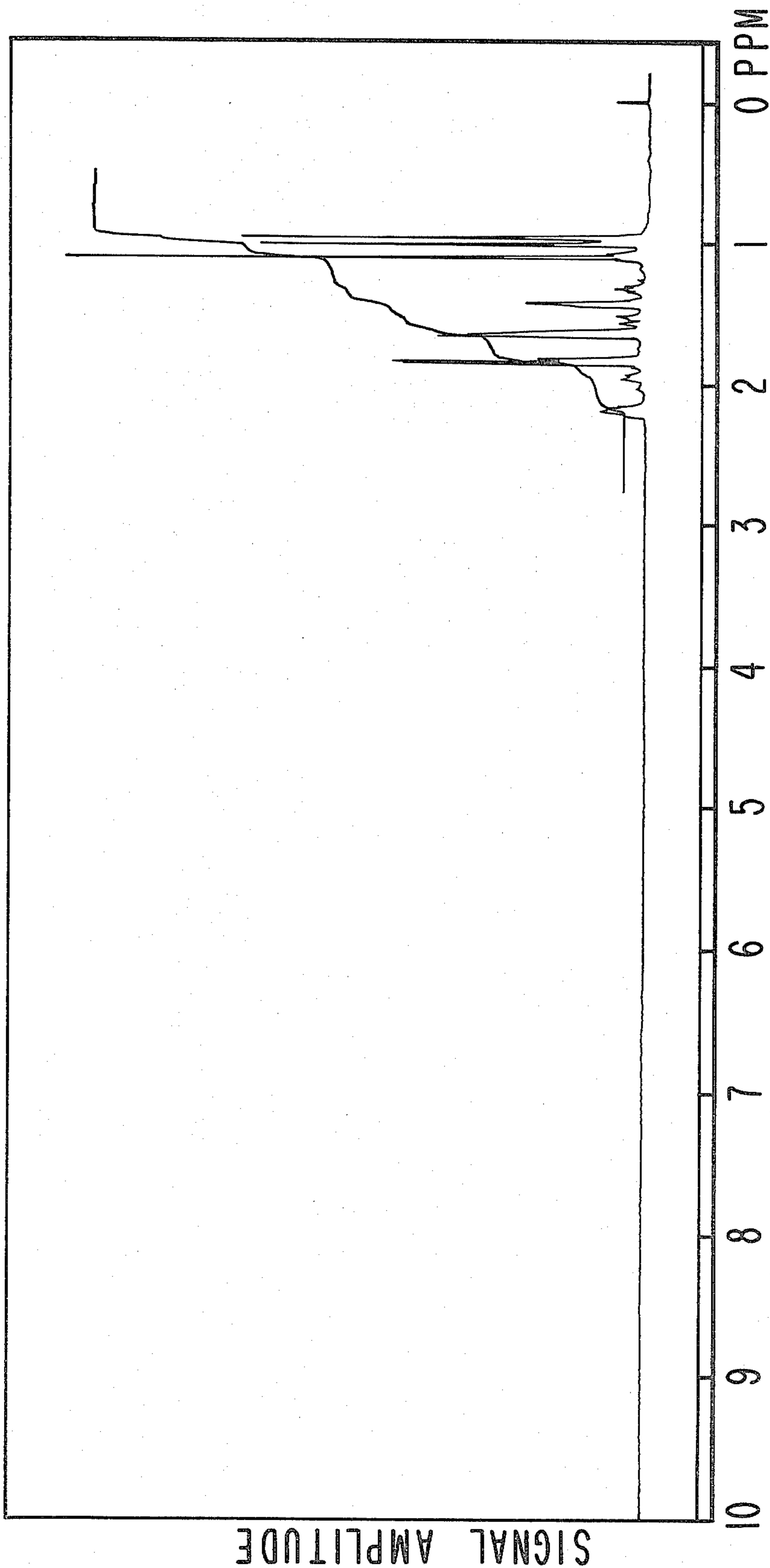
NMR SPECTRUM FOR PEAK 501 OF FIG. 5, EXAMPLE II.
