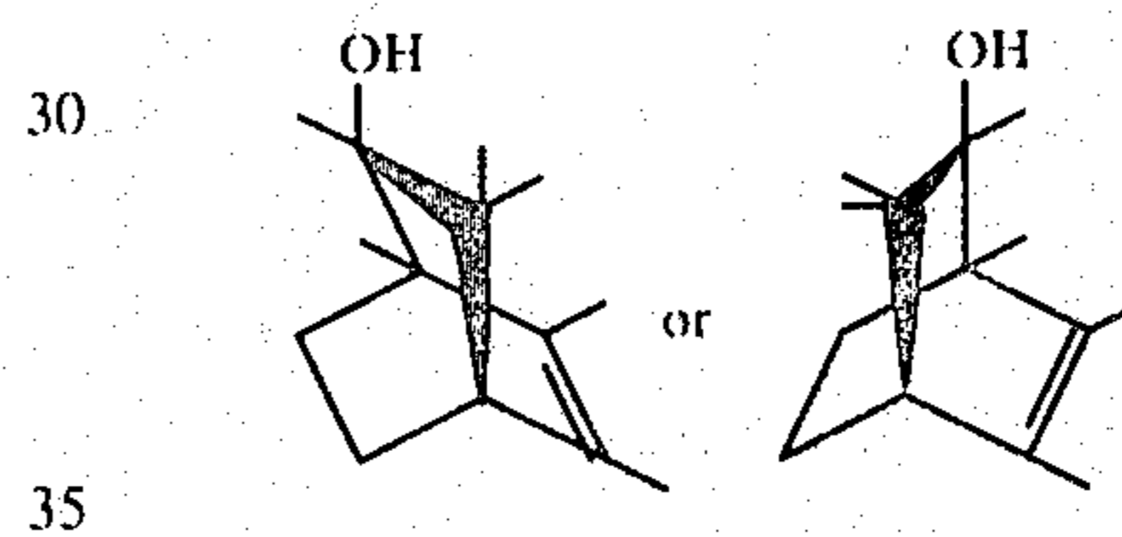
FIG. 7 is the NMR spectrum for the compound of peak 501 of FIG. 5 having the structure:
