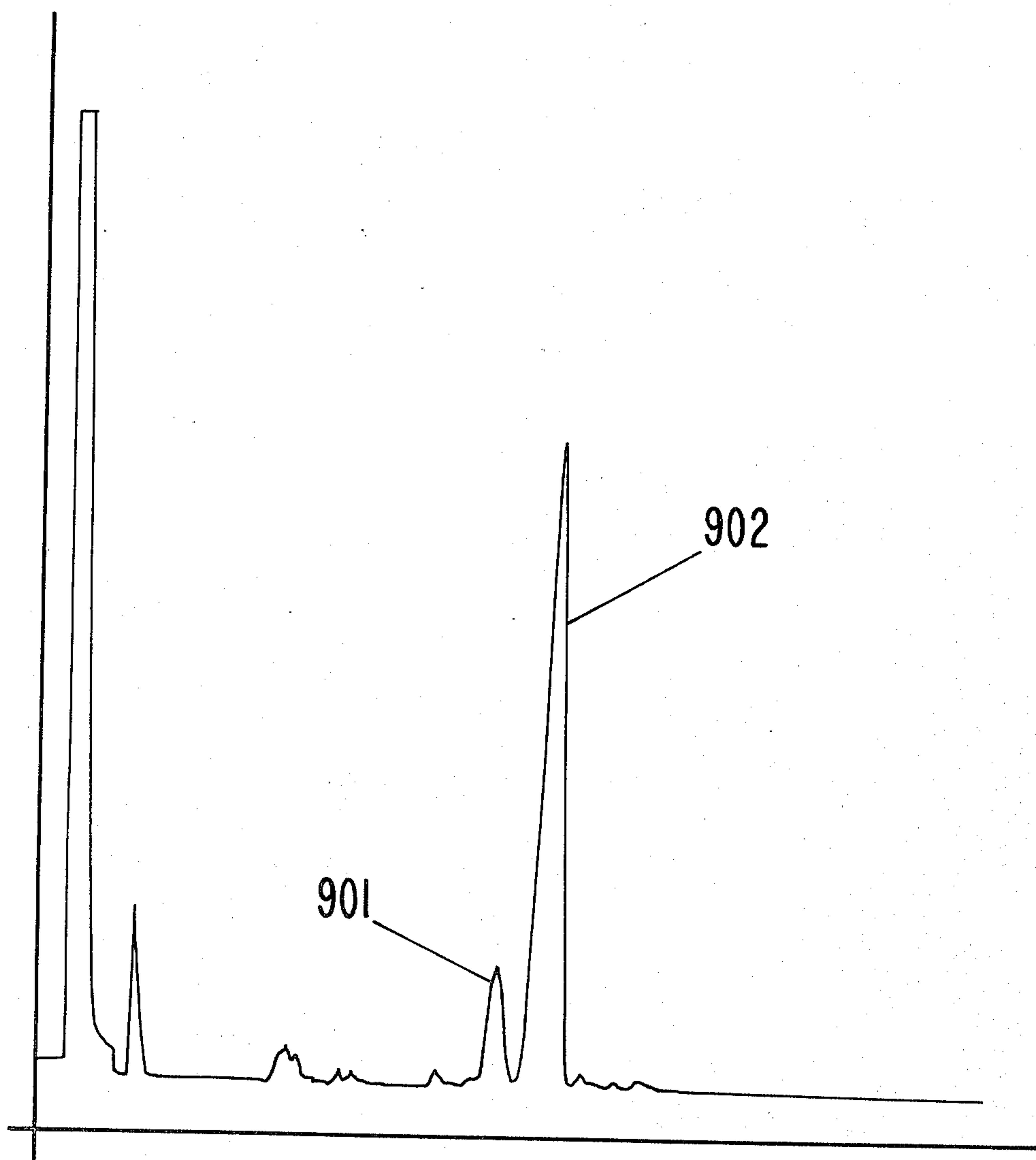
GLC PROFILE FOR EXAMPLE III.
