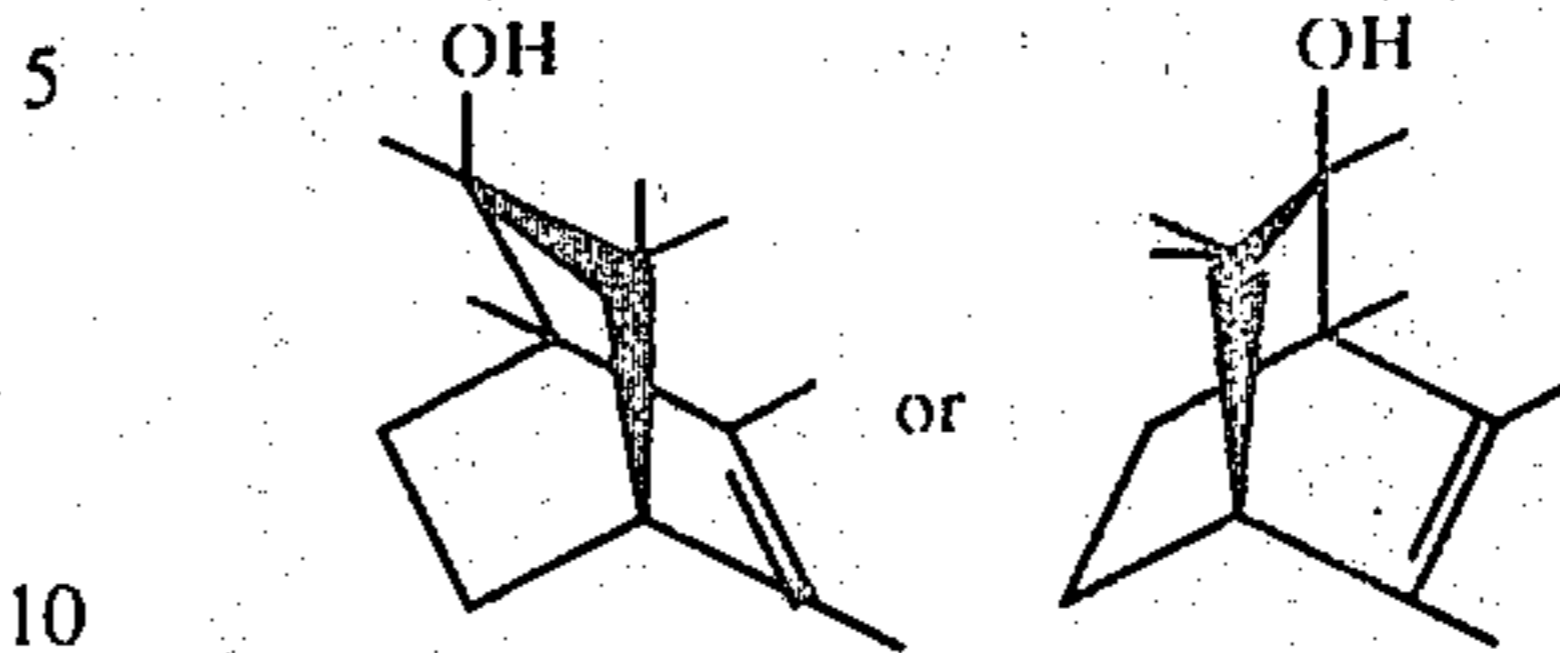
FIG. 11 is the infra-red spectrum for the compound of peak 901 of FIG. 9 having one of the structures:
