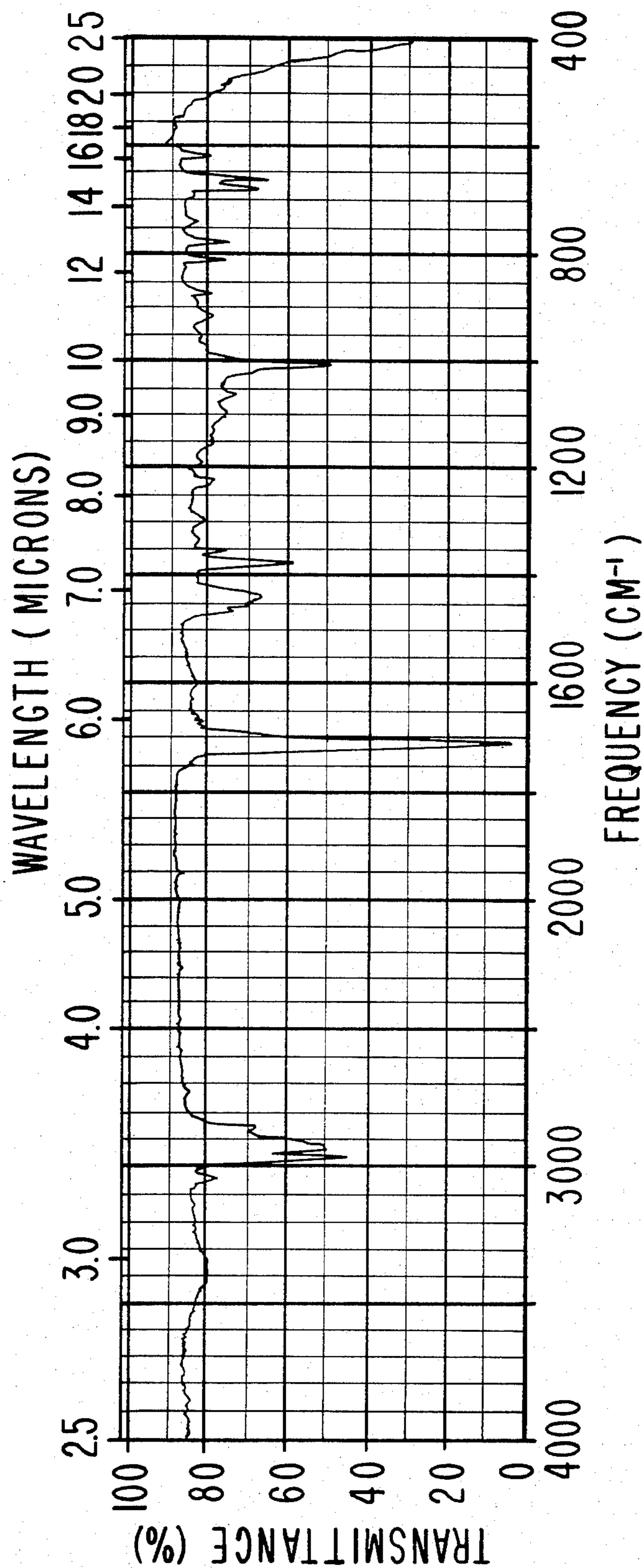
IR SPECTRUM FOR PEAK 101 OF FIG.1 FOR EXAMPLE I.
