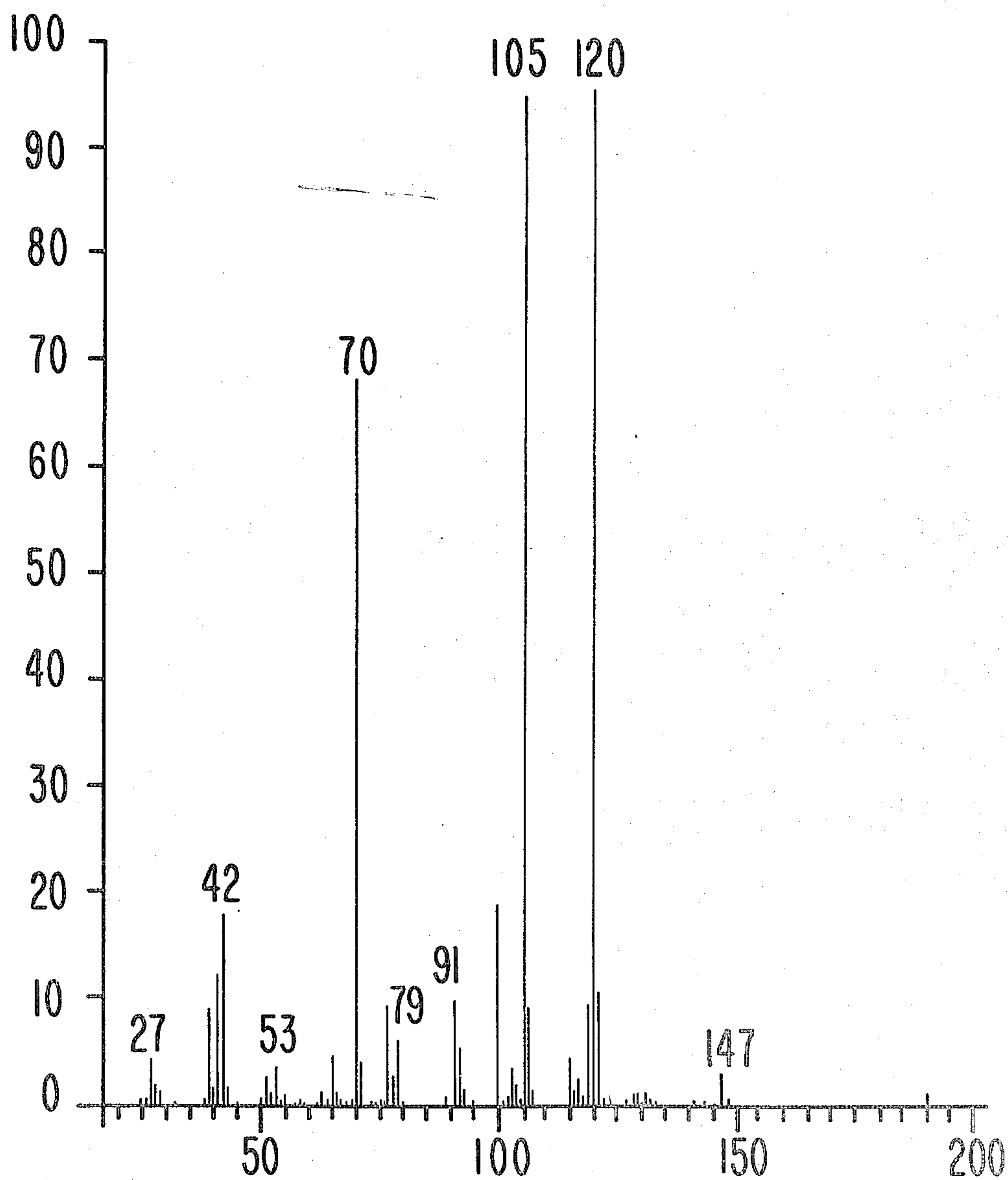
MASS SPECTRUM FOR PEAK 101 OF FIG. 1, EXAMPLE I.
