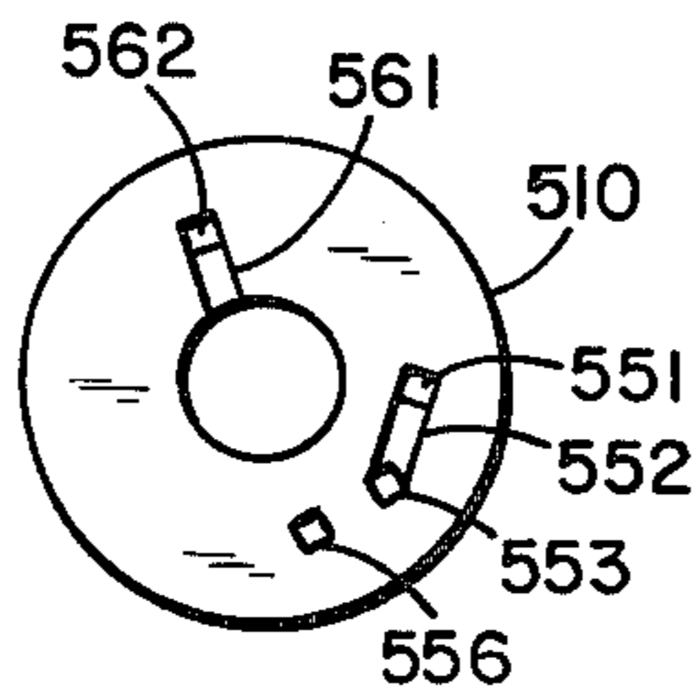
FIG. 3 (BOTTOM VIEW)
