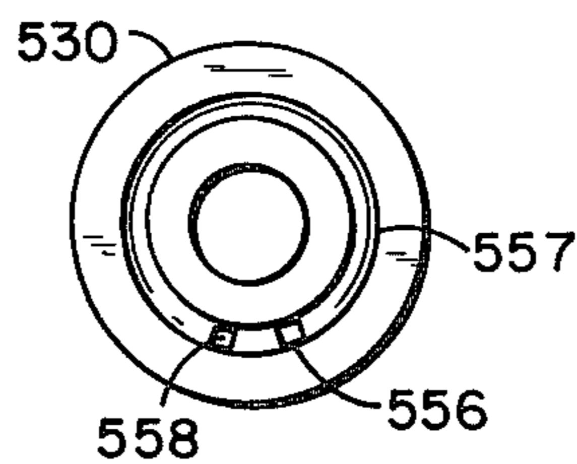
FIG. 5 (BOTTOM VIEW)
