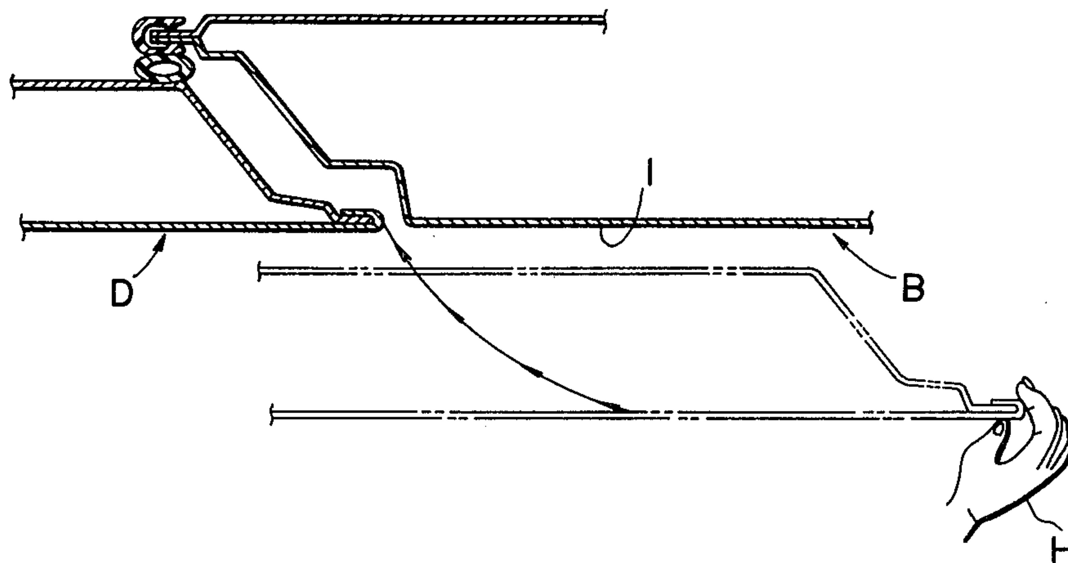
FIG. 3 (PRIOR ART)
