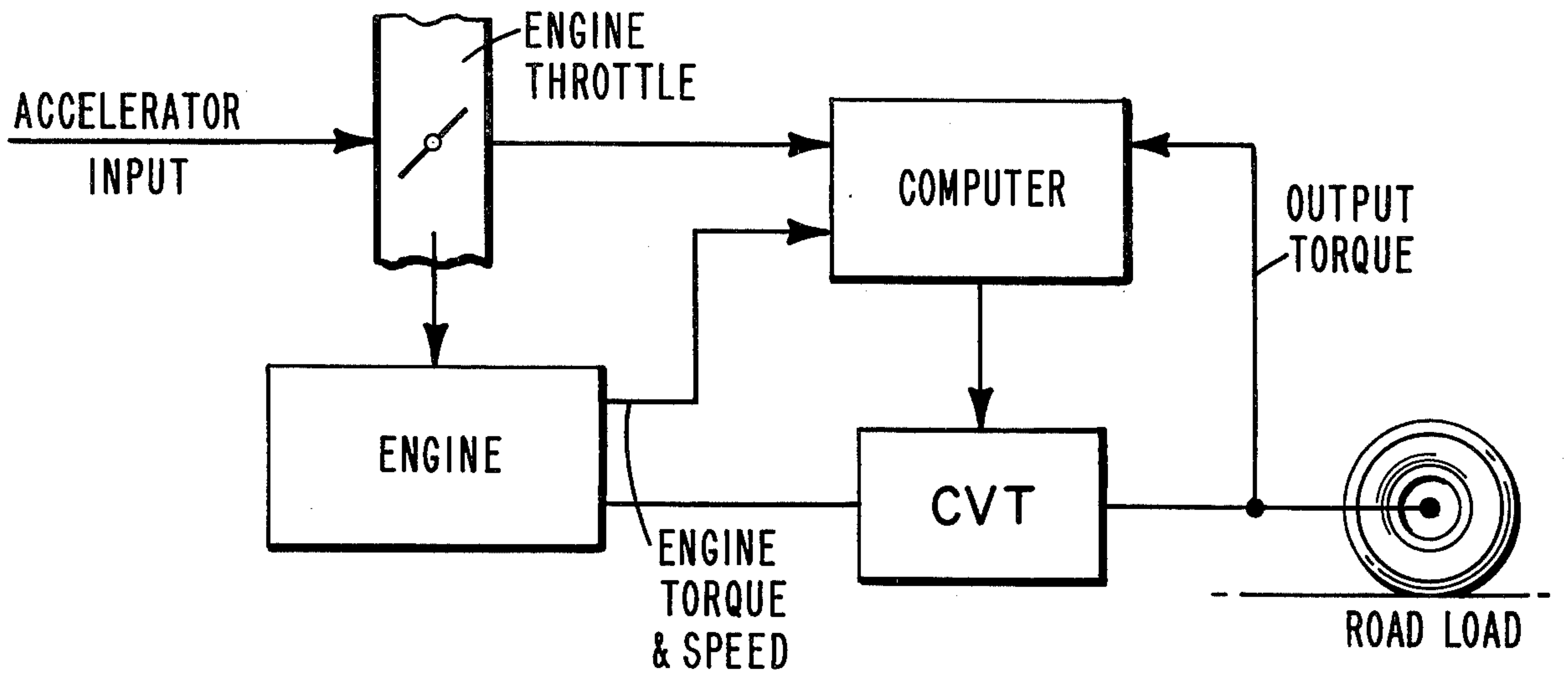
FIG. 3 PRIOR ART
