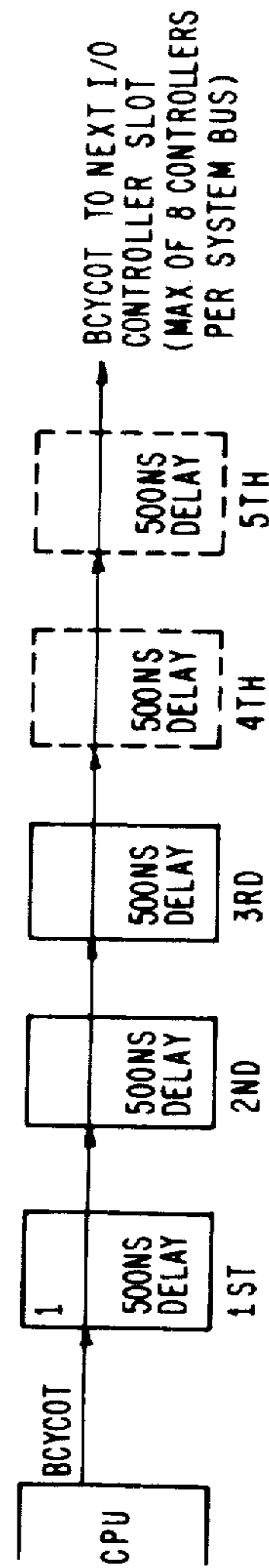
I/O CONTROLLERS ON SYSTEM BUS
