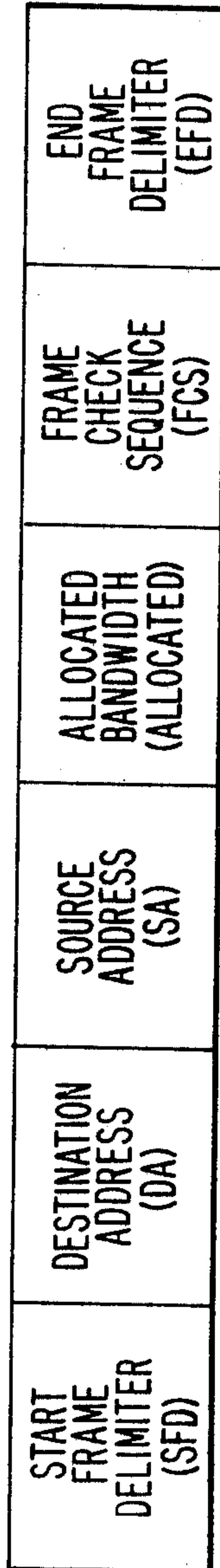
BANDWIDTH ALLOCATION TOKEN FORMAT
