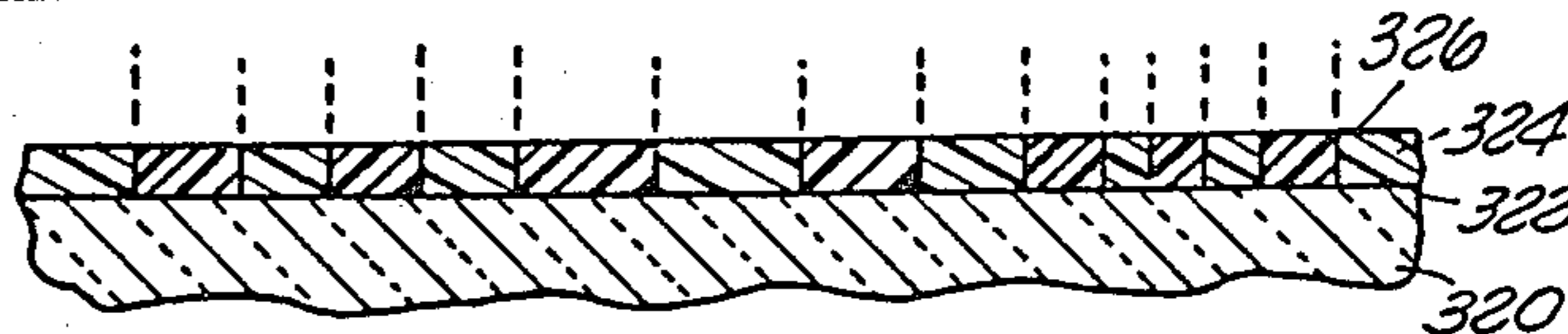
FIG. 6 CROSSECTION OF MASTER VIDEO DISC.
