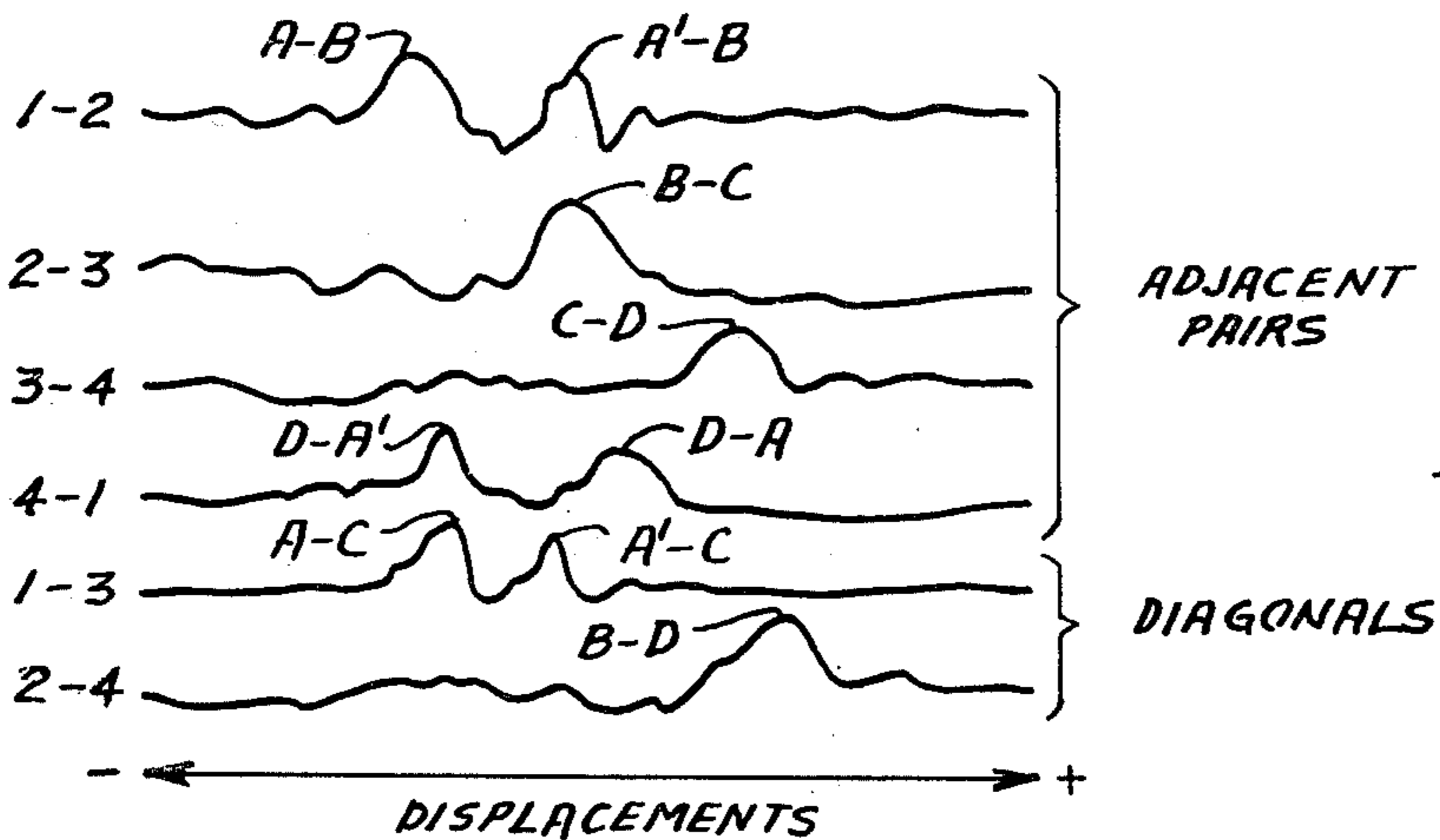
CORRELOGRAMS
