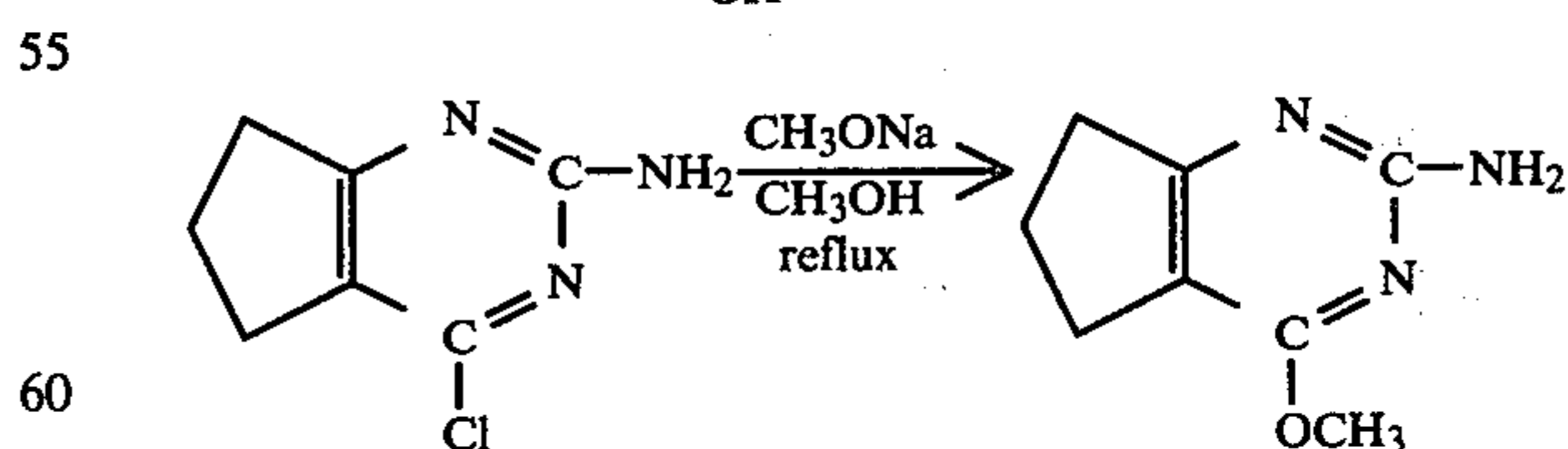
6,7-dihydro-4-methoxy-5H-cyclopentapyrimidin-2-amine.
