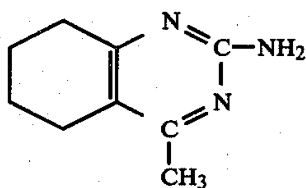
5,6,7,8-tetrahydro-4-methyl-2-quinazolinamine.
