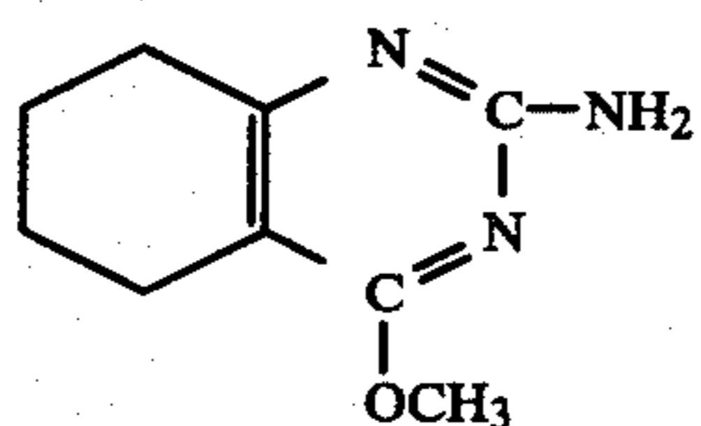
5,6,7,8-tetrahydro-4-methoxy-2-quinazolinamine.
