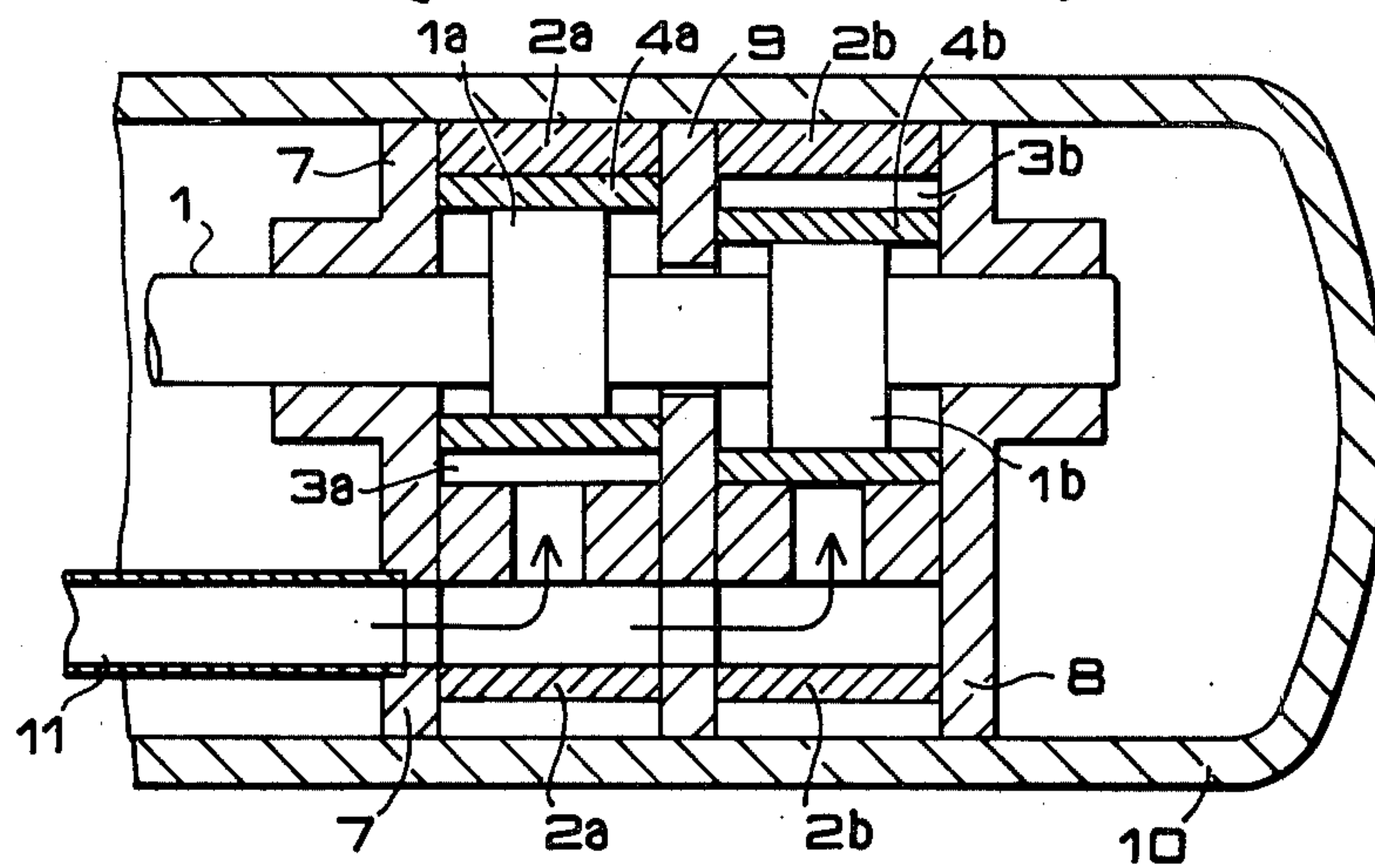
FIG. 1 (PRIOR ART)
