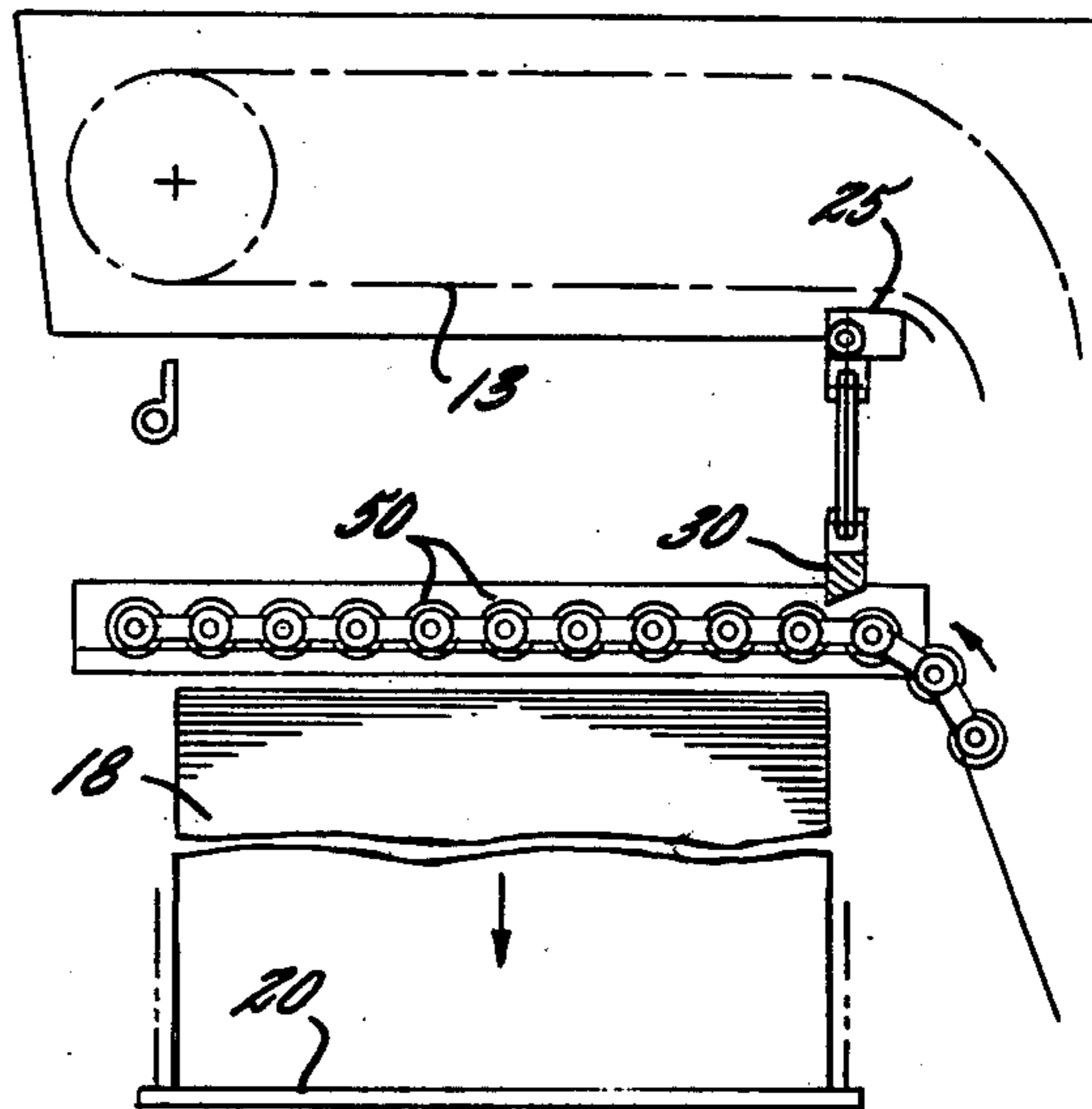
FIG. 7. FILLED PILE BOARD LOWERED ROLLERS INTERPOSED
