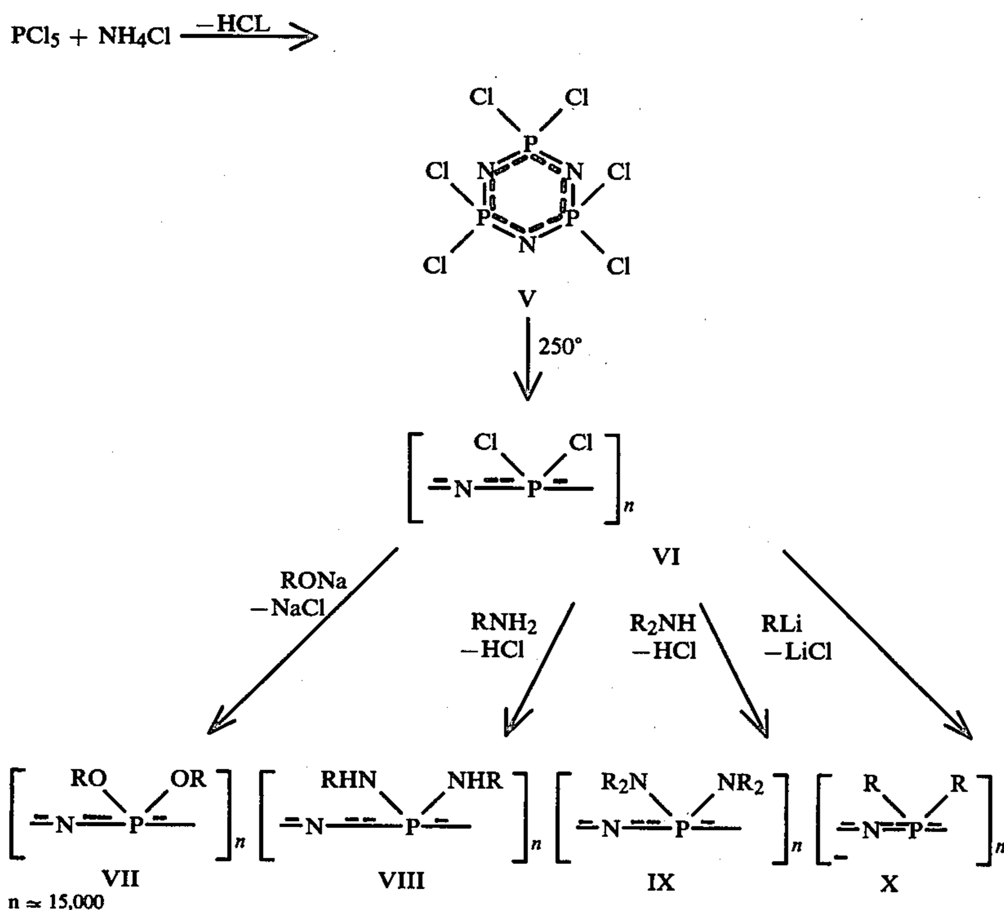
Scheme 1 General synthesis routes to poly- (organophosphazenes)
