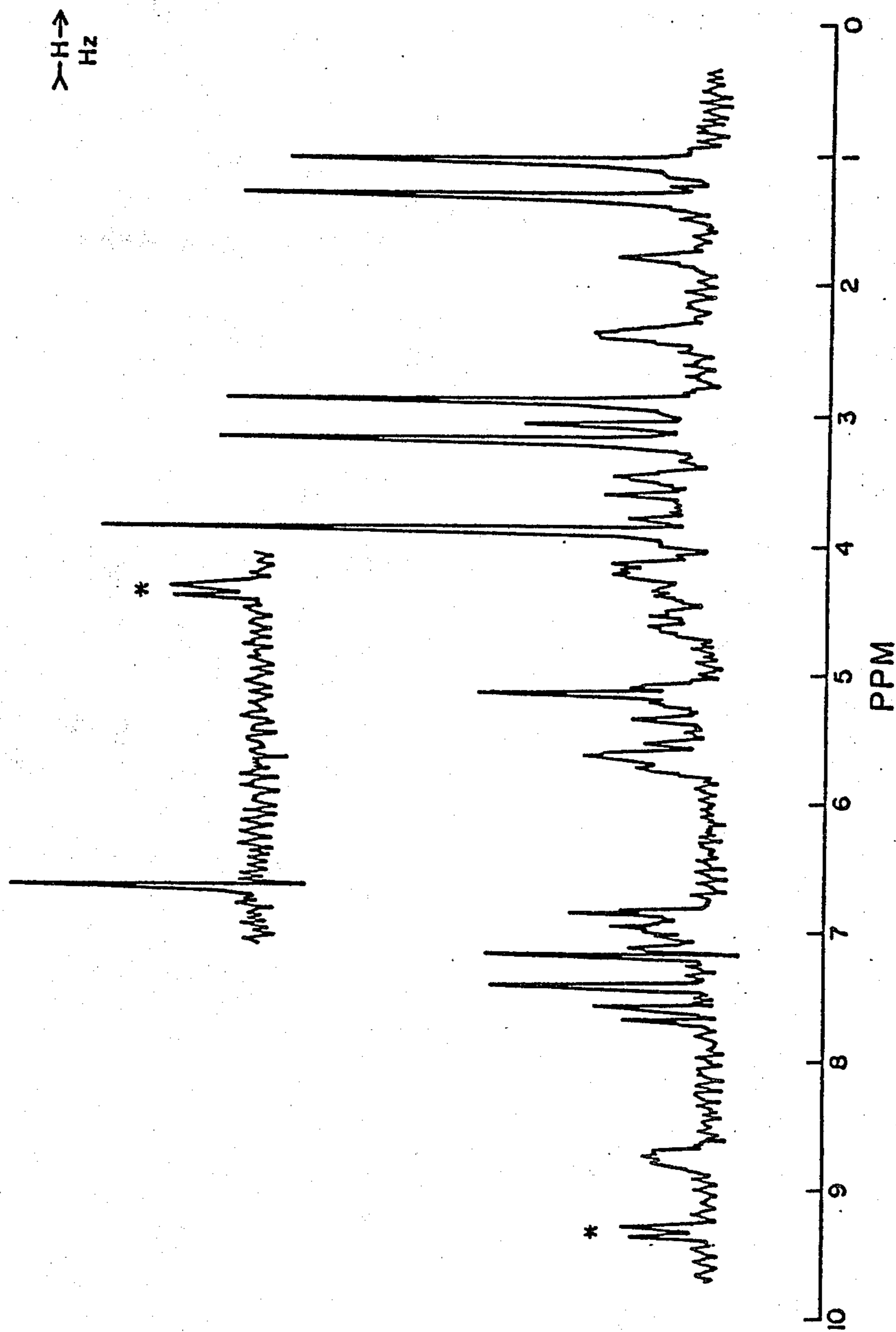
FIG. 7 NMR SPECTRUM OF BBM-928 C
