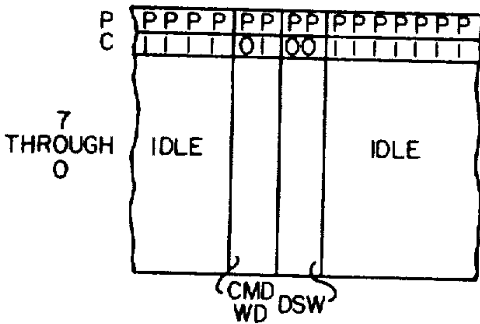
B. MESSAGE FORMAT (CONTROL/STATUS PRIMARY MESSAGES)
