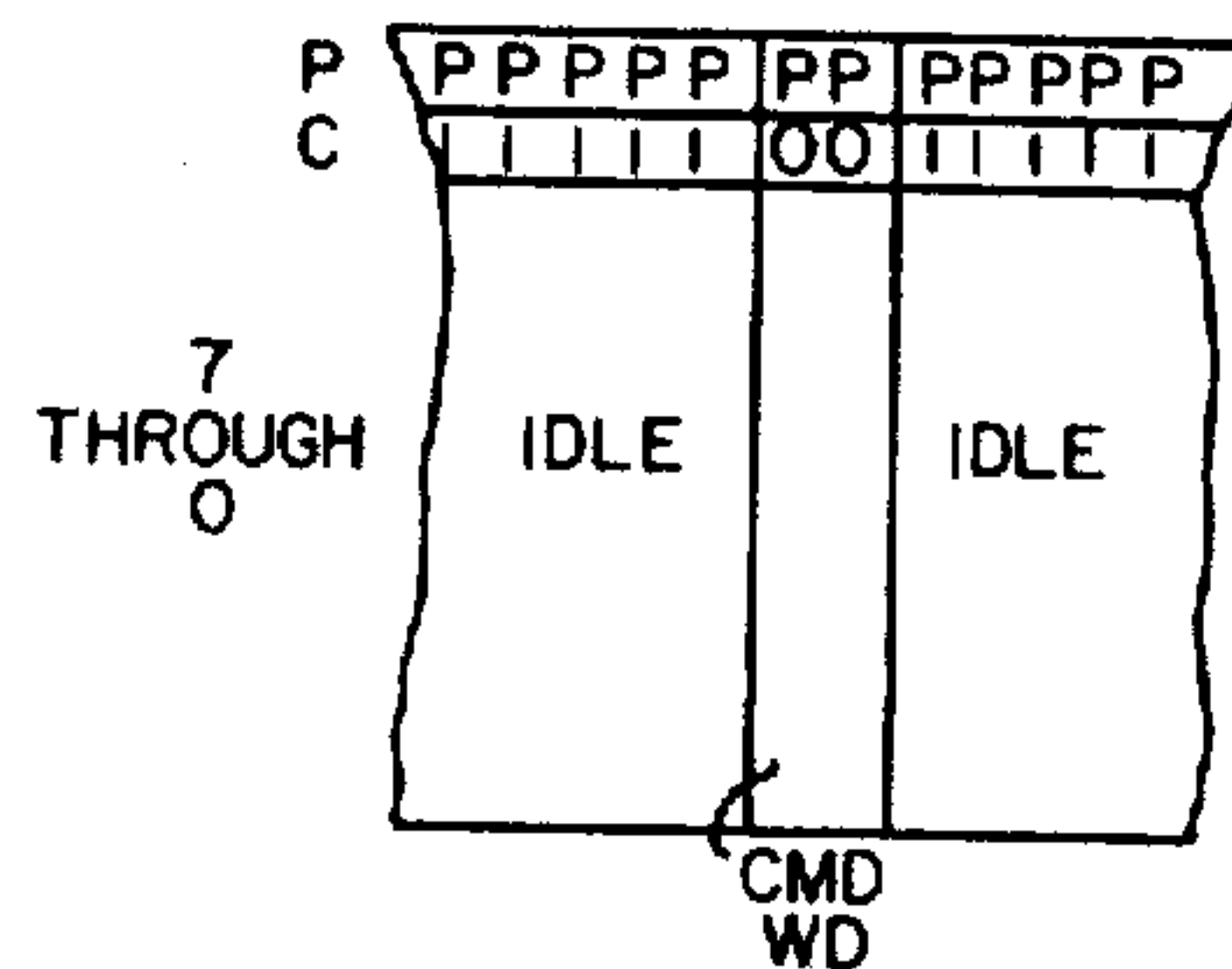
C. MESSAGE FORMAT (RESPONSE MESSAGE. ACK NAK SACK NAP)
