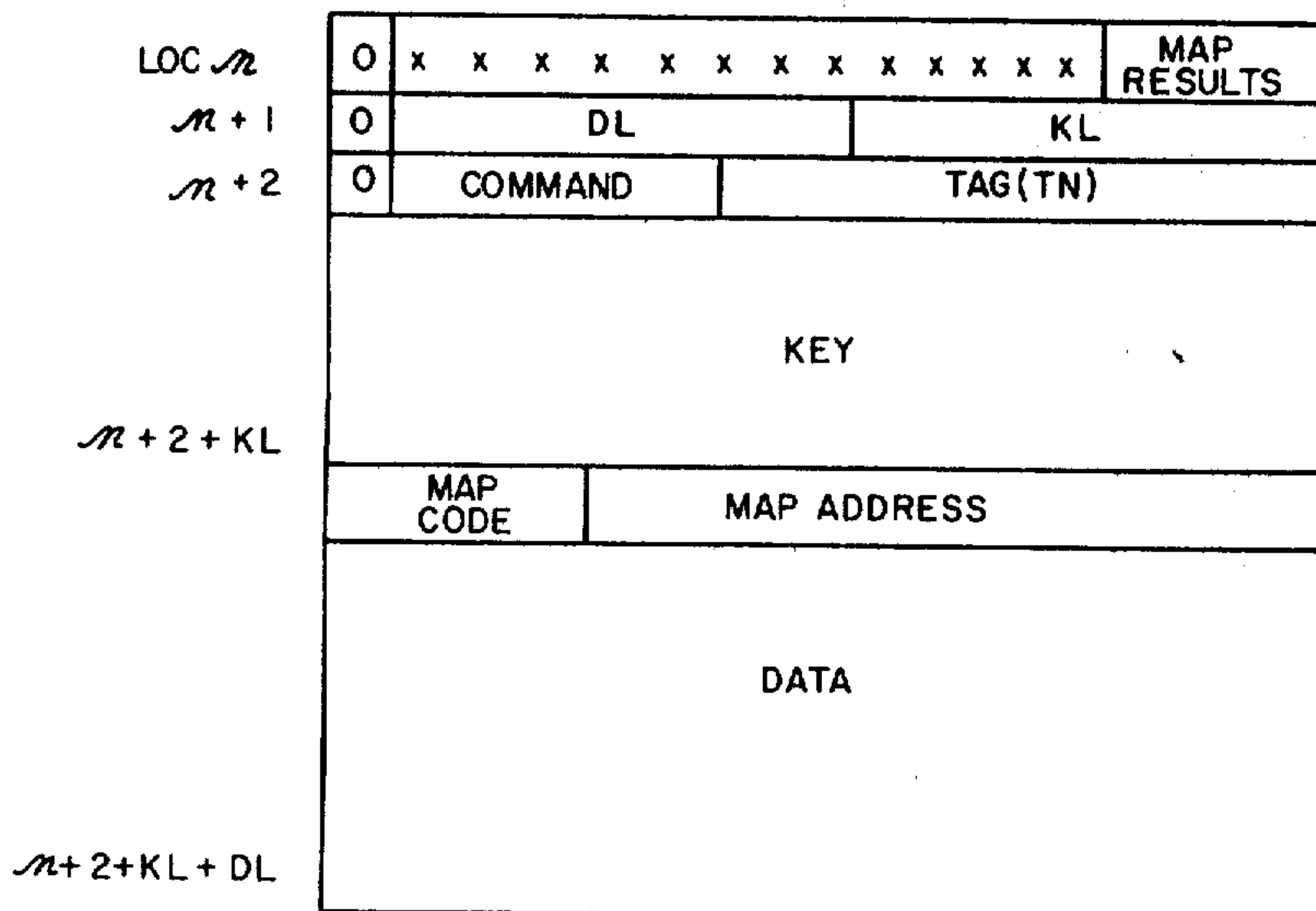
B. RECEIVE MESSAGE FORMAT
