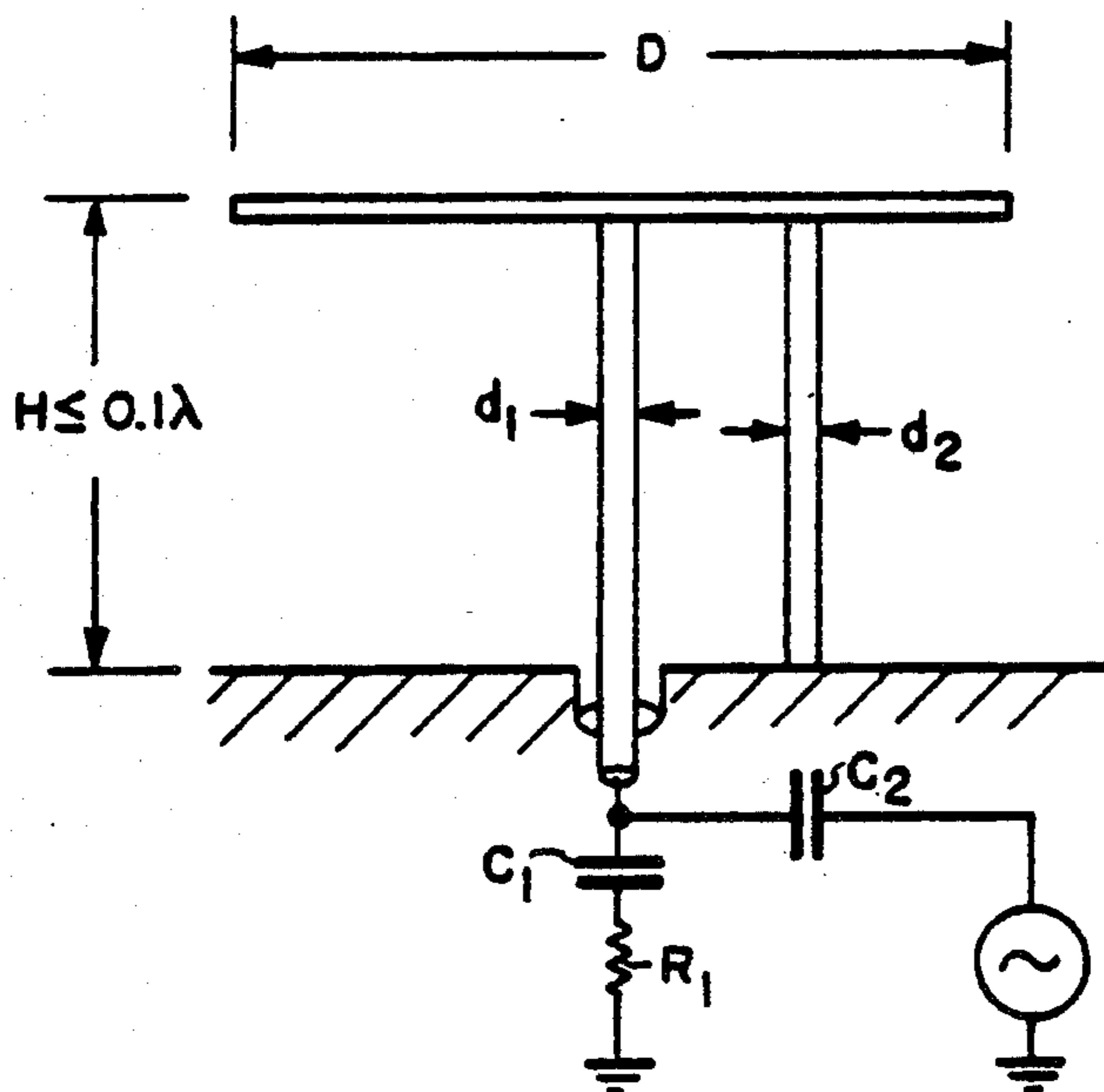
TOP-LOADED, FOLDED ANTENNA WITH "L"-NETWORK AND REVERSE CHARACTERISTIC NETWORKS.
