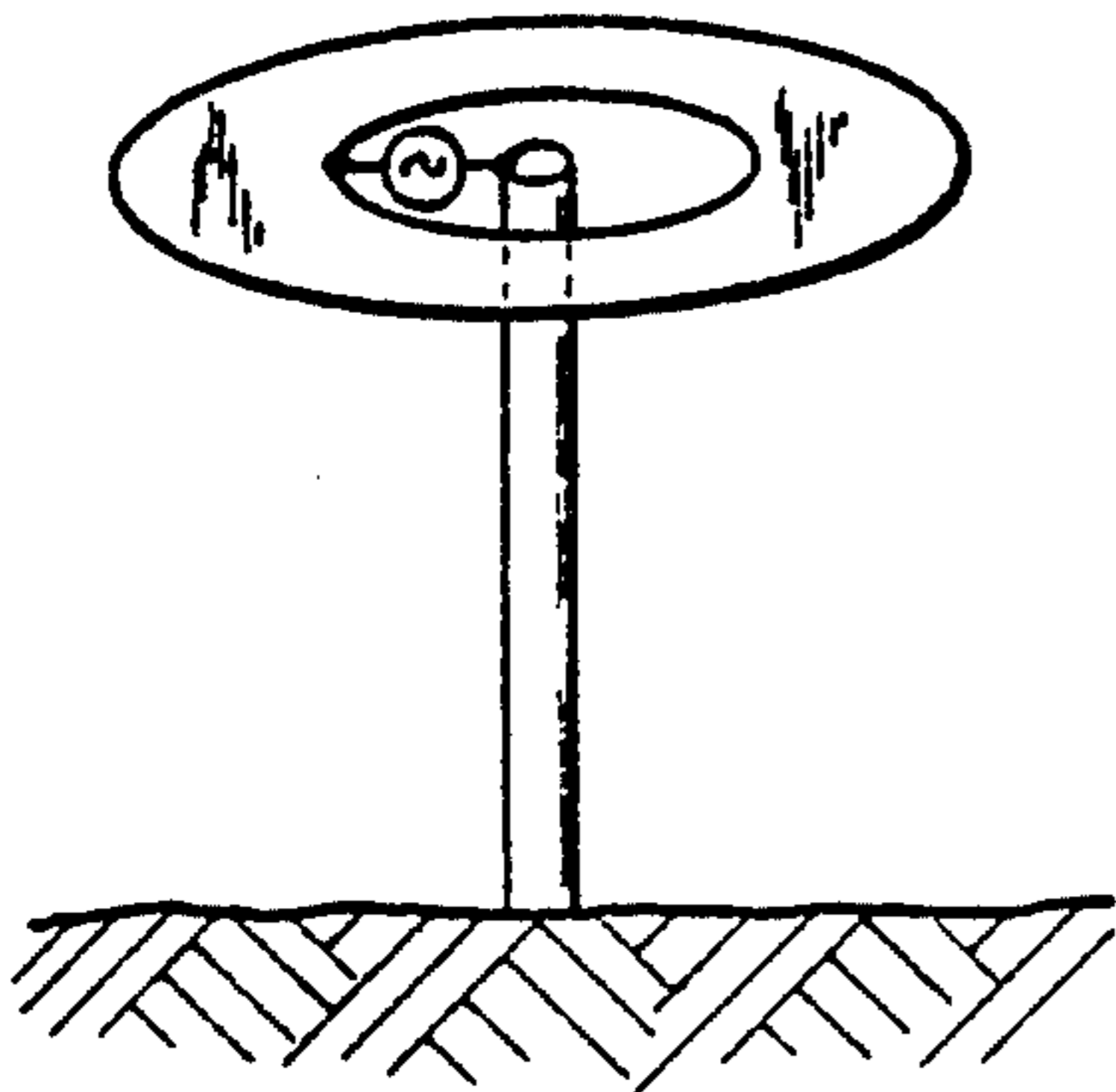
FIG. 4 GROUNDED-BASE, TOP-LOADED ANTENNA
