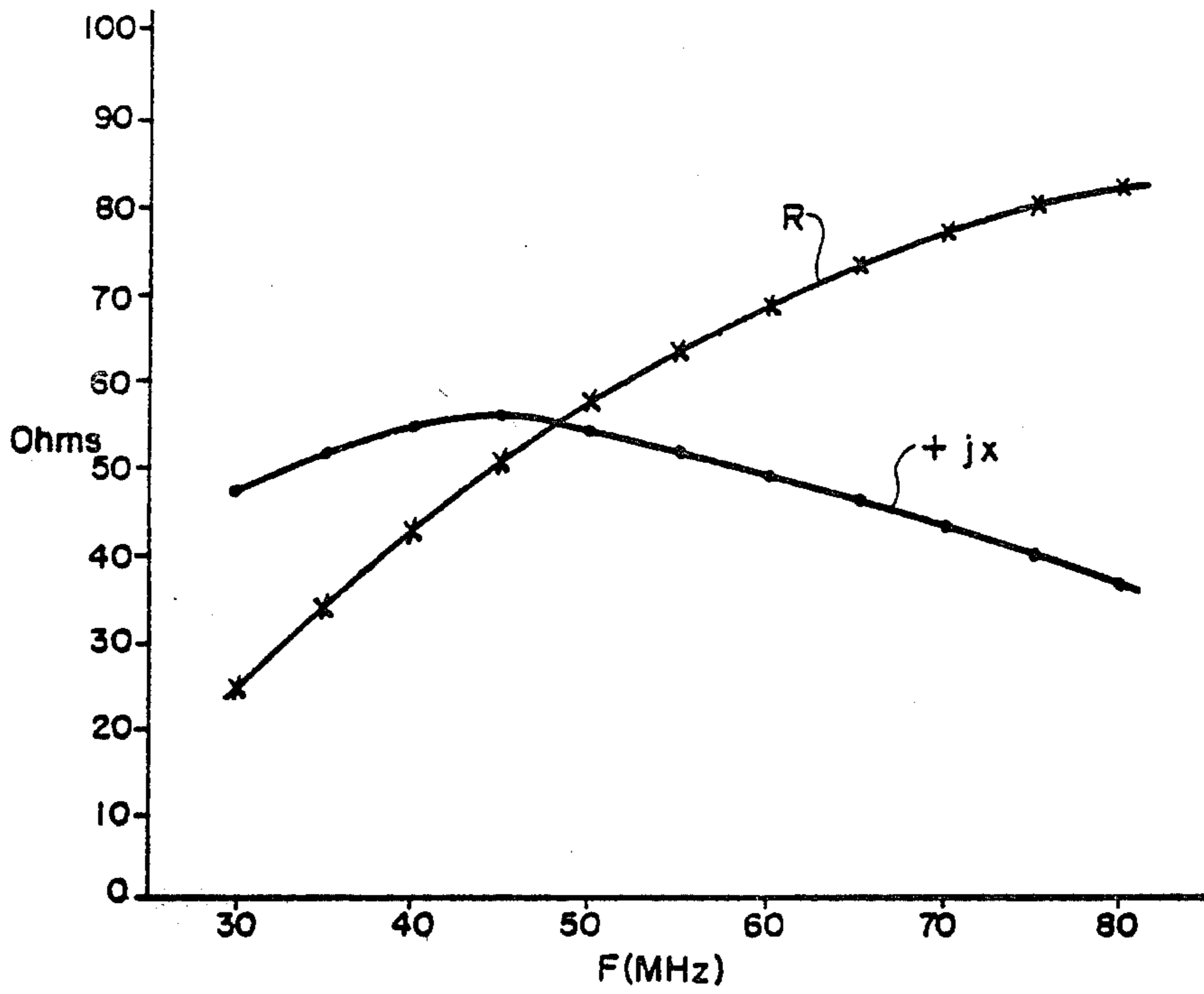
FIG. 9 MEASURED IMPEDANCE vs FREQUENCY
