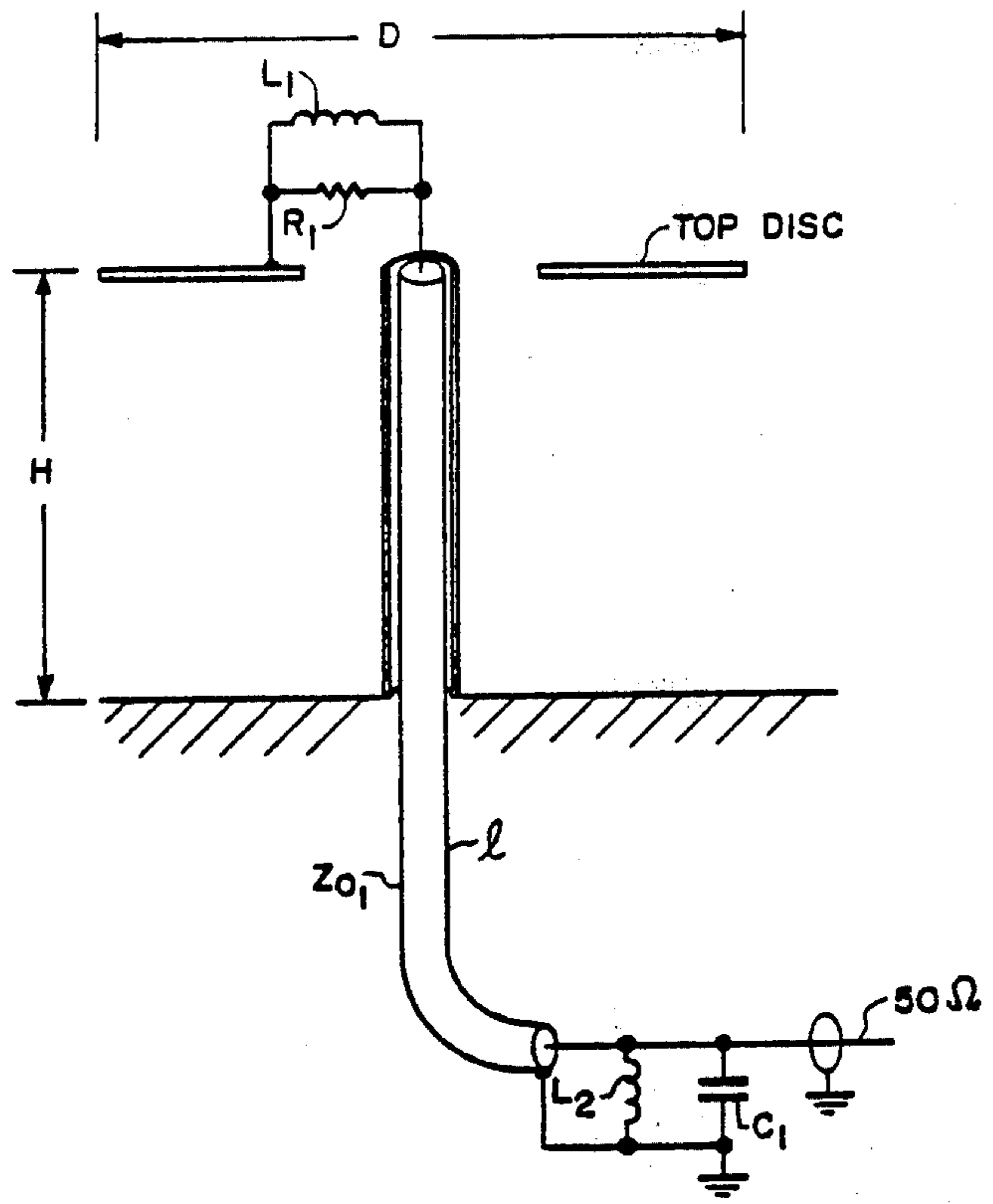
FIG. 11 GROUND BASE TOP-LOADED MONOPOLE
