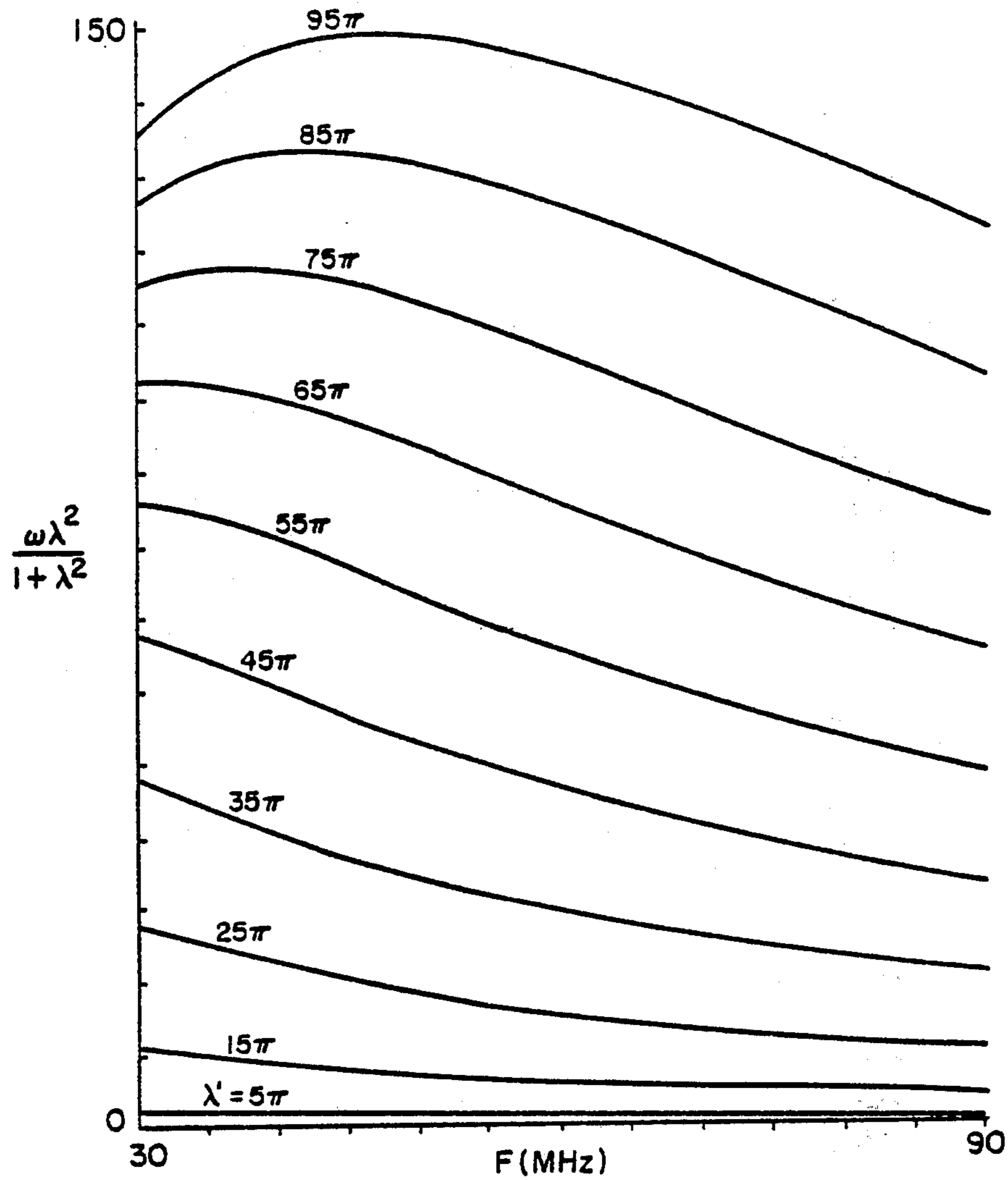
FIG. 3 SERIES REACTANCE, R/L NETWORK
