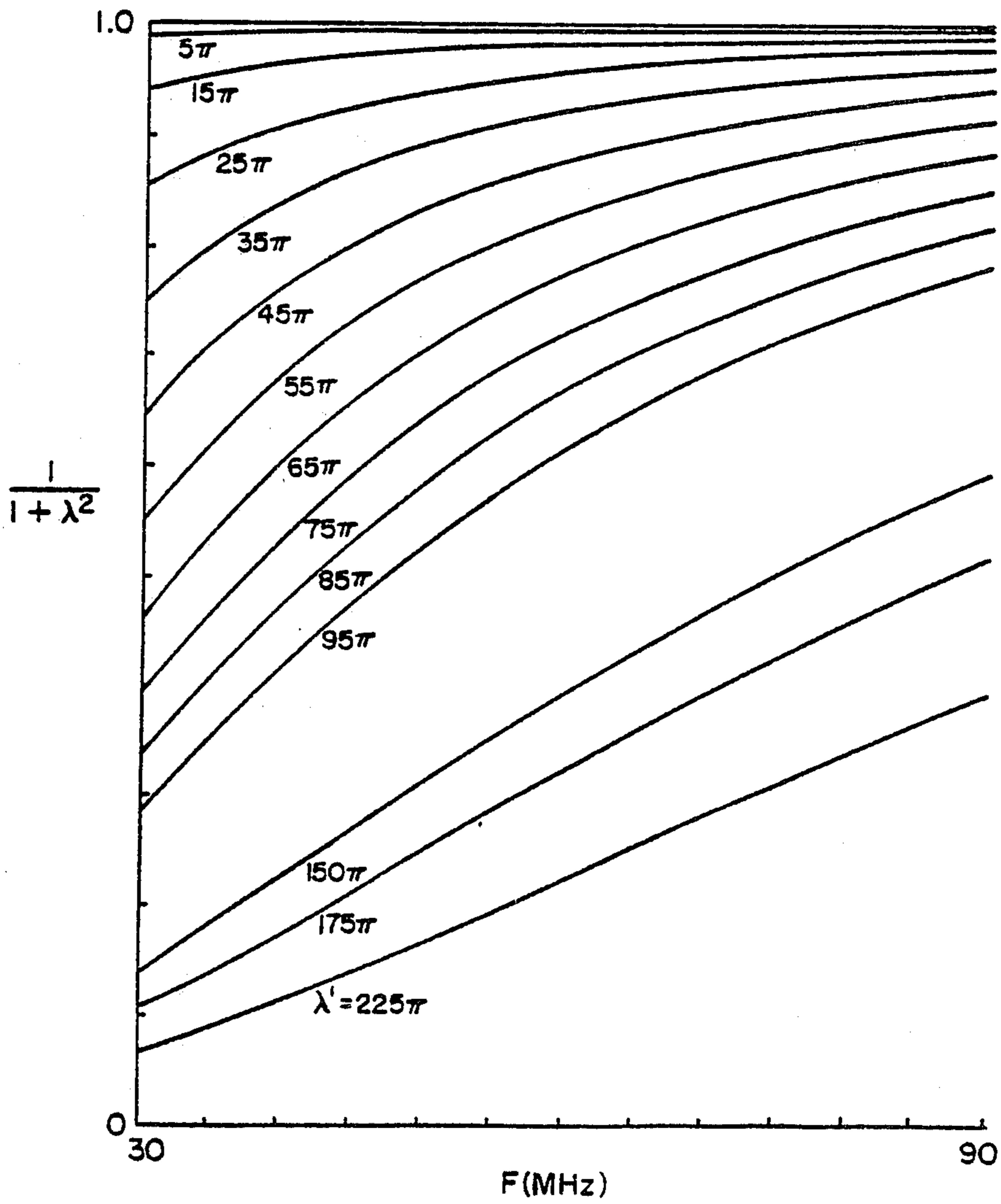
FIG. 2 SERIES RESISTANCE (R-L NETWORK)
