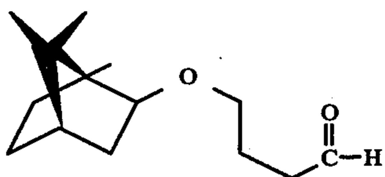
FIG. 12 is the GLC profile for fraction 6 of the distillation product of the reaction product of Example II containing the compound having the structure:
