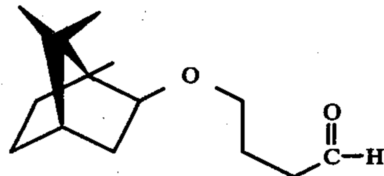
FIG. 10 is the GLC profile for fraction 4 of the distillation product of the reaction product of Example II containing the compound having the structure:
