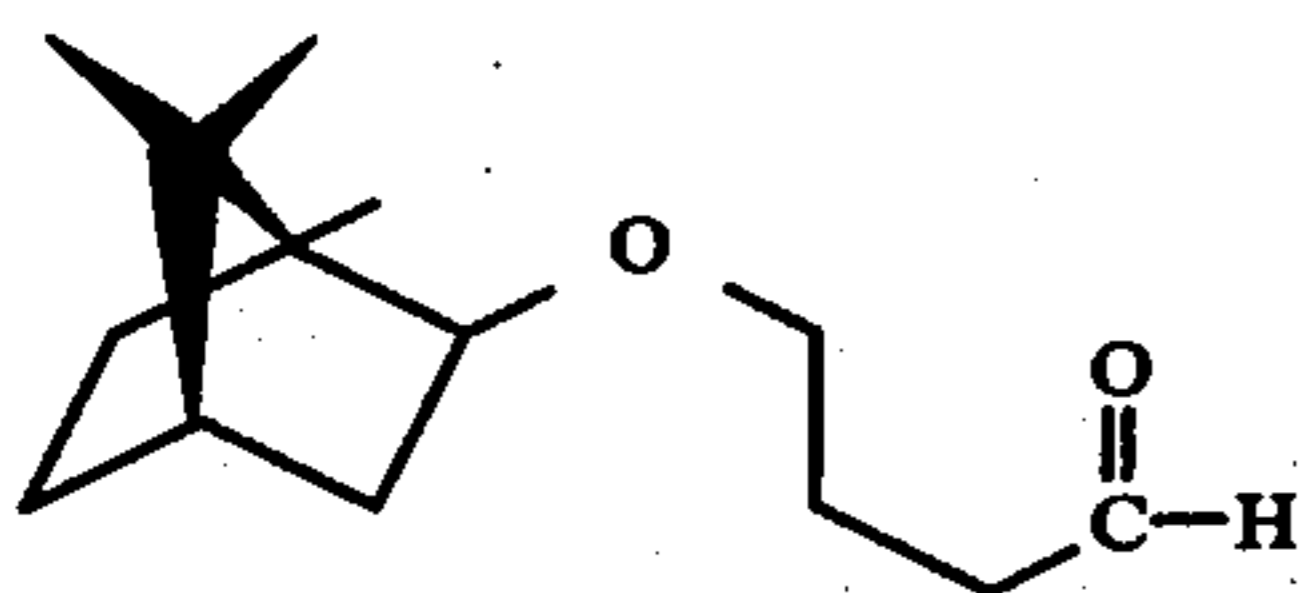
FIG. 7 is the GLC profile for fraction 1 of the distillation product of the reaction product of Example II containing the compound having the structure:
