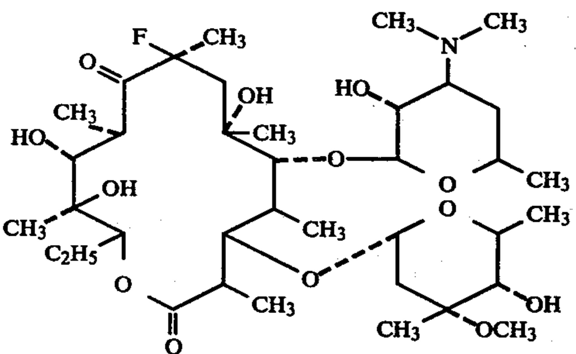
or the pharmaceutically acceptable salts thereof. 10. (8S)-8-fluoroerythromycin B, having the formula
