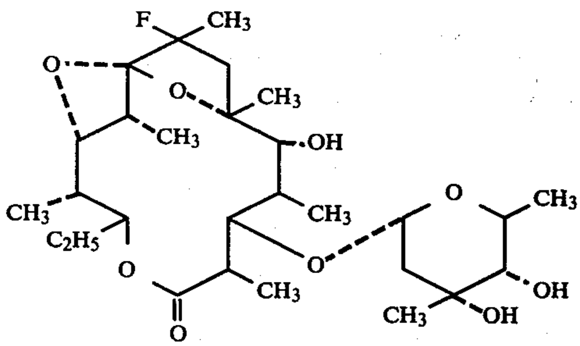
8. 3-O-mycarosyl-8,9-anhydroerythronolide B-6,9-hemiacetal having the formula:
