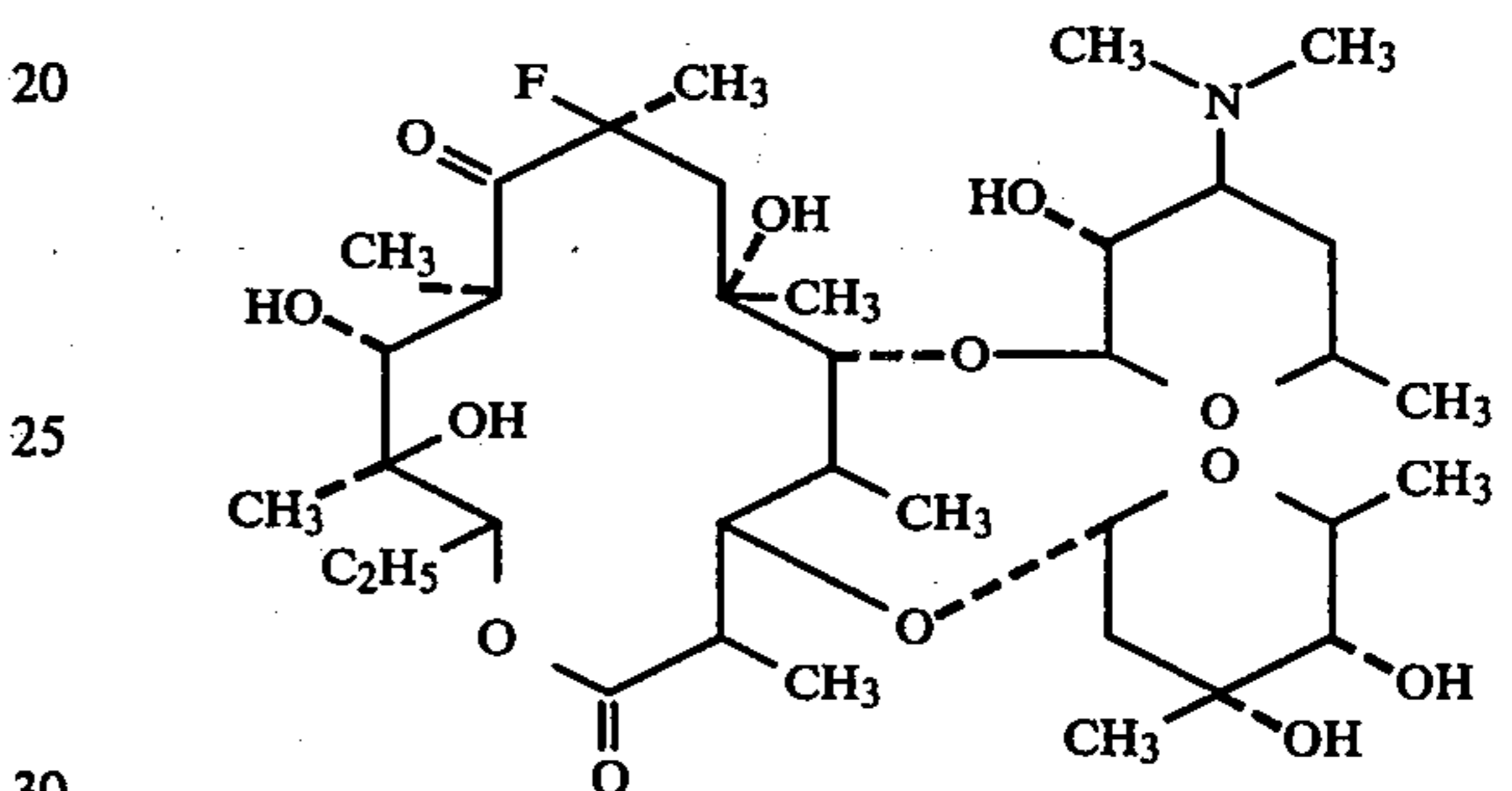
12. (8S)-8-fluoroerythromycin D, having the formula
