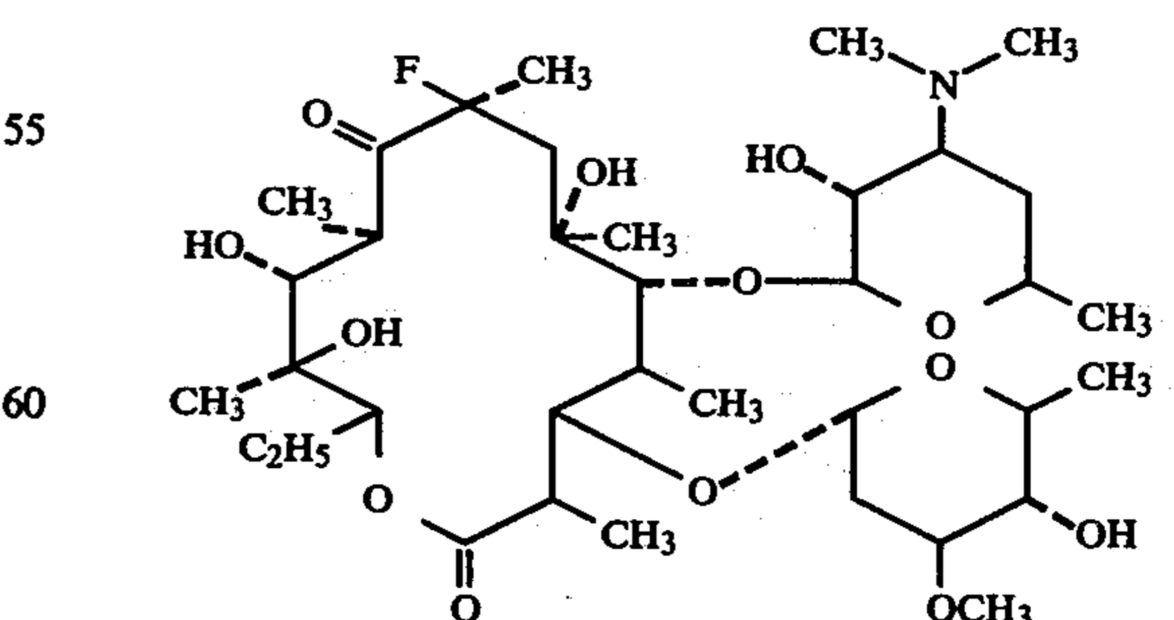
14. 3-O-oleandrosyl-5-O-desosaminyl-(8S)-8-fluoroerythronolide B, having the formula
