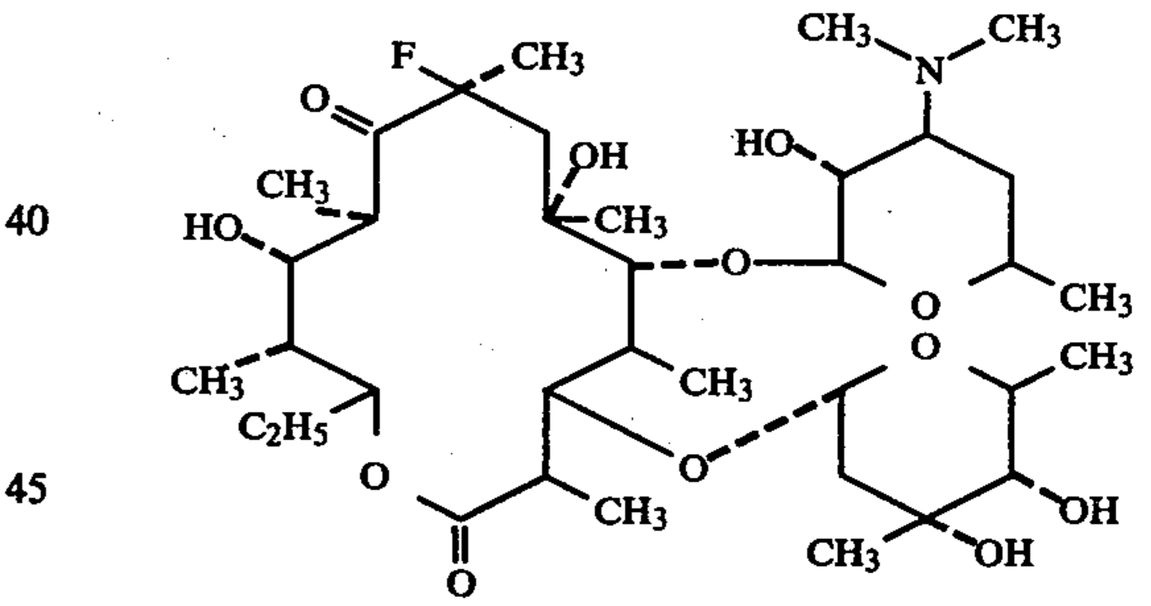
13. 3-O-oleandrosyl-5-O-desosaminyl-(8S)-8-fluoroerythronolide A, having the formula
