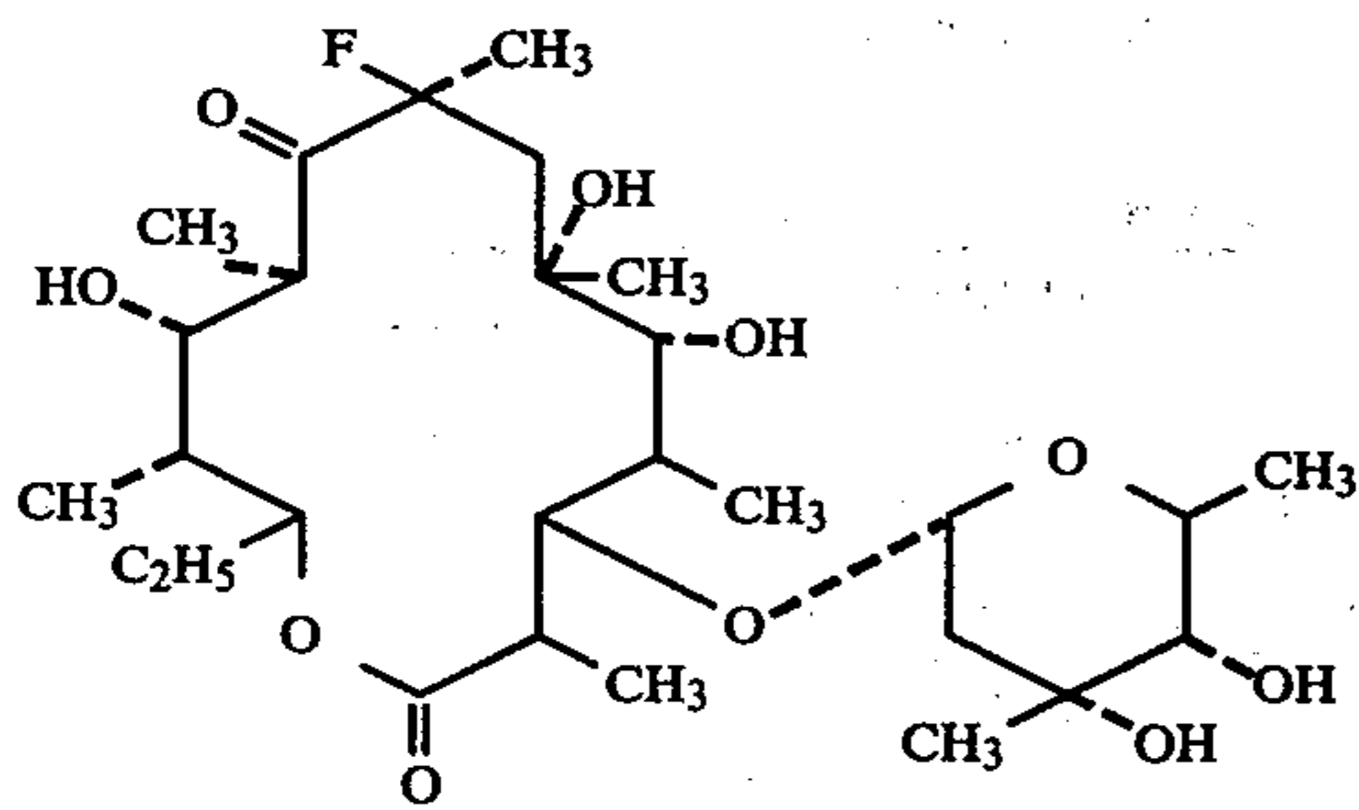
7. 3-O-mycarosyl-(8S)-8-fluoroerythronolide 6,9;9,11-acetal having the formula:
