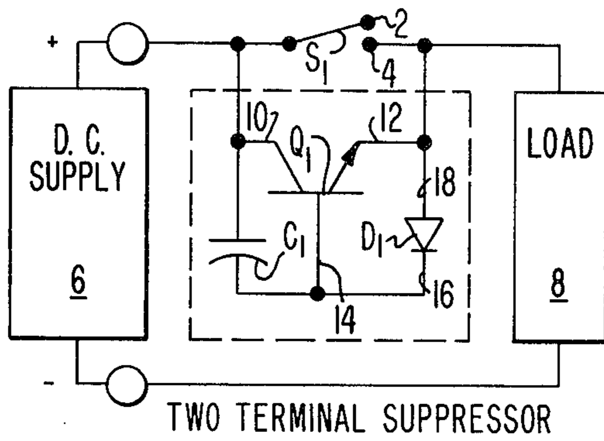
FIG. 1 WITH NPN TRANSISTOR
