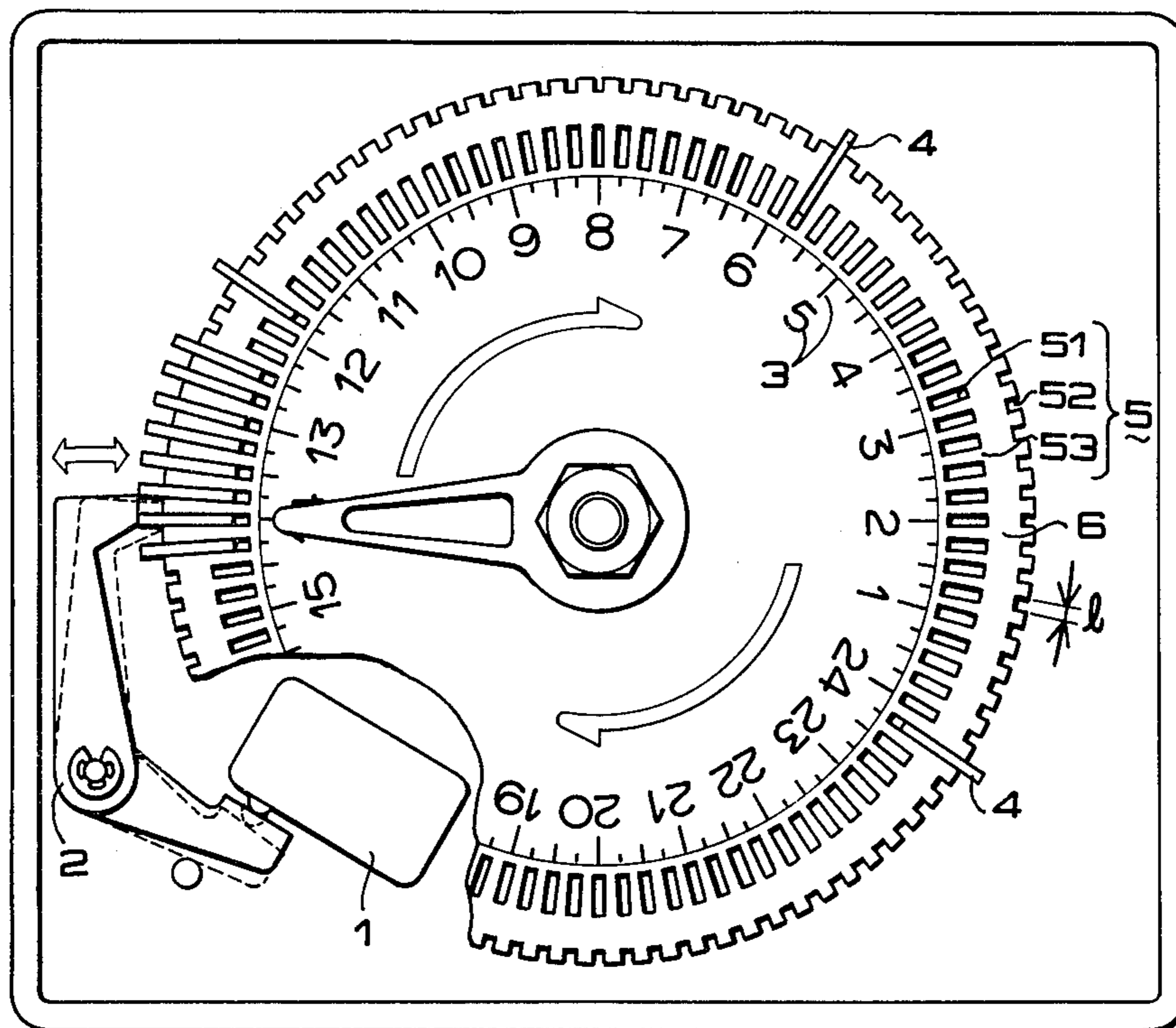
FIG. 1 (PRIOR ART)
