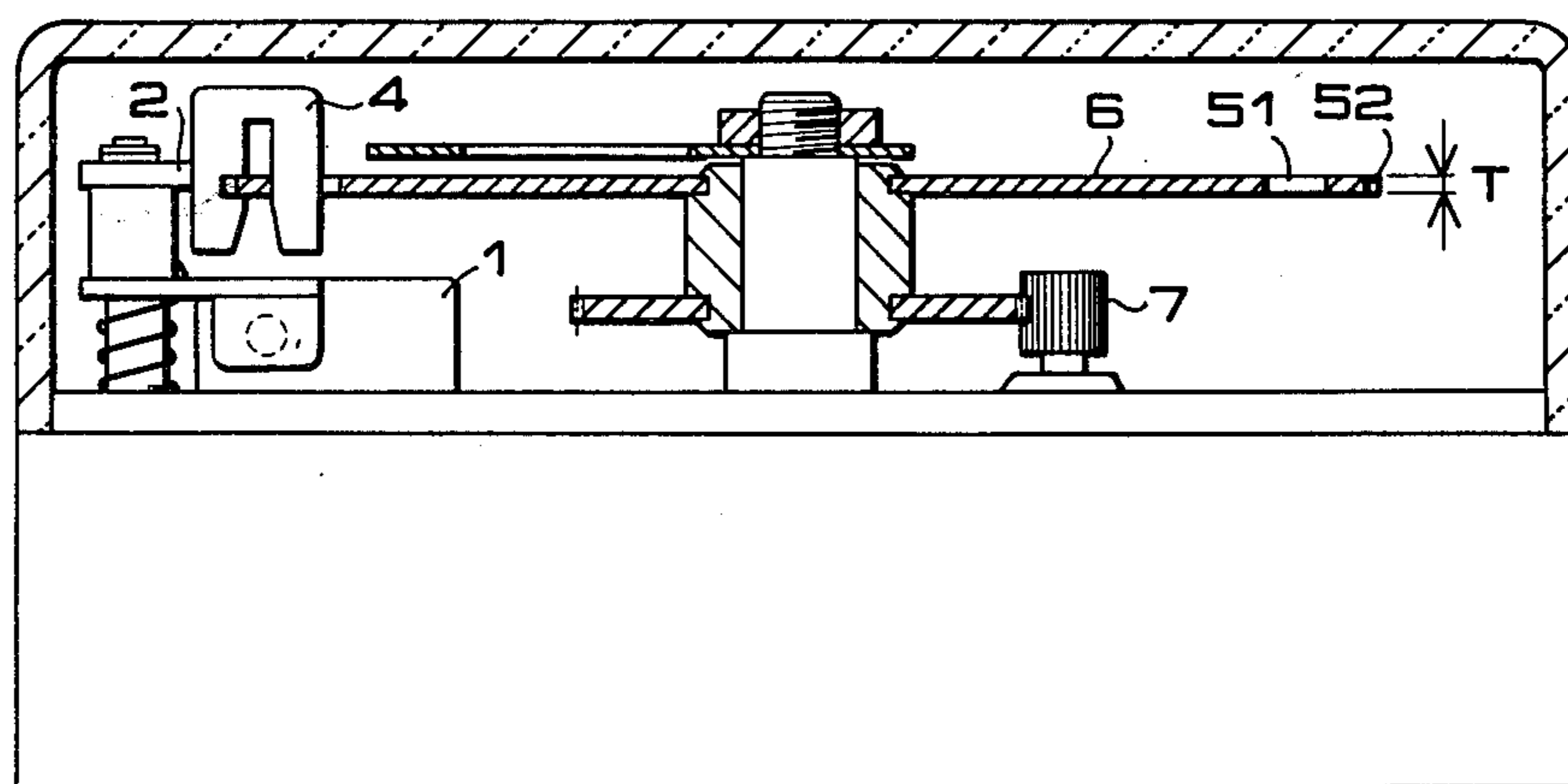
FIG. 2 (PRIOR ART)
