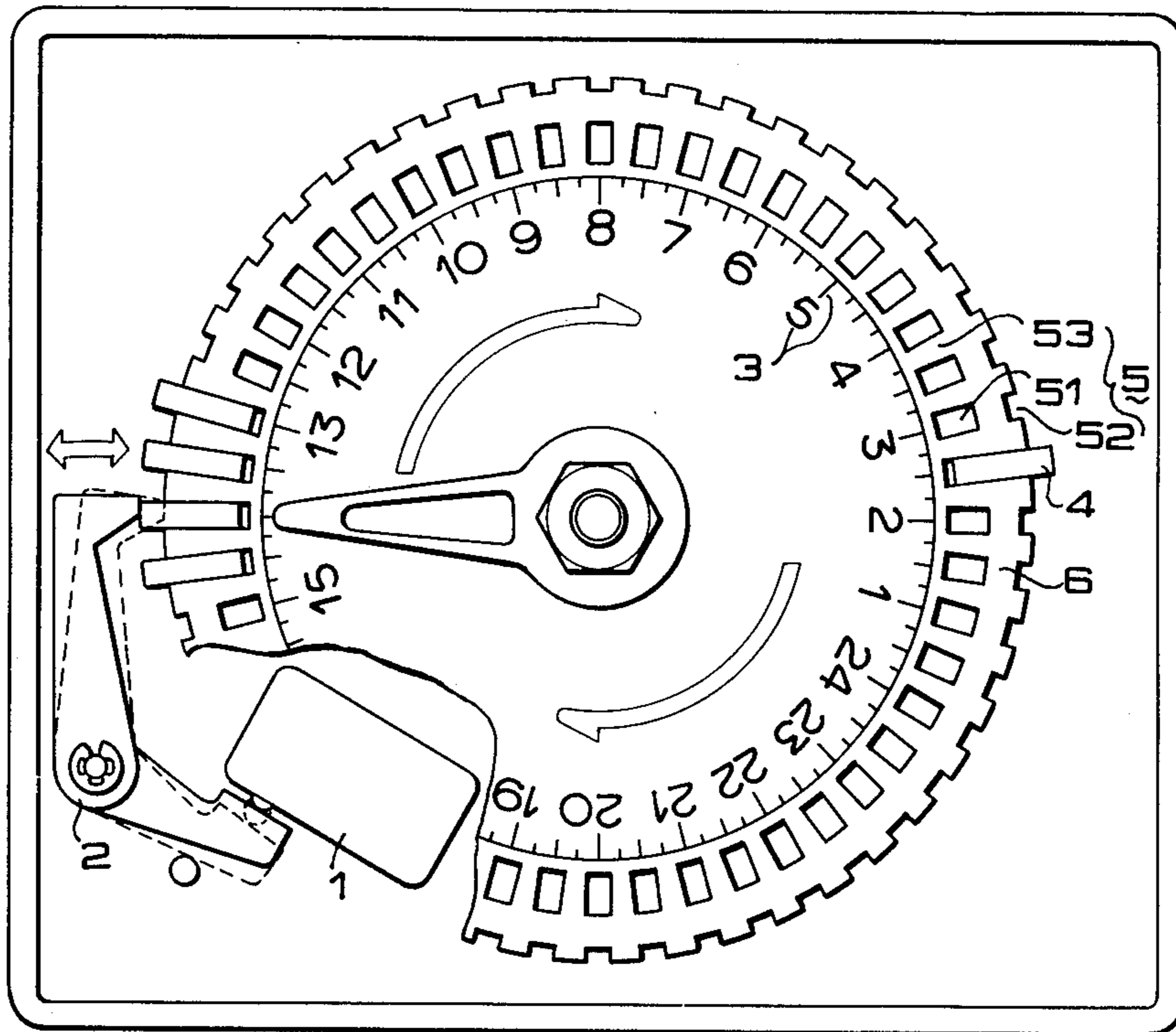
FIG. 3 (PRIOR ART)
