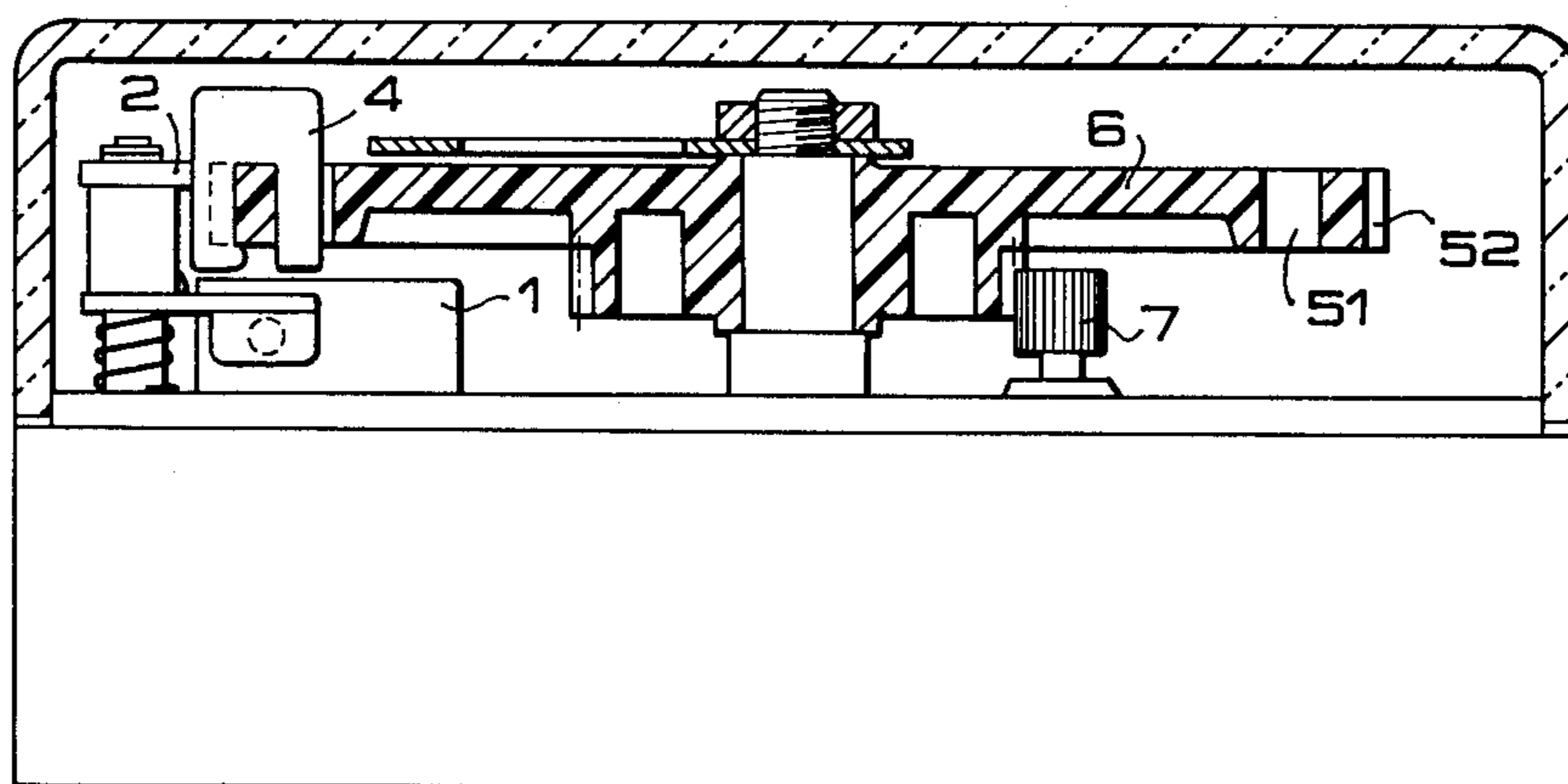
FIG. 4 (PRIOR ART)
