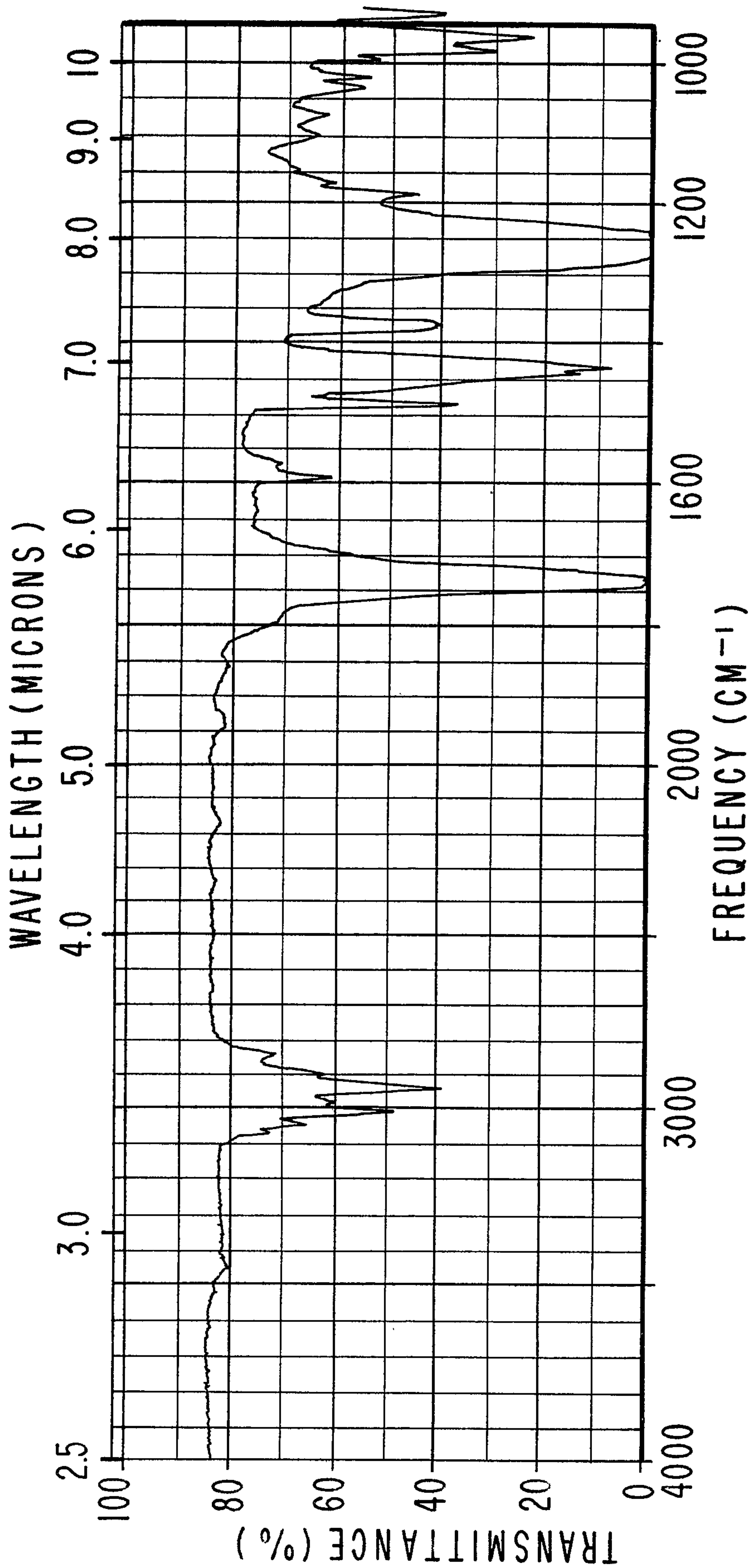
IR SPECTRUM FOR FRACTION 6 OF EXAMPLE I.
