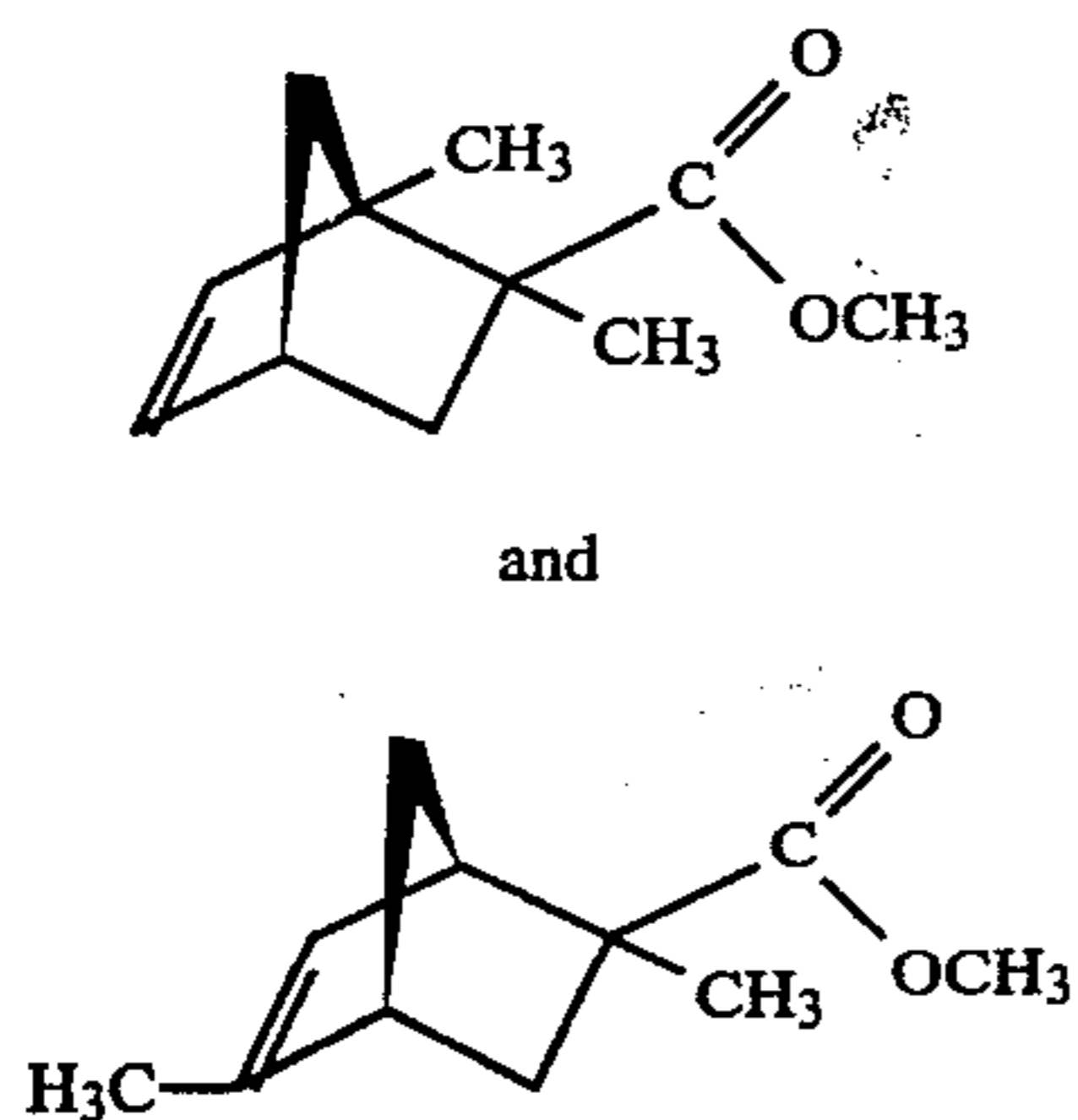
FIG. 3 is the NMR spectrum for fraction 3 of the distillation product of the reaction product of Example II containing the compounds having the structures:
