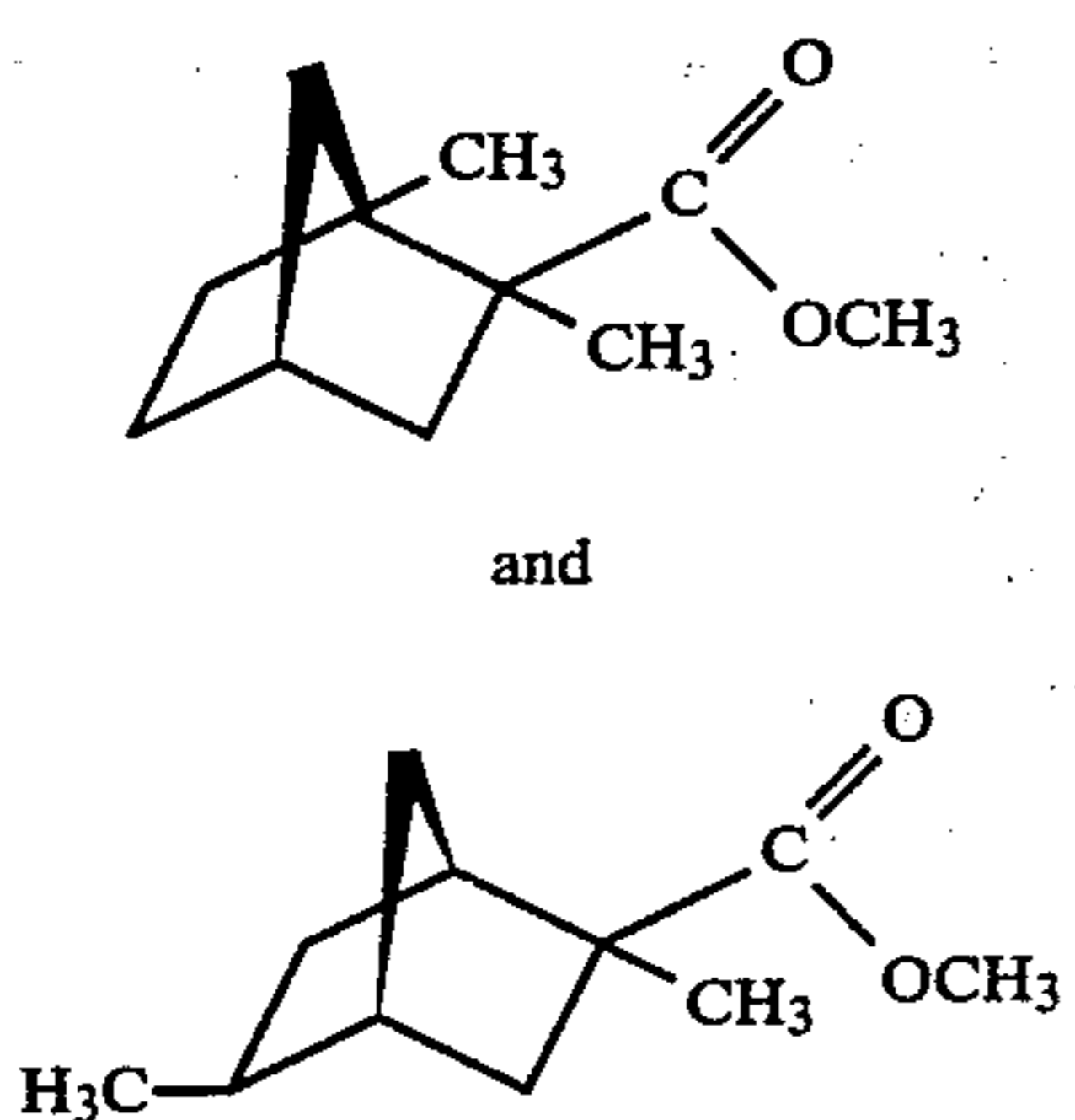
FIG. 4 is the infra-red spectrum for fraction 3 of the distillation product of the reaction product of Example II containing the compounds having the structures:
