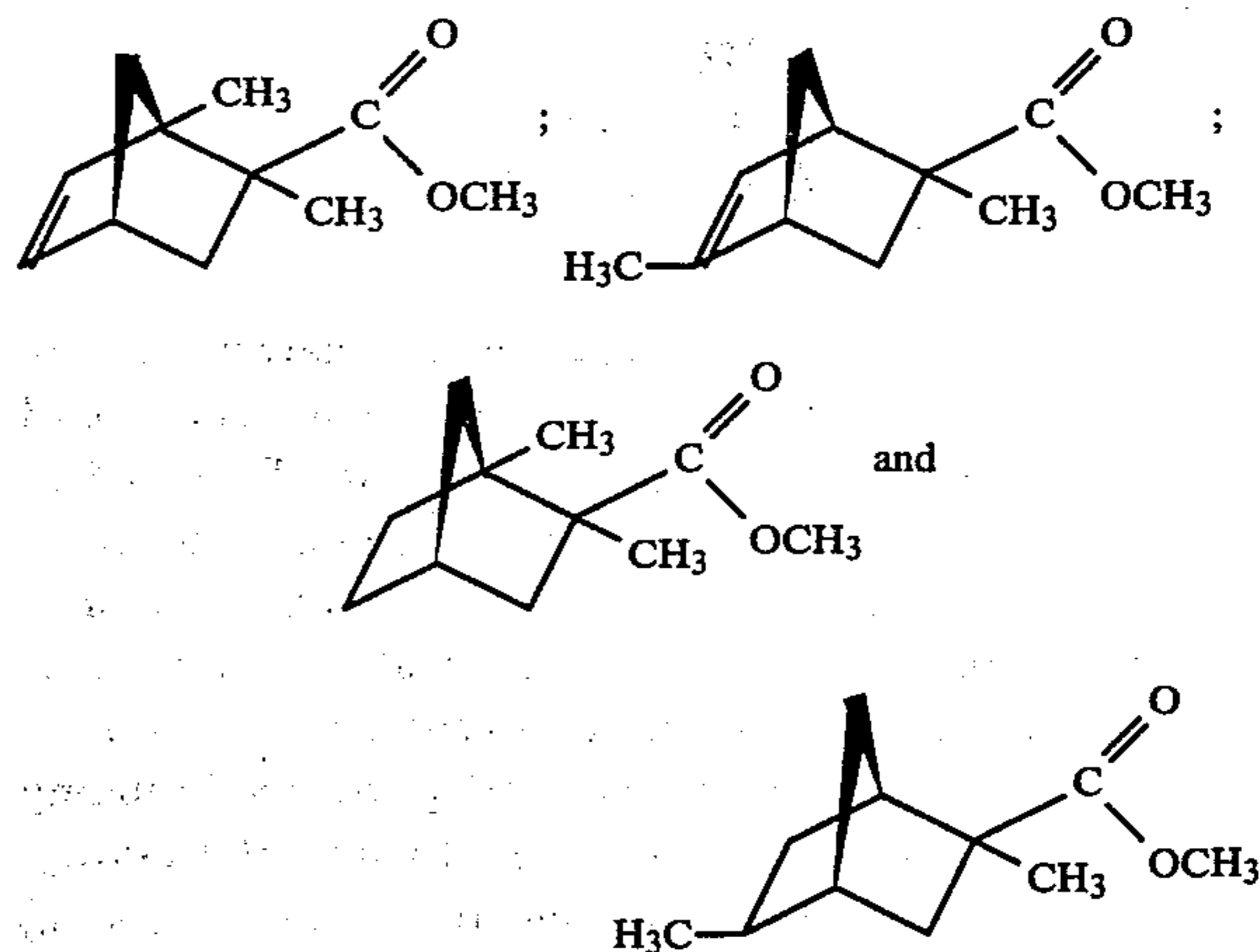
FIG. 4 is the infra-red spectrum for fraction 3 of the distillation product of the reaction product of Example II containing the compounds having the structures:
