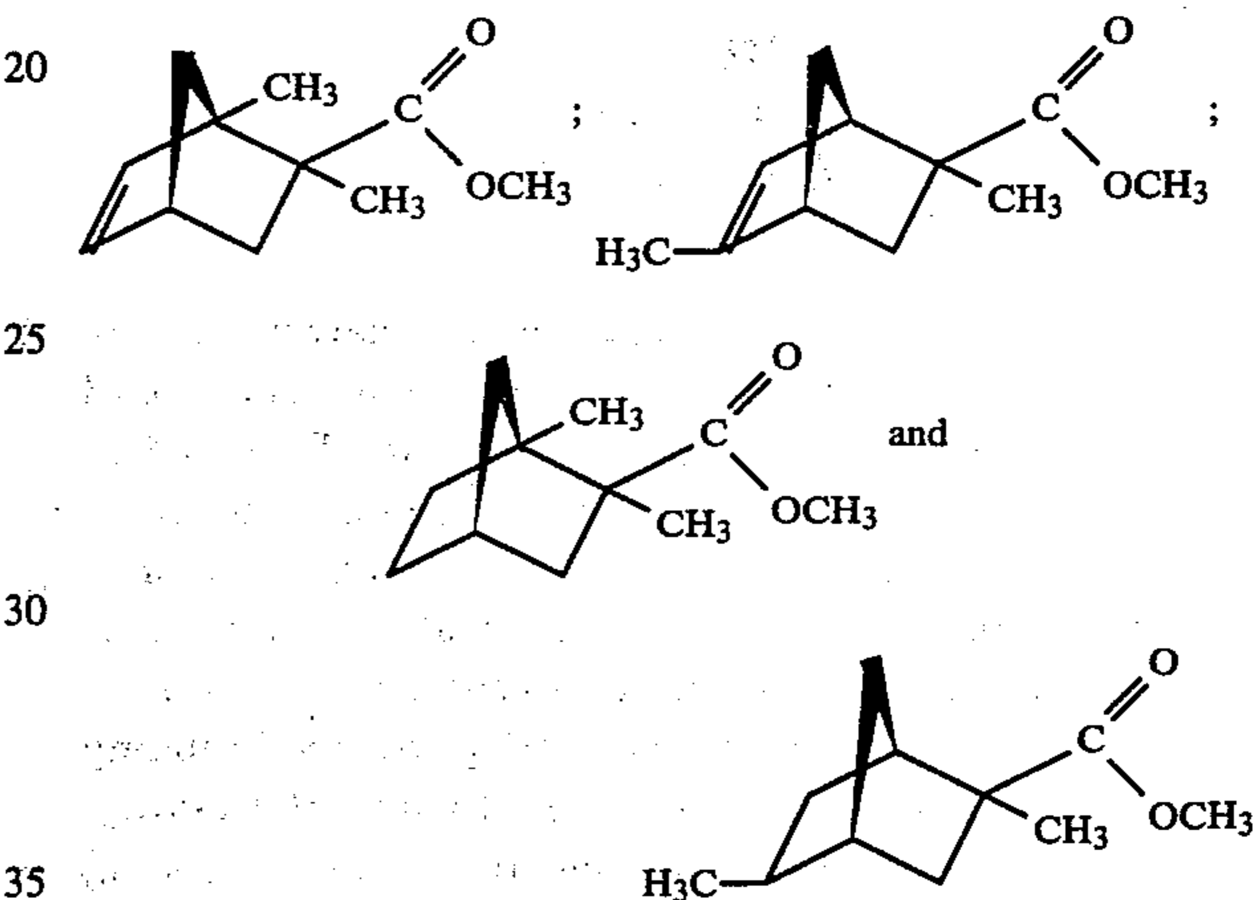
FIG. 4 is the infra-red spectrum for fraction 3 of the distillation product of the reaction product of Example II containing the compounds having the structures:
