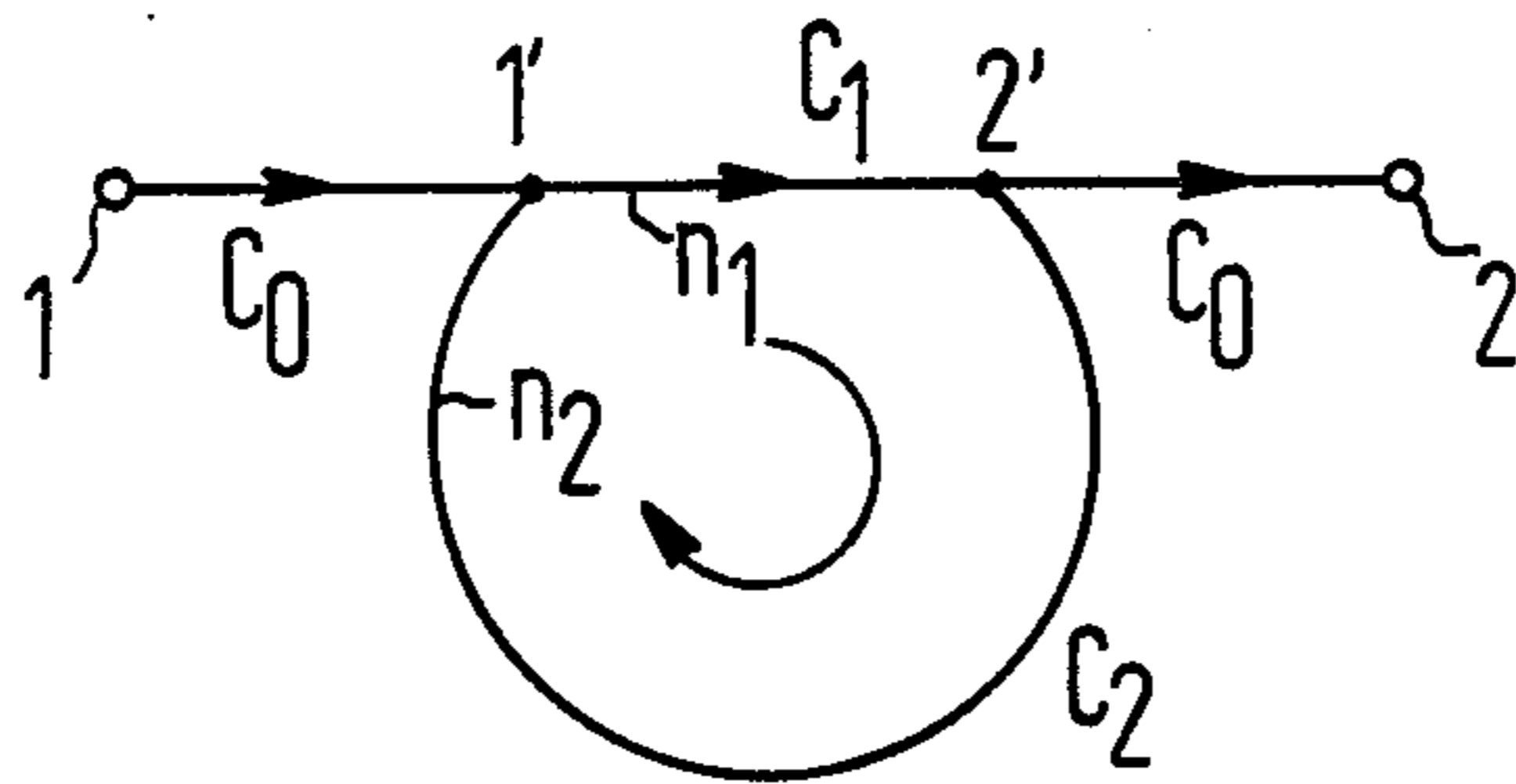
FIG 1 (PRIOR ART)
