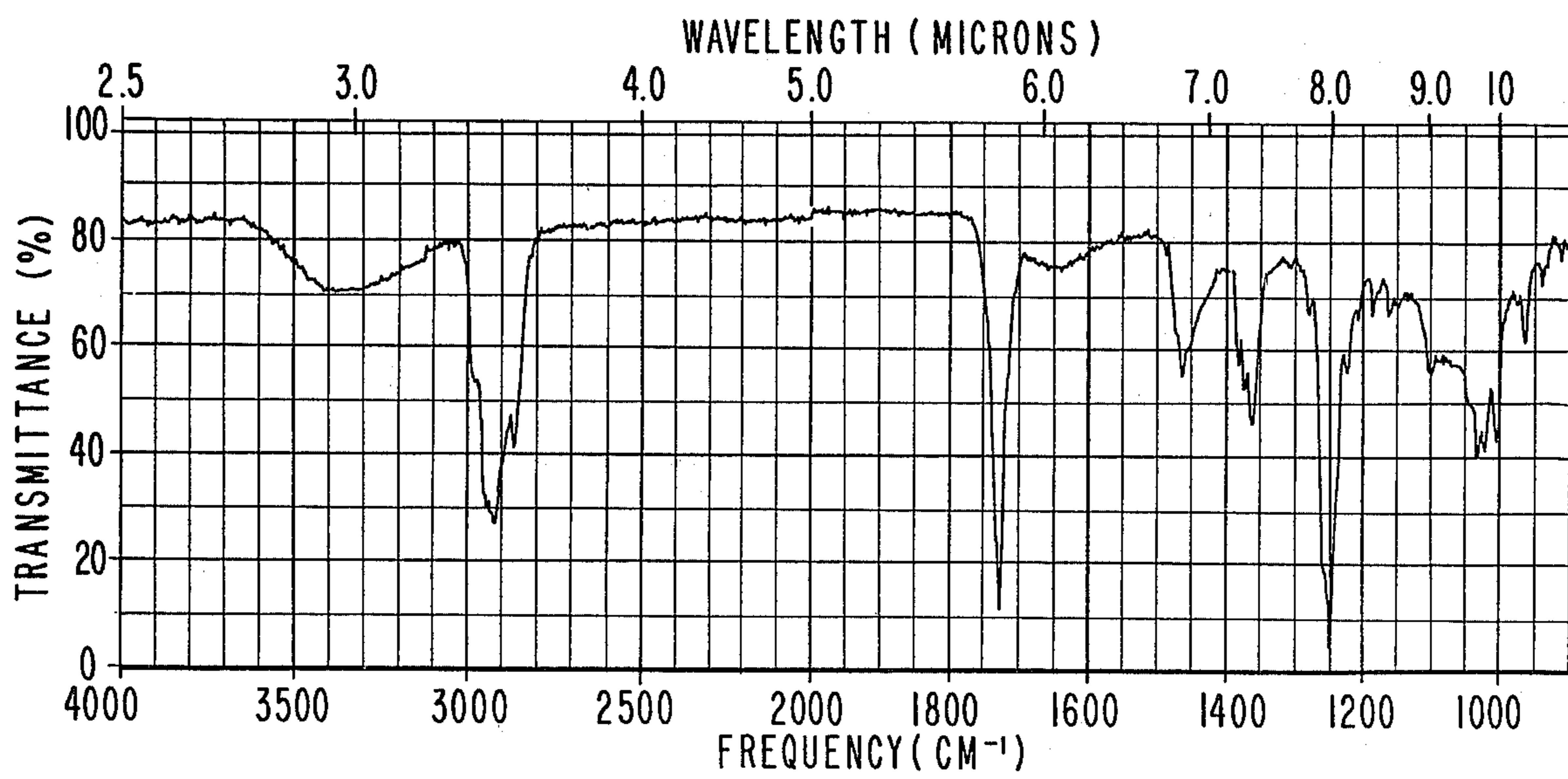
IR SPECTRUM FOR EXAMPLE III.
