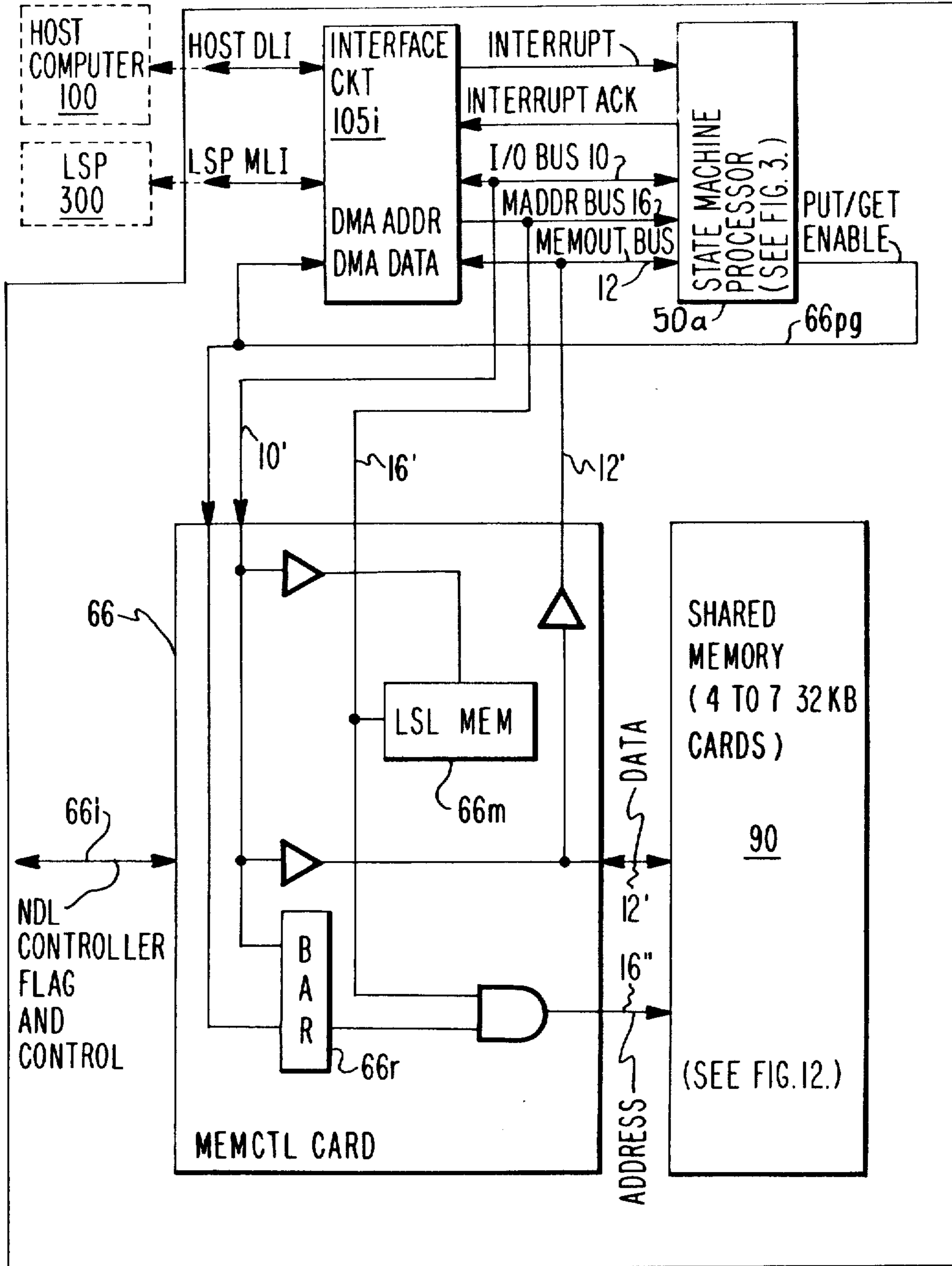
FIG. 7. EXTERNAL BUS LOGIC BLOCK DIAGRAM.
