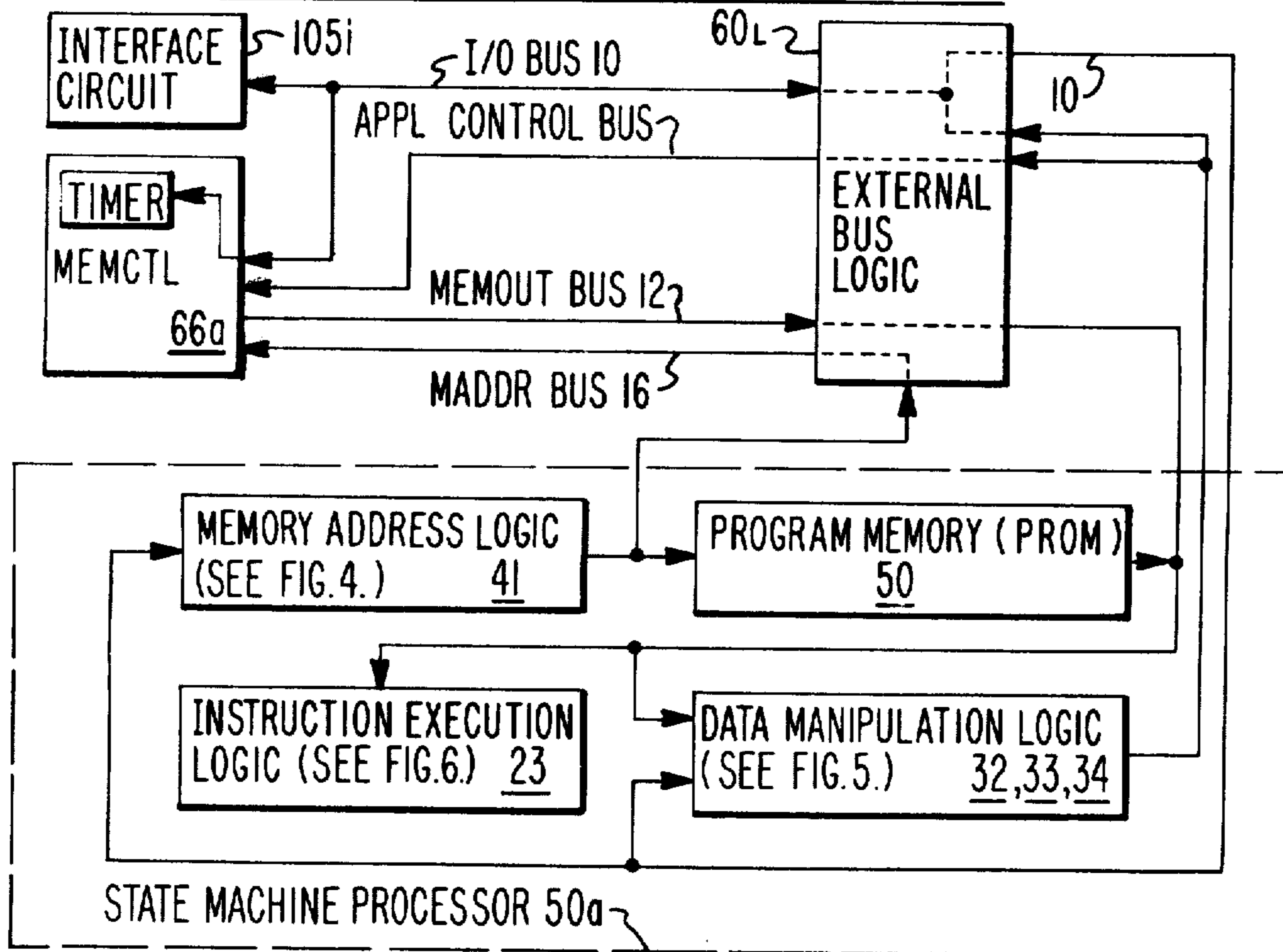
FIG. 3. STATE MACHINE PROCESSOR AND ADJACENT UNITS.
