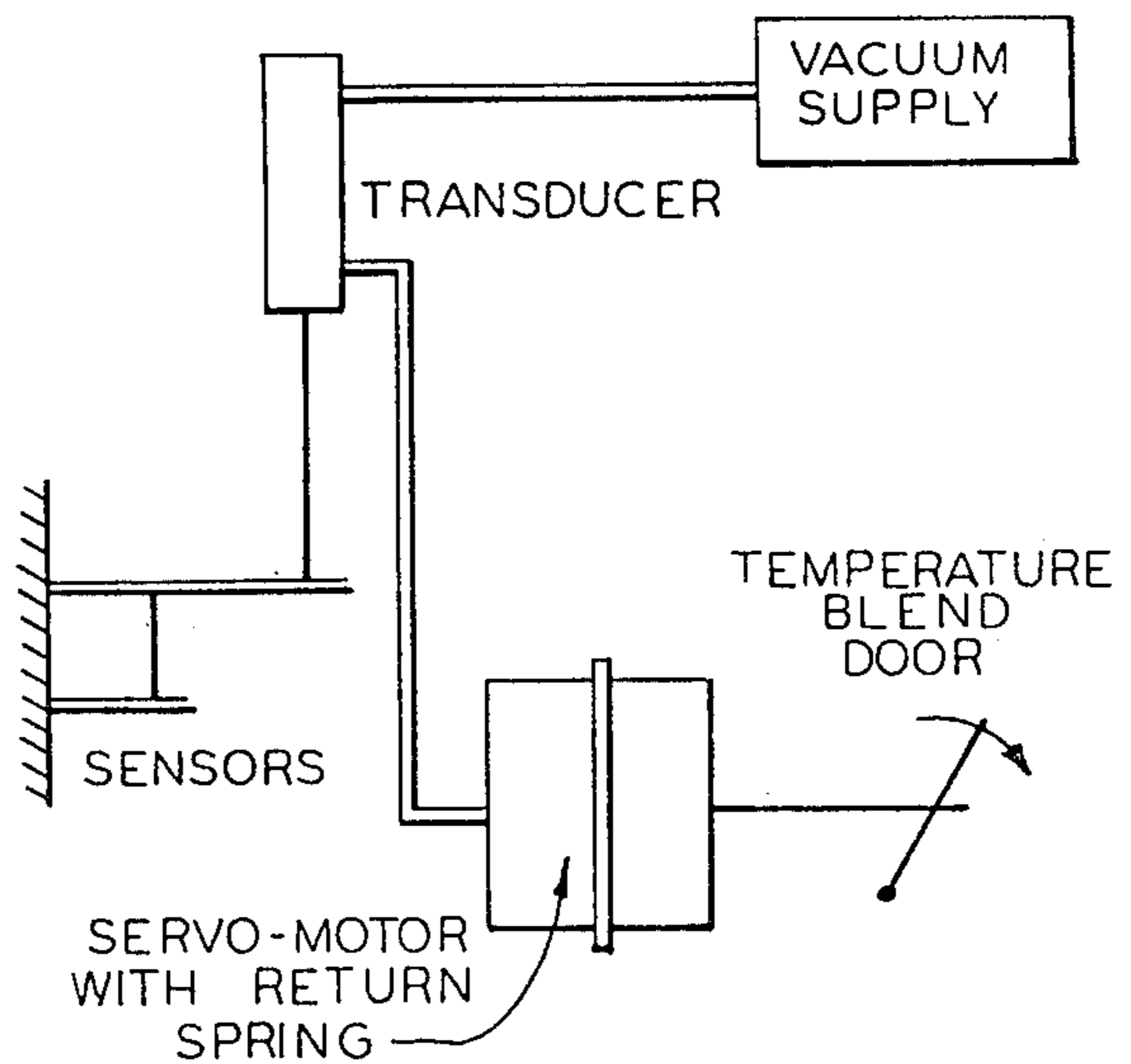
FIG. 9 Prior Art
