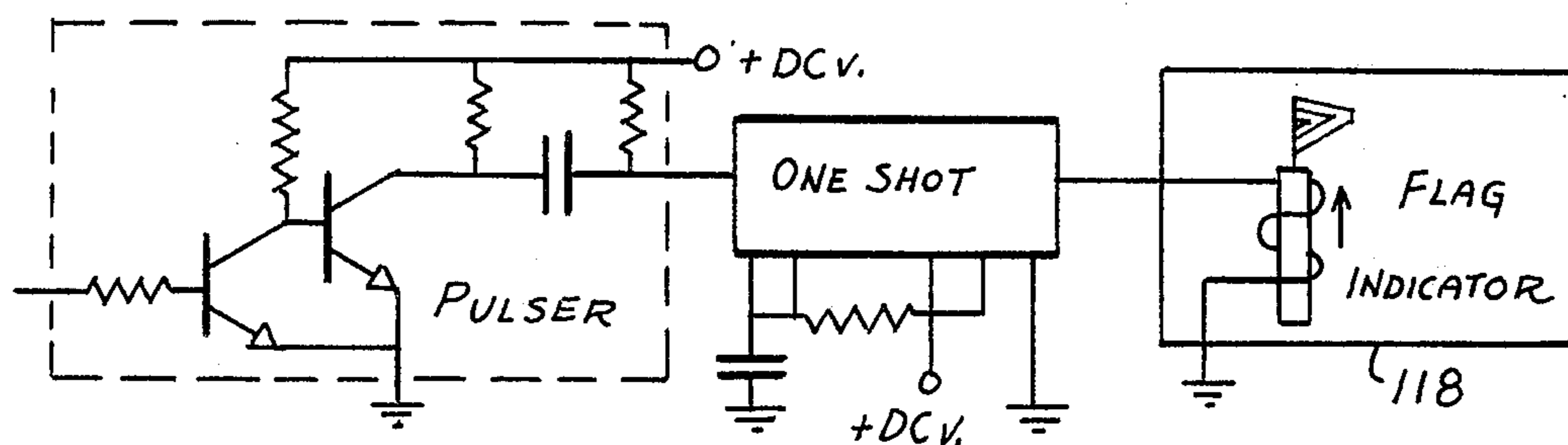
FLAG INDICATOR CIRCUIT
