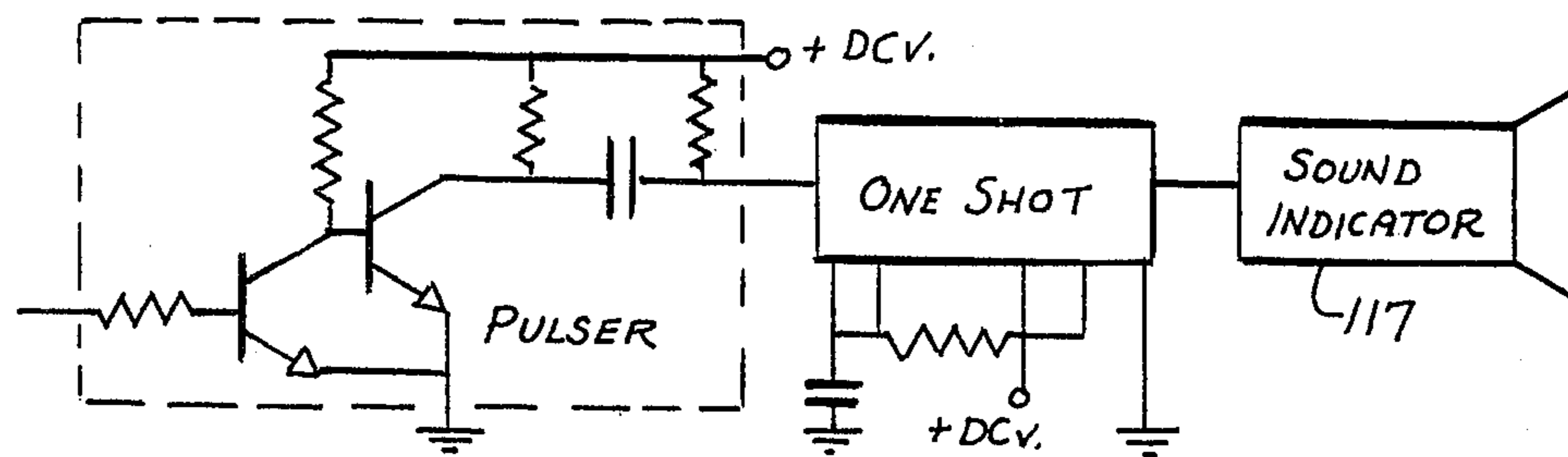
SOUND INDICATOR CIRCUIT
