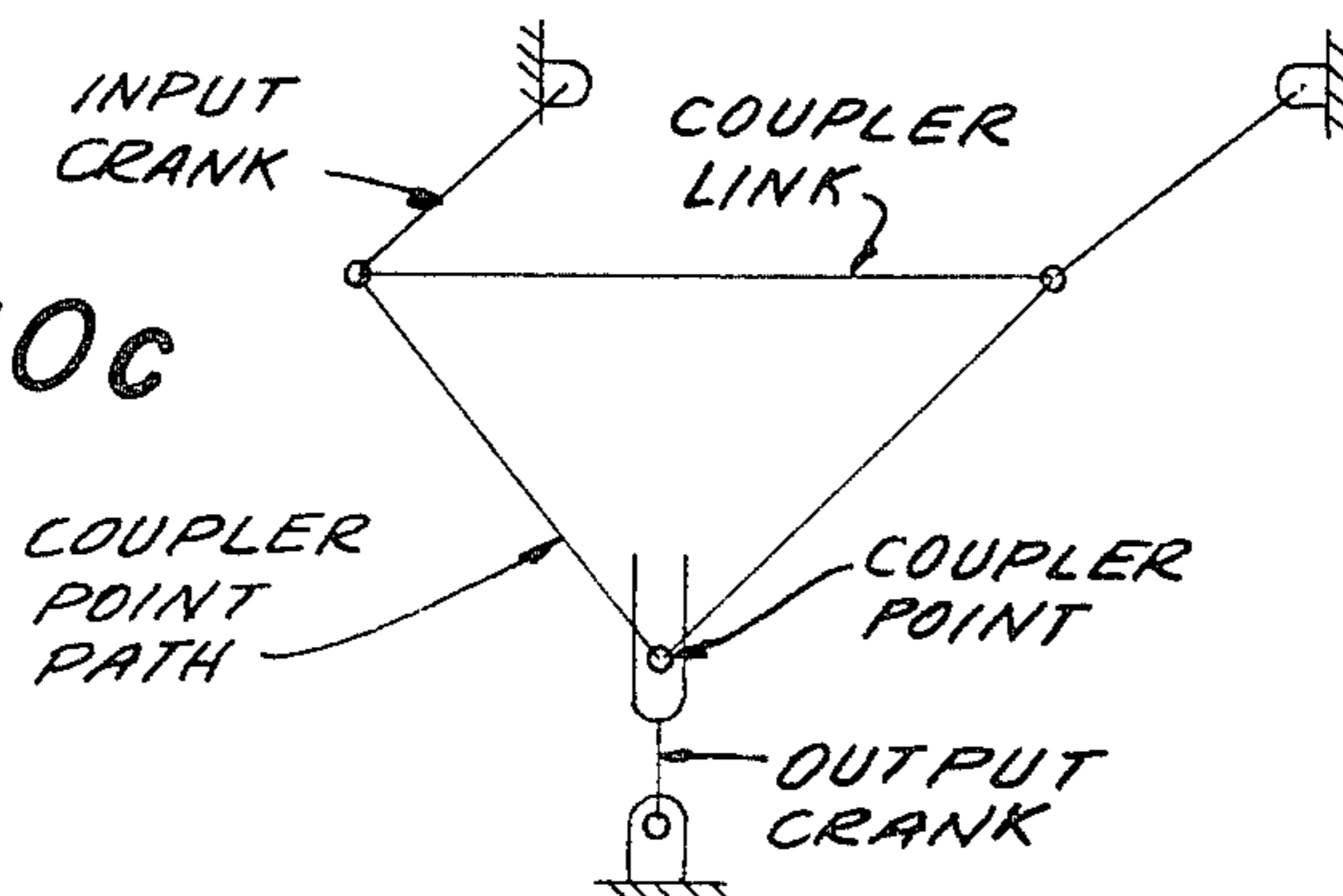
6-BAR CONTROL MECHANISM
