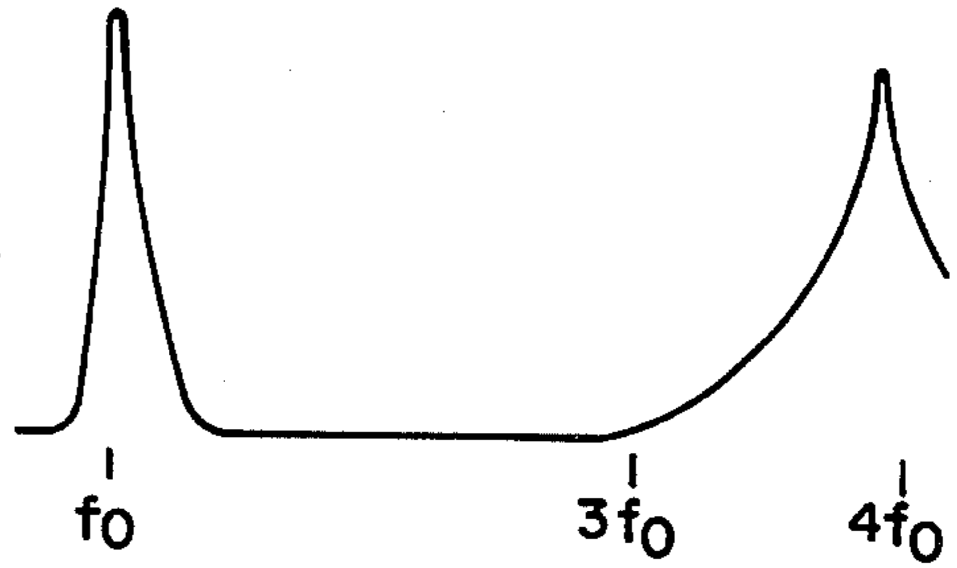
FILTER WITH RE-RESONANCE RATIO n=4
