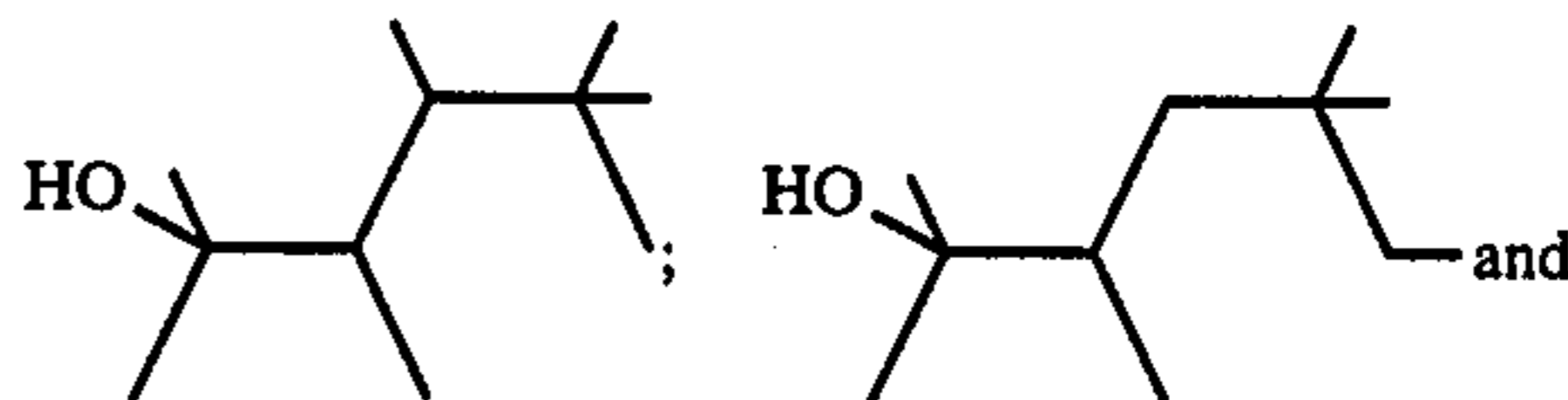
FIG. 11 is the NMR spectrum for distillation fraction 10 of the foregoing distillation containing the compounds having the structures:
