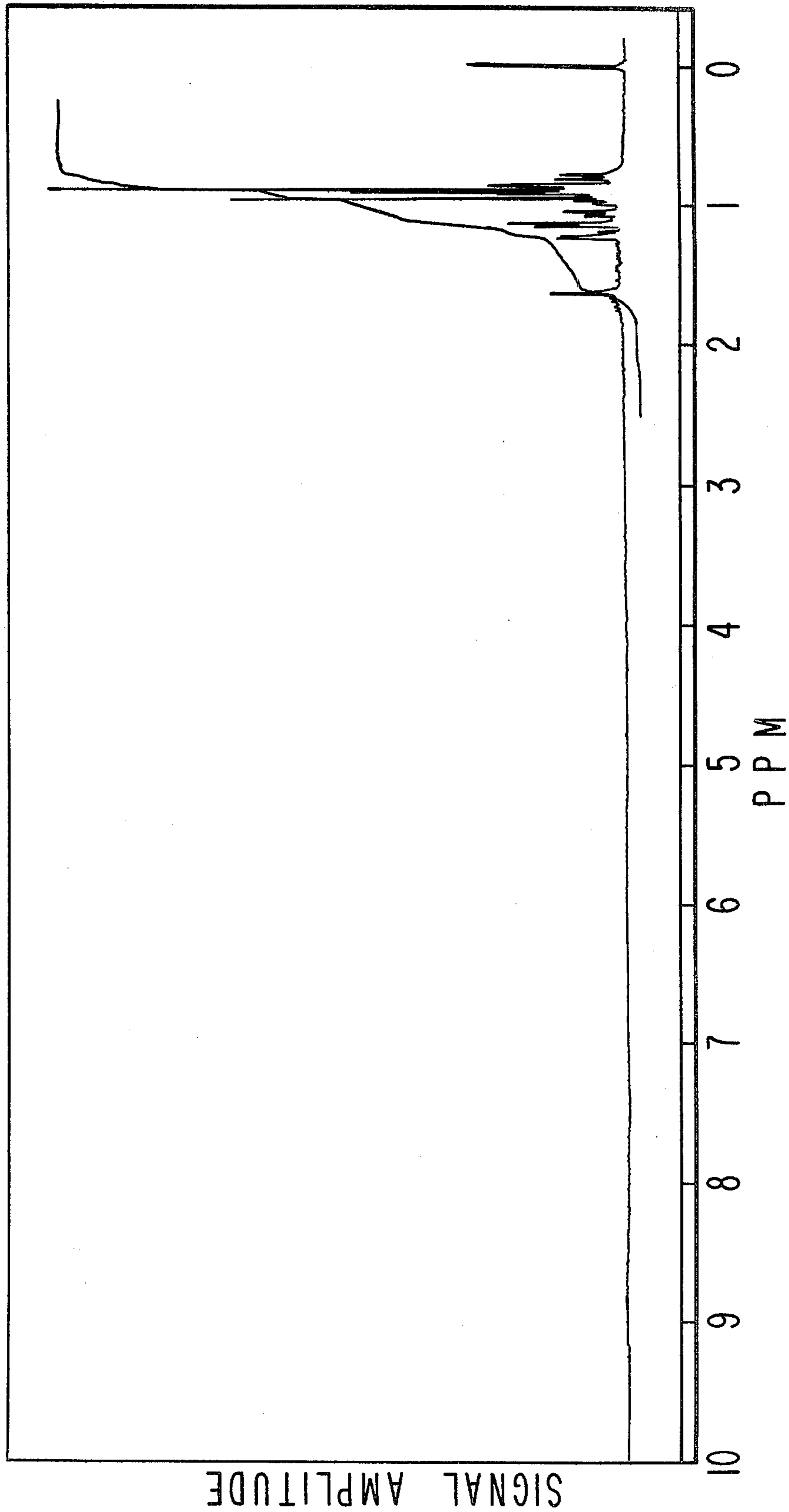
NMR SPECTRUM FOR FRACTION 10 OF EXAMPLE II.
