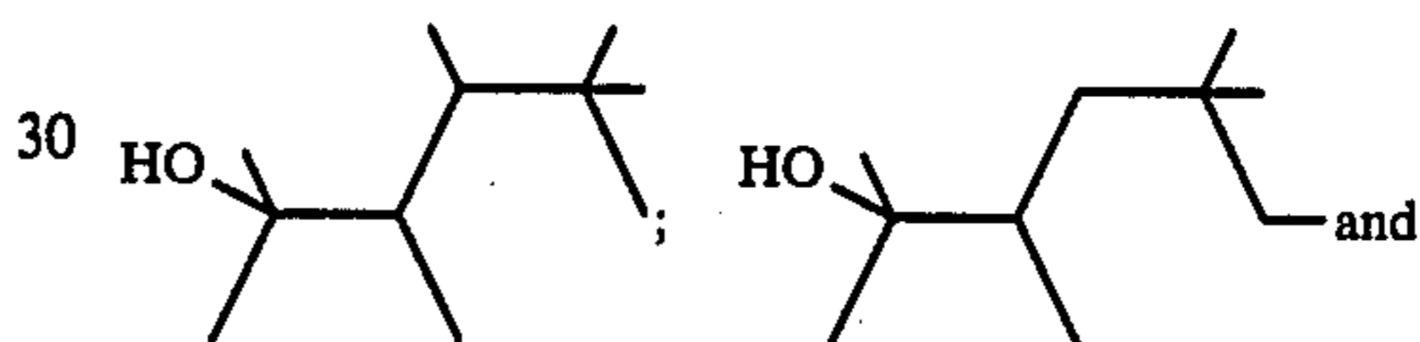
FIG. 12 is the infra-red spectrum for fraction 10 of the foregoing distillation containing the compounds having the structures:
