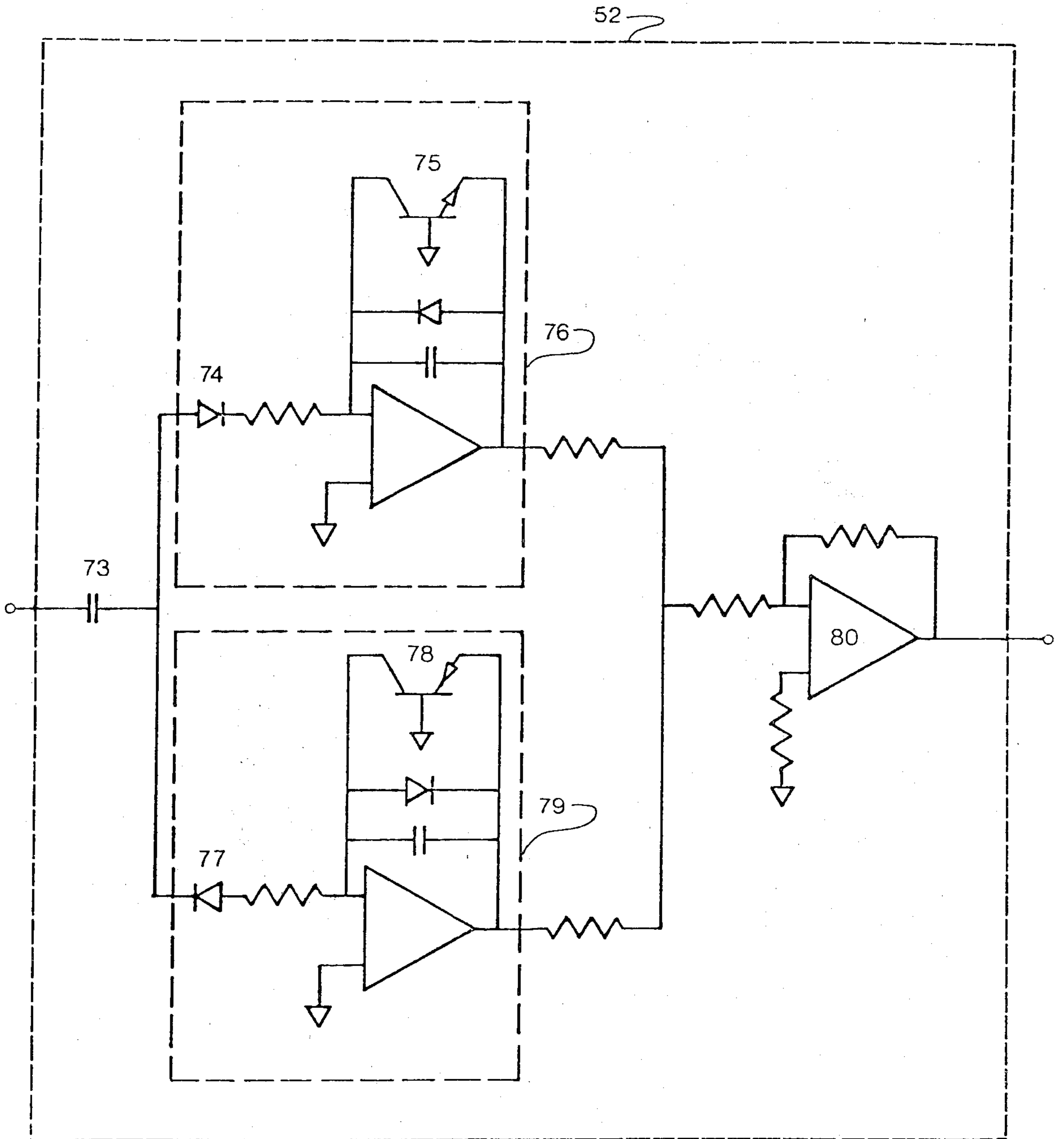
NON-LINEAR AMP.
