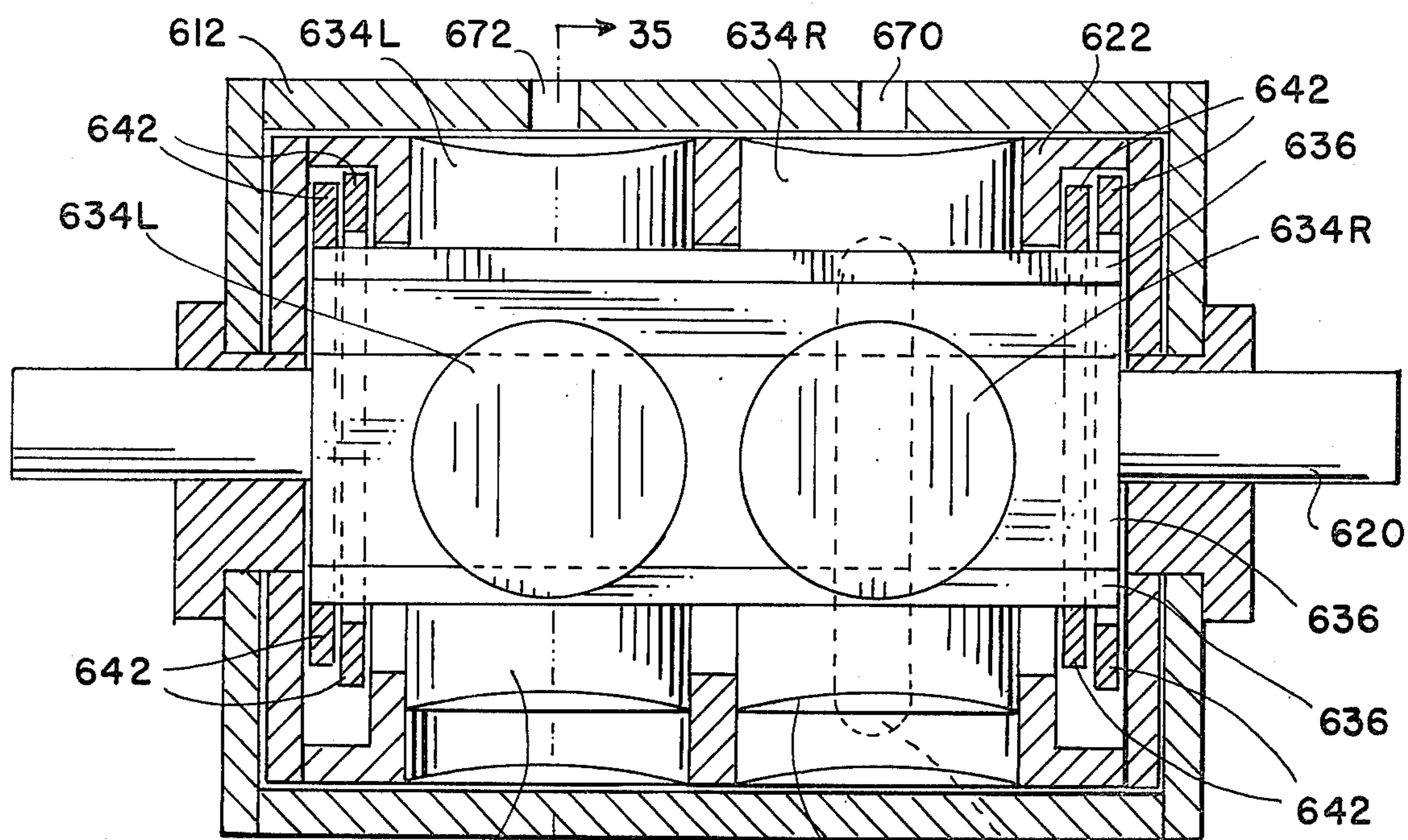
FIG. 34 SEC. 34-34
