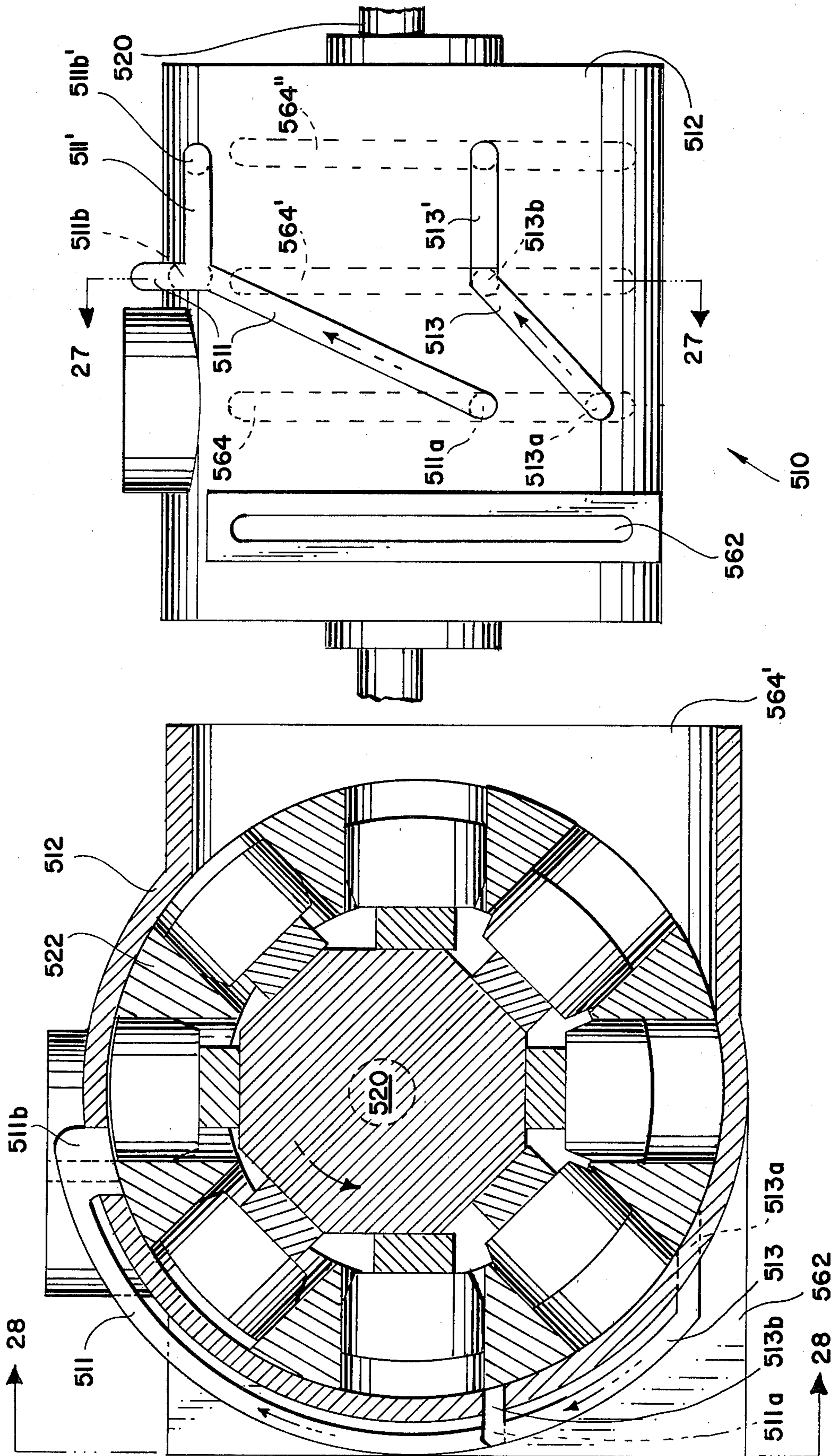
FIG. 27 SEC. 27-27
