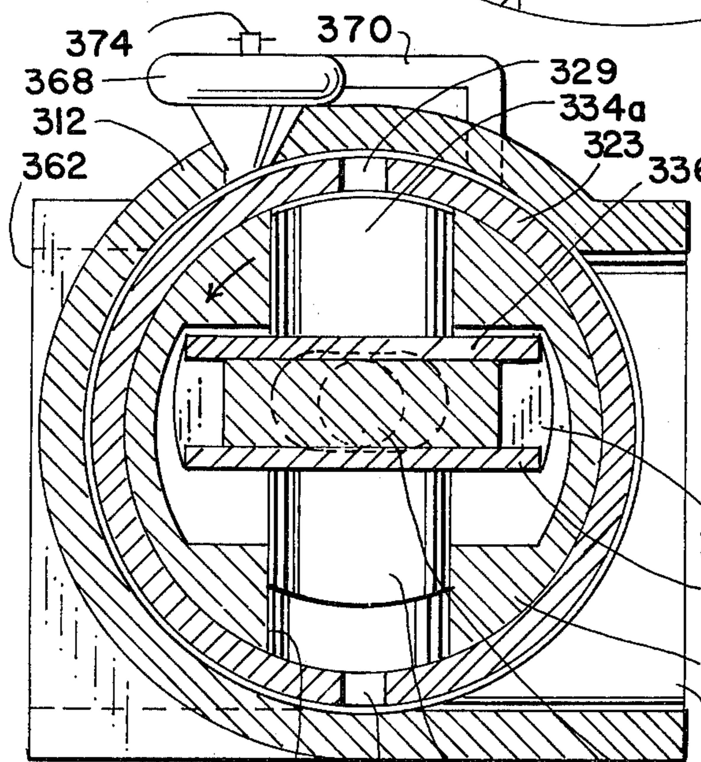
FIG. 24 SEC. 24-24
