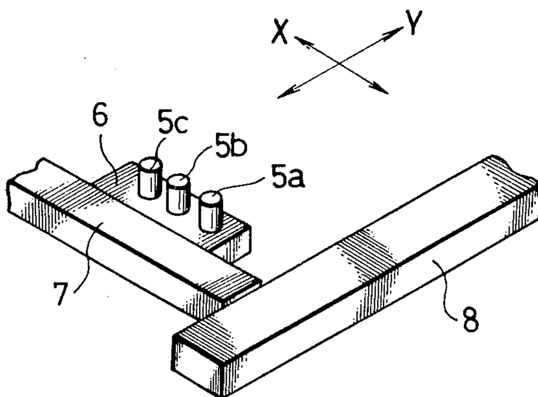
Fig.2 PRIOR ART
