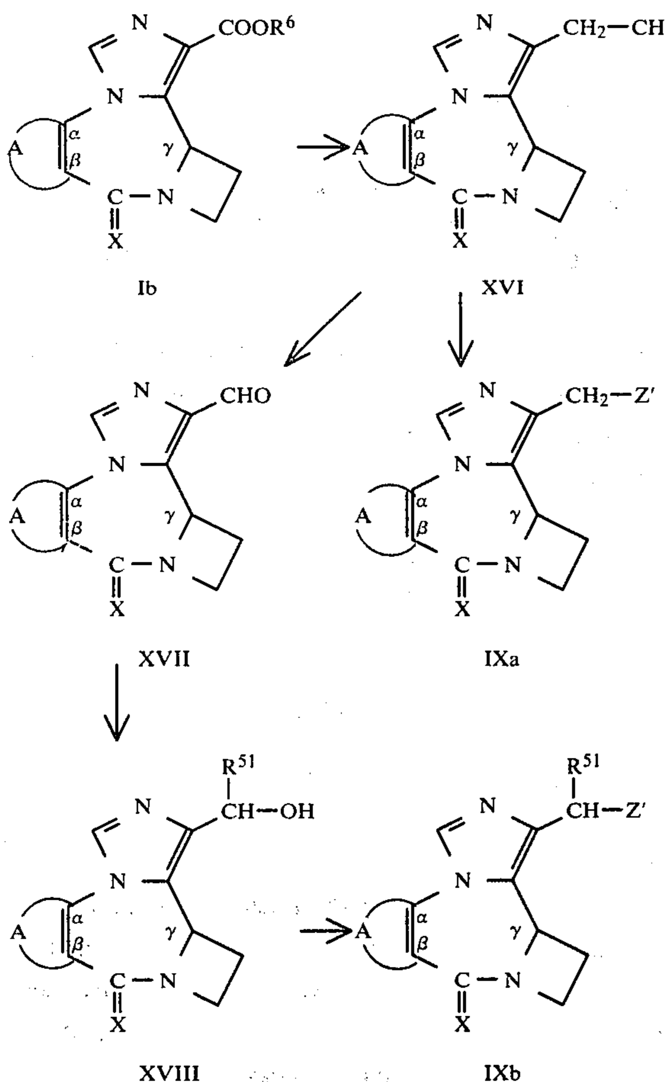
Formula Scheme 2
