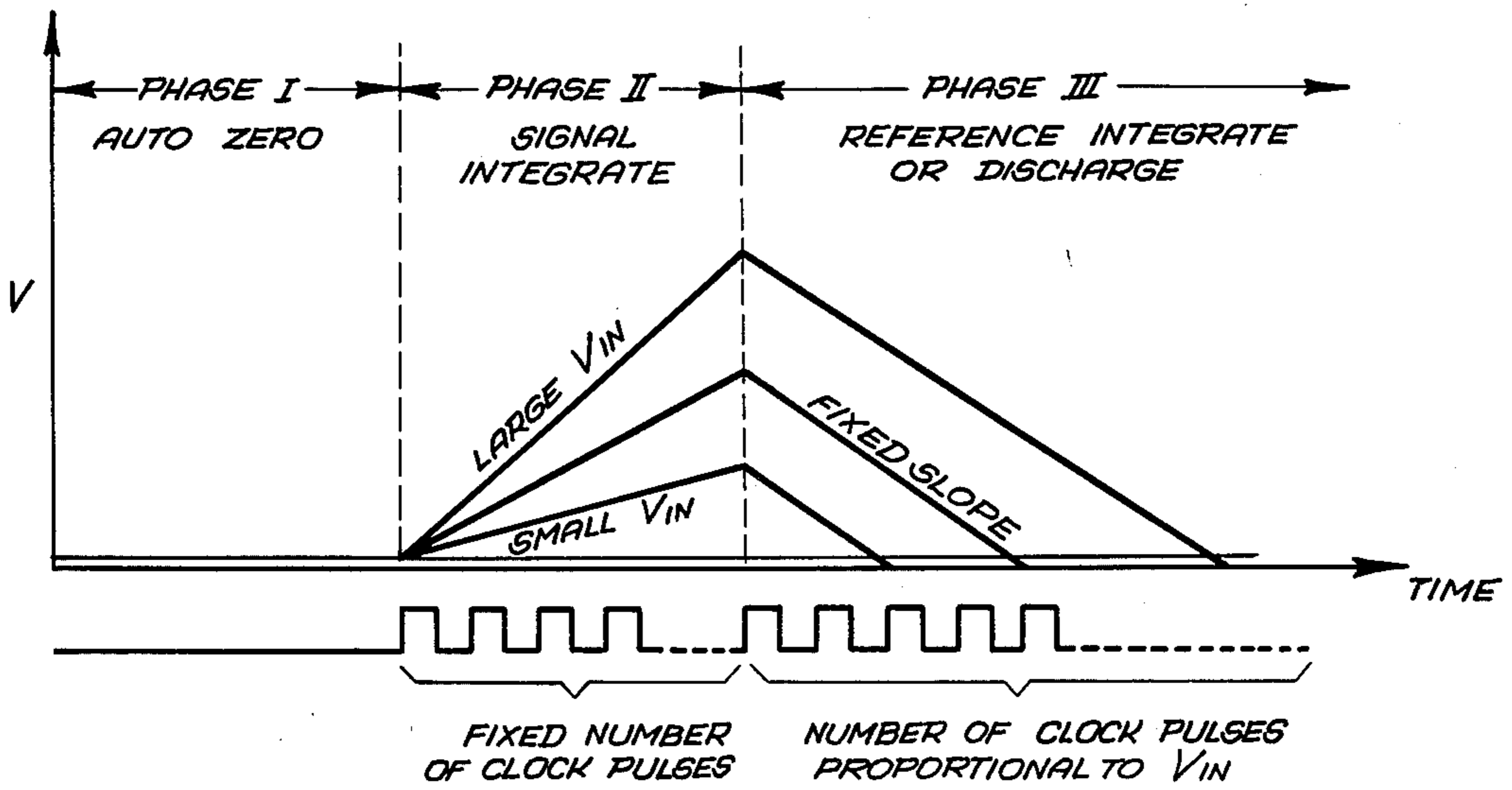
Fig. 2. PRIOR ART
