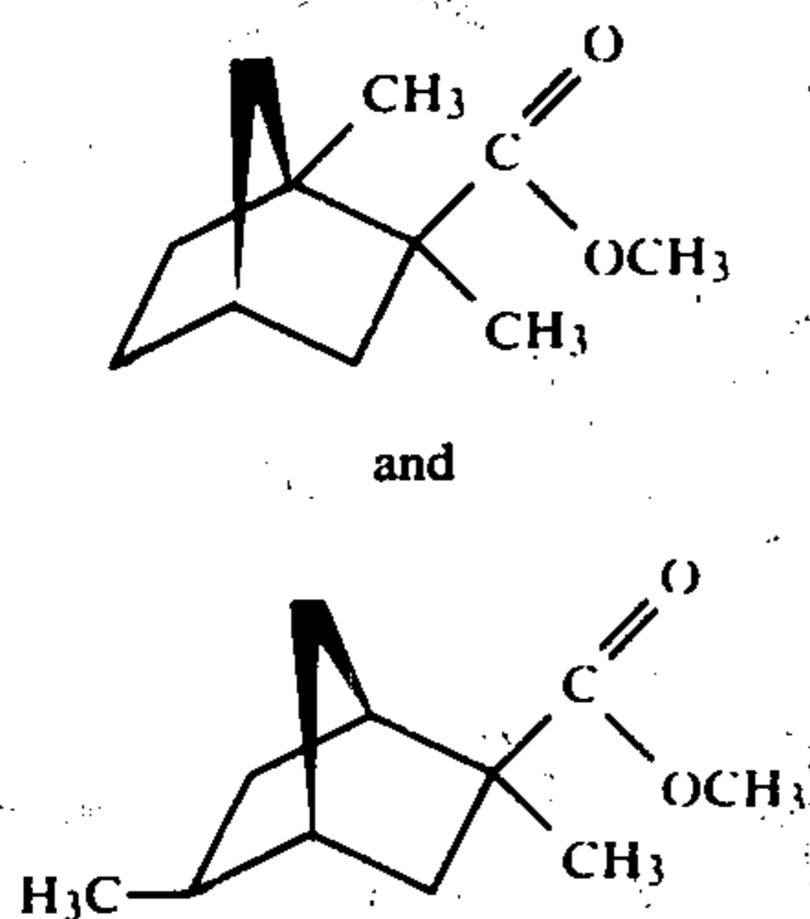
FIG. 4 is the infra-red spectrum for fraction 3 of the distillation product of the reaction product of Example II containing the compounds having the structures:
