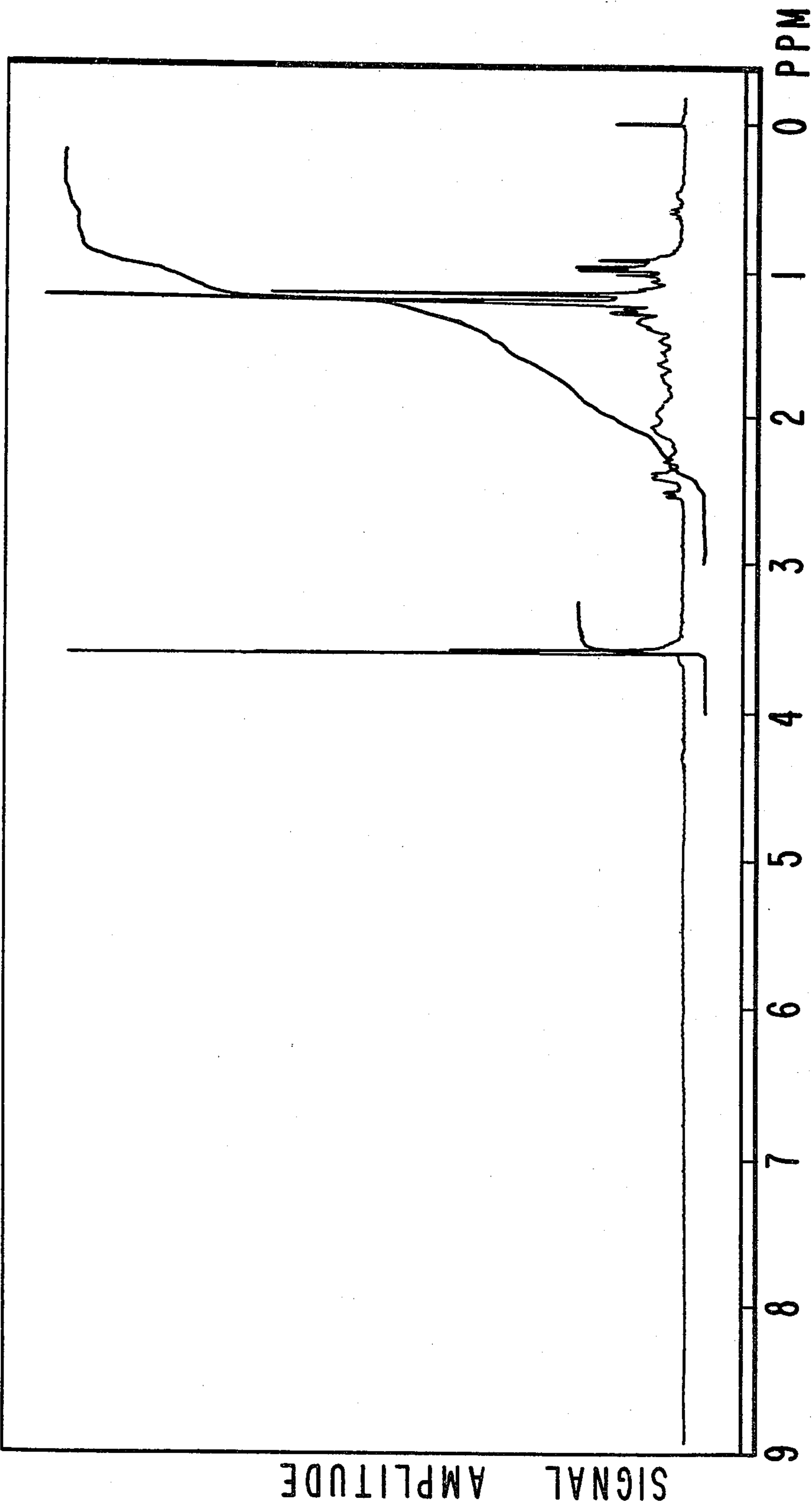
NMR SPECTRUM FOR FRACTION 3 OF EXAMPLE II.
