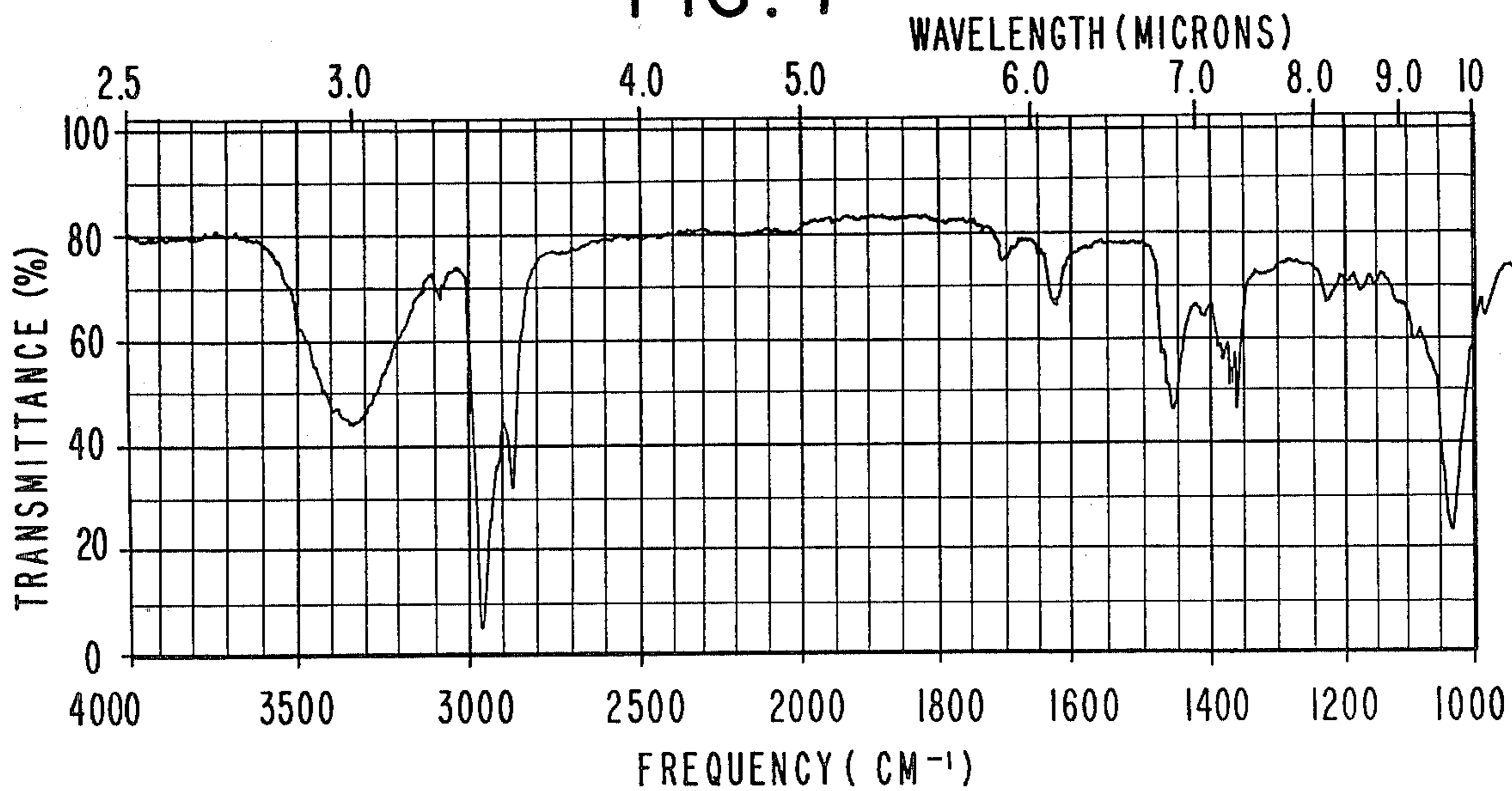
IR SPECTRUM FOR EXAMPLE II.
