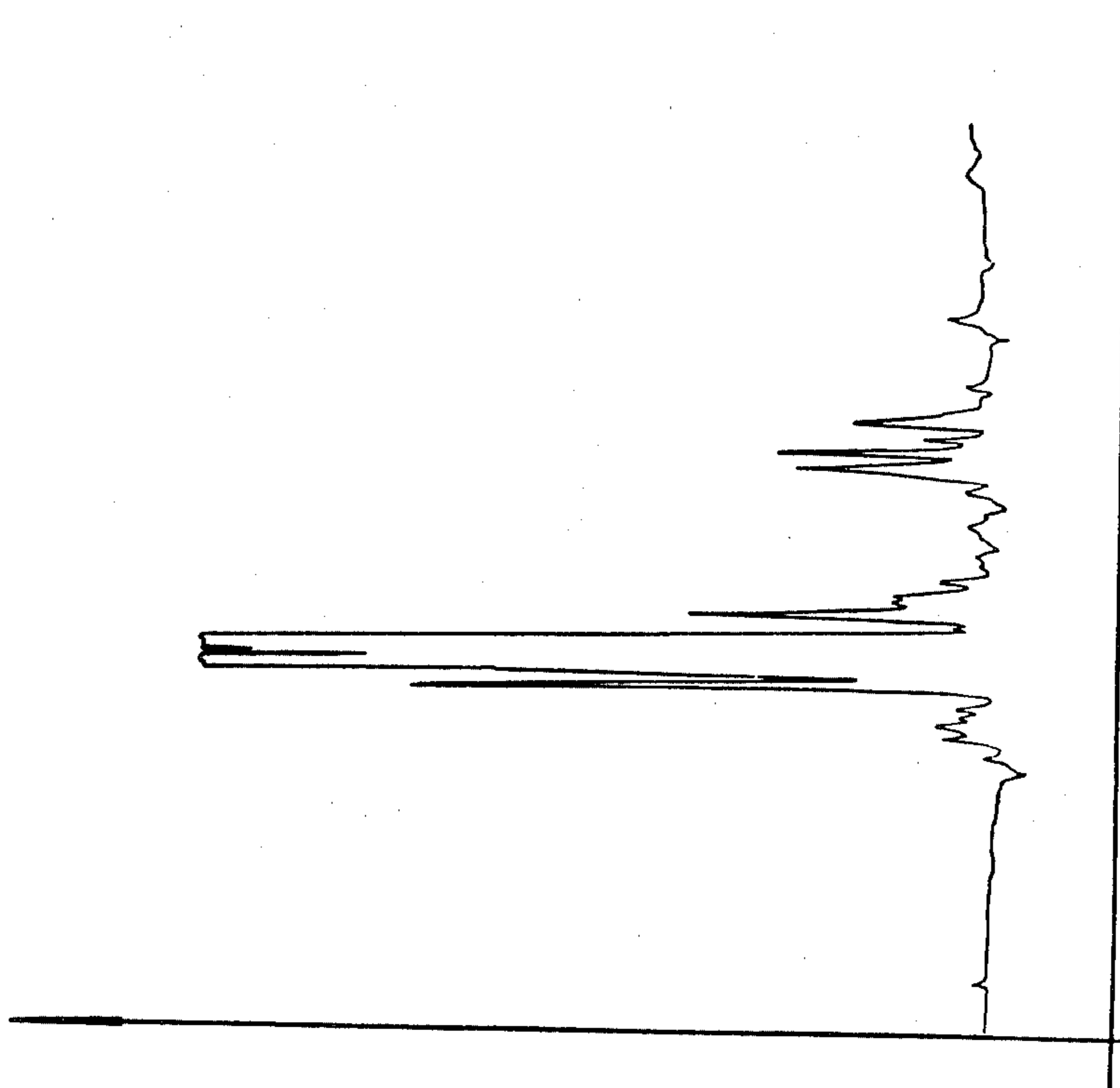
GLC PROFILE FOR EXAMPLE A CRUDE PRODUCT
