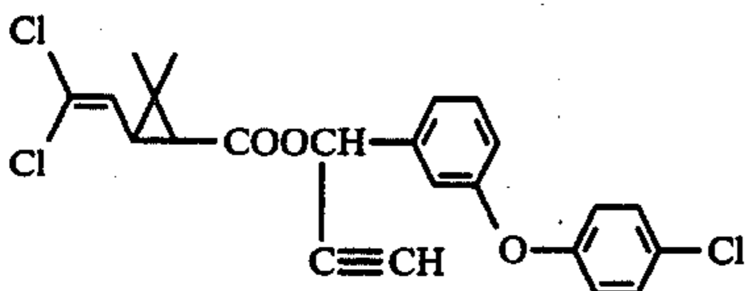
3-(4-Chloro- phenoxy)- \alpha - ethynylbenzyl 2,2-dimethyl-3- (2,2-dichloro- vinyl)cyclopro- panecarboxylate [hereinafter referred to as Compound (2)]
