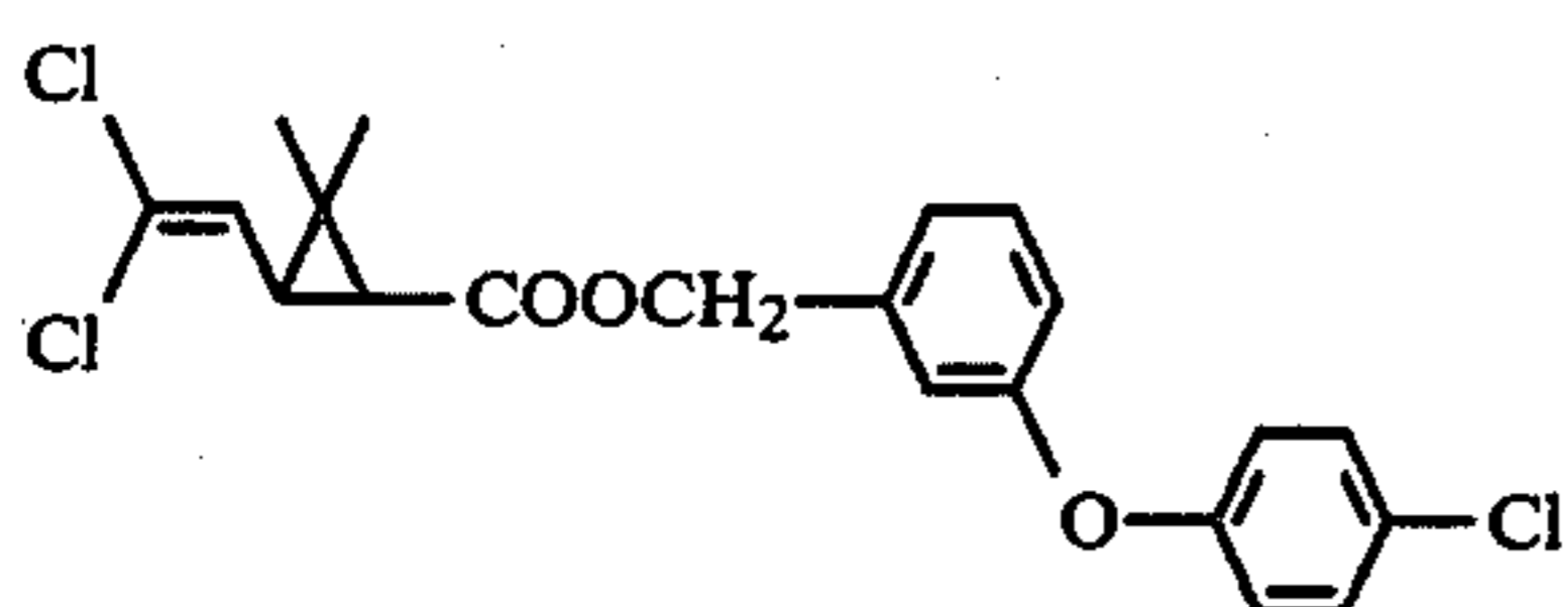
3-(4-Chloro- phenoxy)benzyl 2,2-dimethyl-3- (2,2-dichloro- vinyl)cyclopro- panecarboxylate [hereinafter referred to as Compound (1)]
