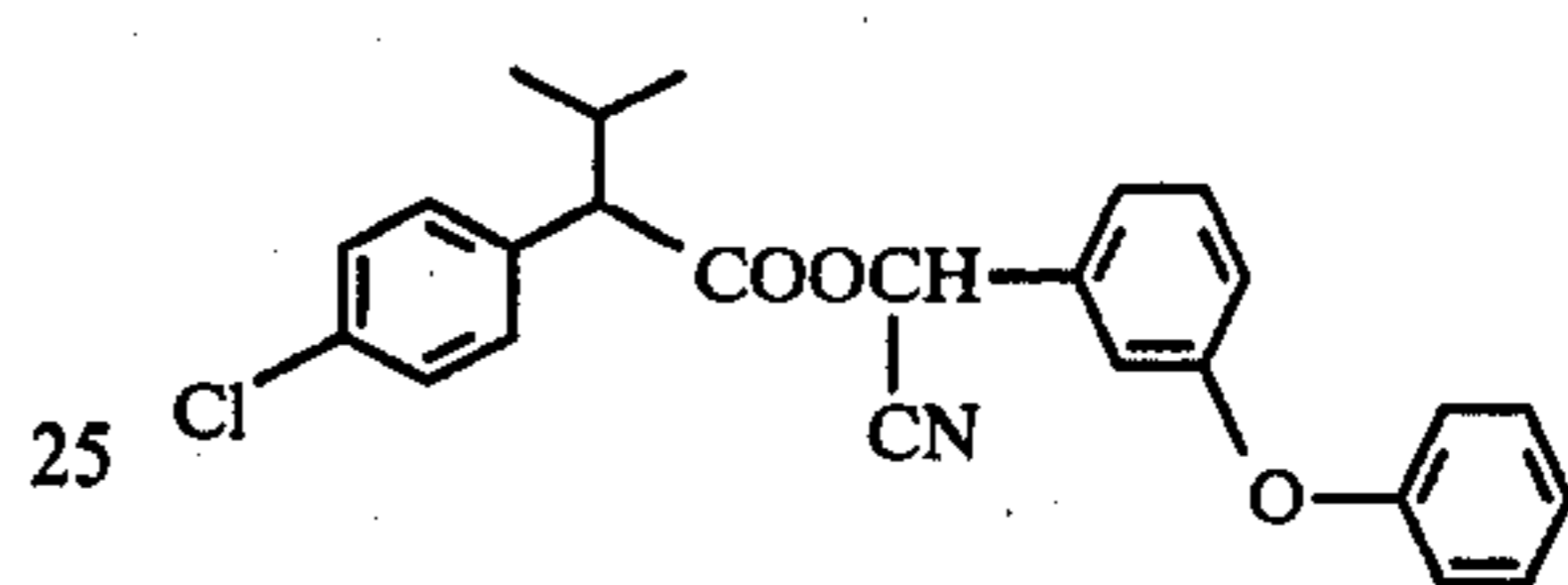
Fenvalerate [hereinafter referred to as Compound (E)]
