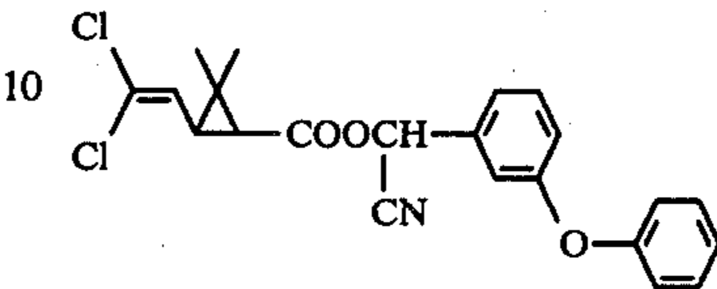
Cypermethrin [hereinafter referred to as Compound (C)]
