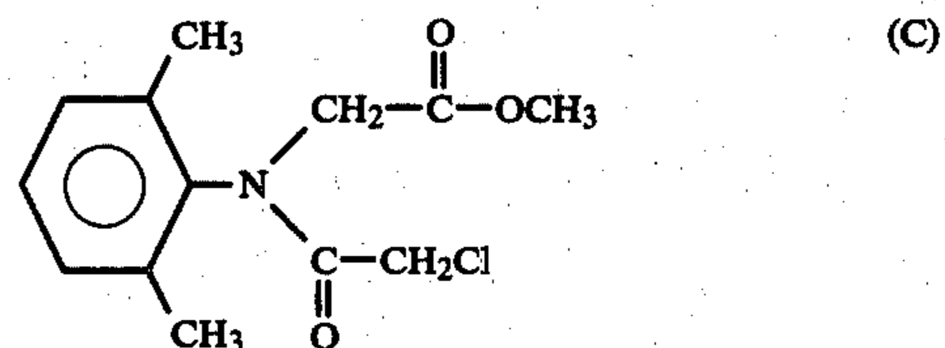
N-Chloroacetyl-N-(2,6-xyllyl)-glycine methyl ester
