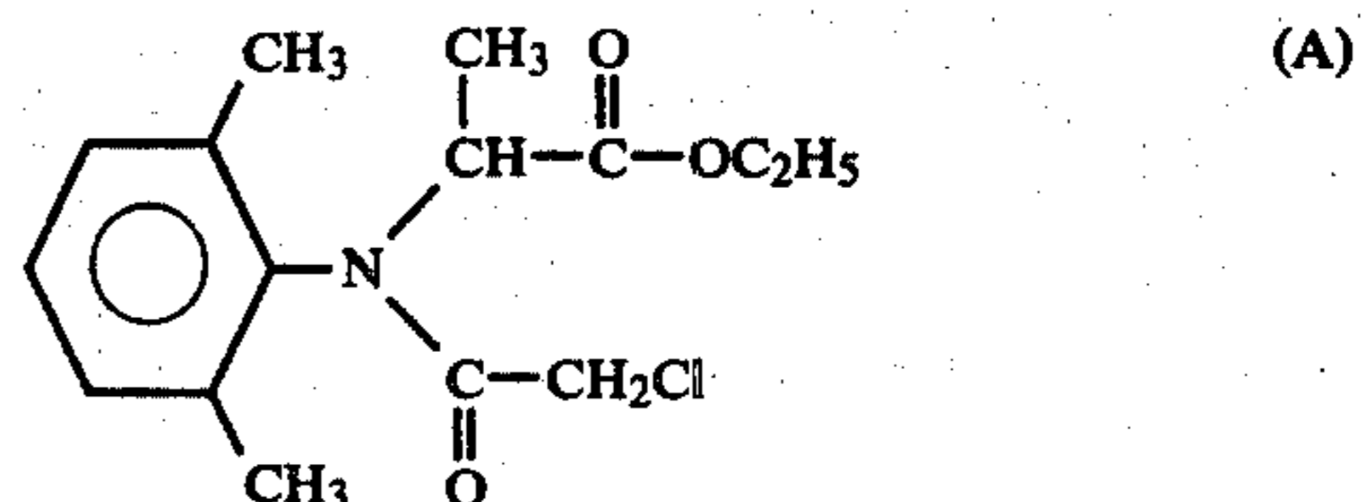
N-Chloroacetyl-N-(2,6-xyllyl)-alanine ethyl ester
