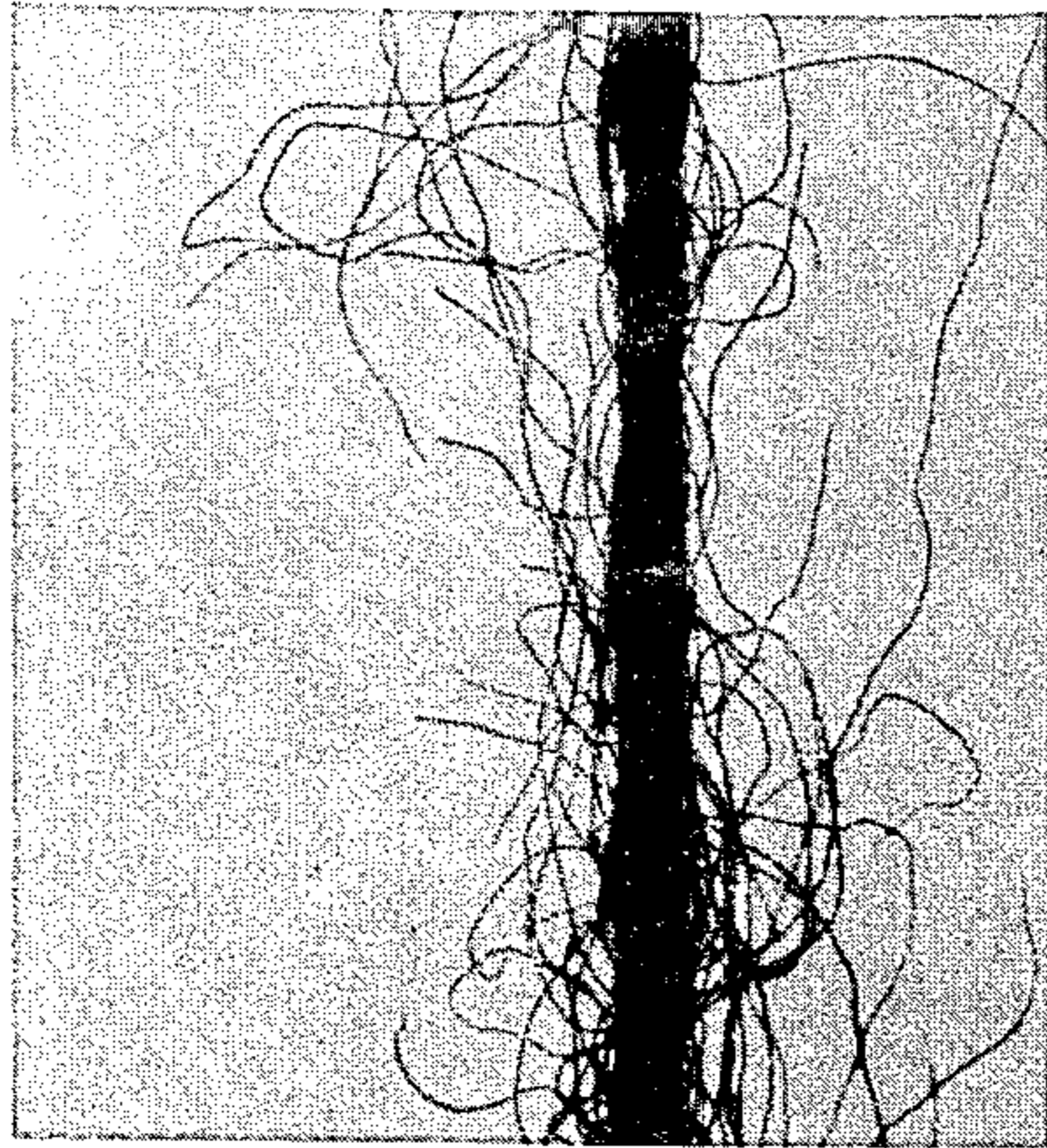
FIGURE 5 100% polyester yarn mixed fiber length 19.4% 1\frac{1}{2} inches (by wt) 41.7% 1\frac{1}{4} inches 20.4% 1 inch 12.5% \frac{3}{4} inch 4.6% \frac{1}{2} inch 1.4% \frac{1}{4} inch
