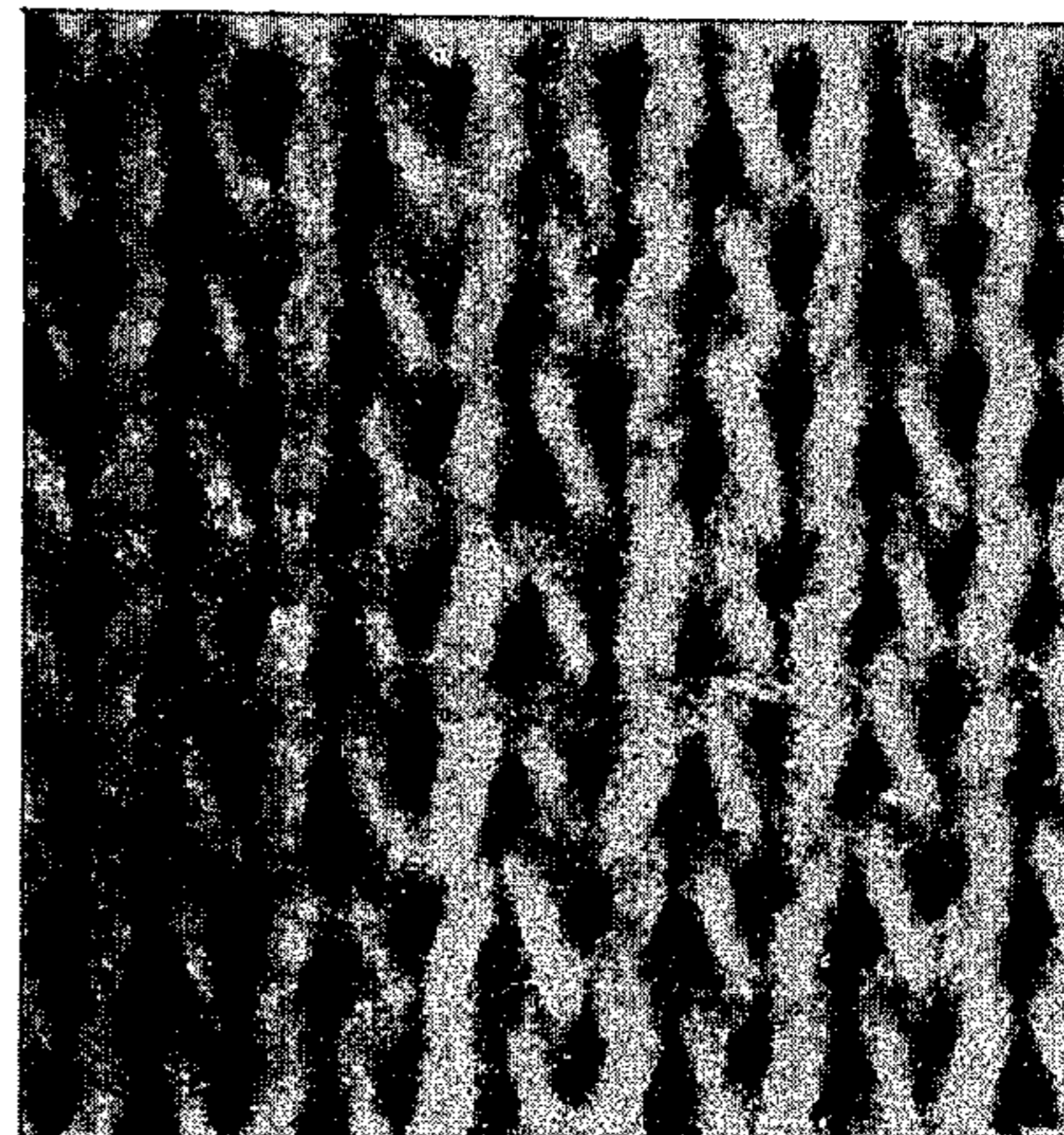
FIGURE 6 100% polyester yarn mixed fiber length 20% 1\frac{1}{4} inches (by wt) 40% 1 inch 25% \frac{3}{4} inch 15% \frac{1}{2} inch
