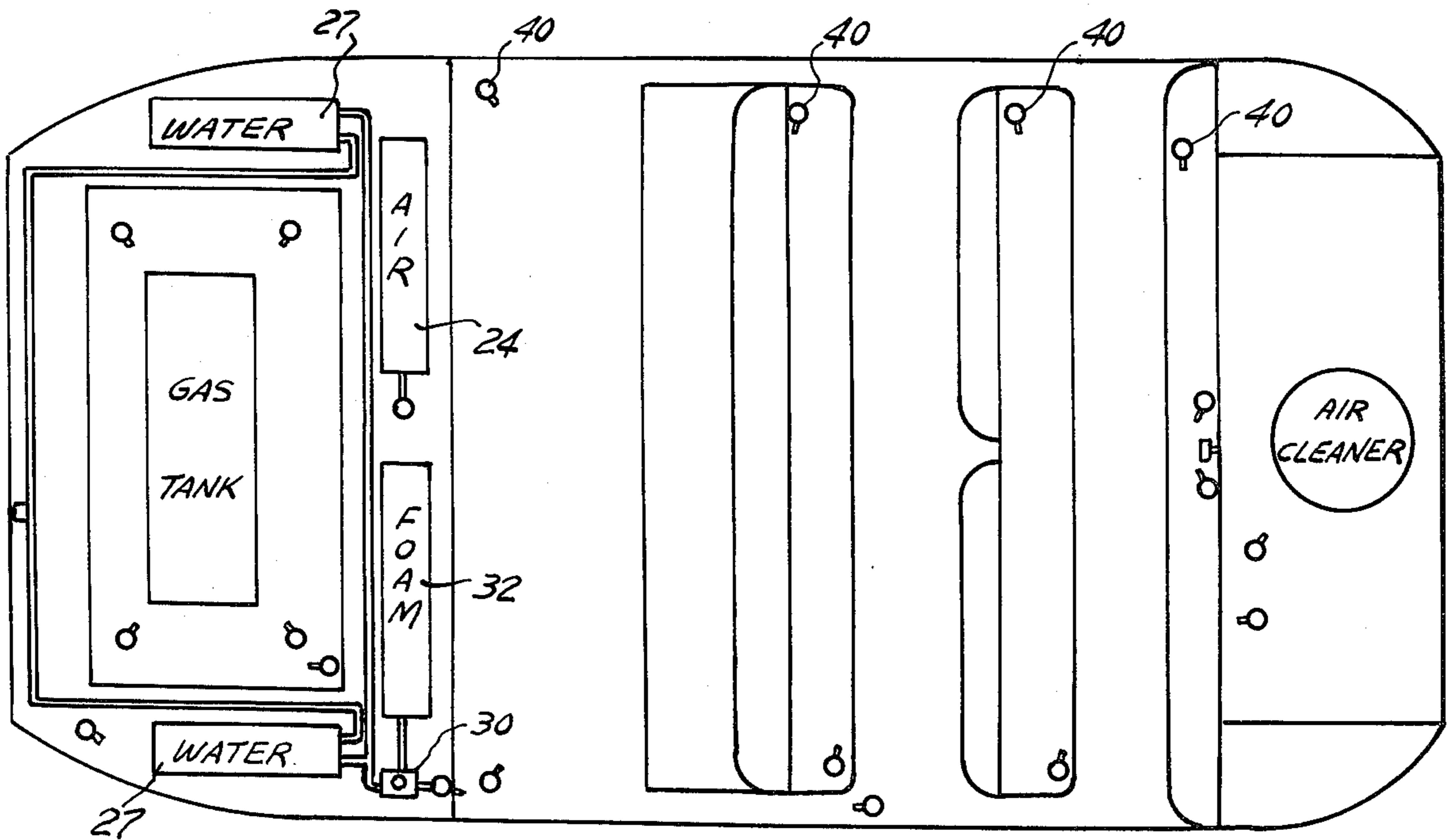
WATER REFILL & TANKS & LINES
