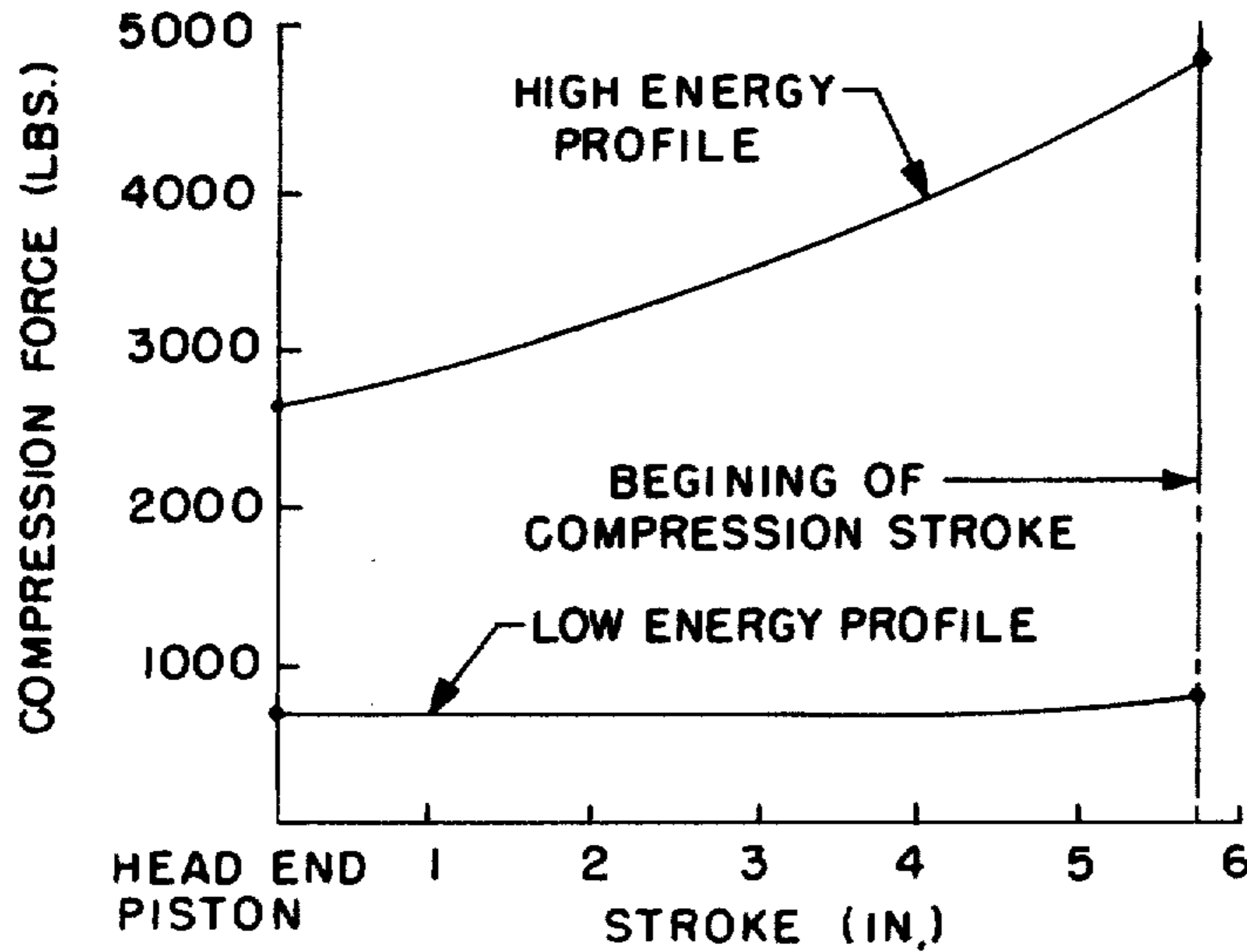
COMPRESSION FORCE VS. PISTON STROKE
